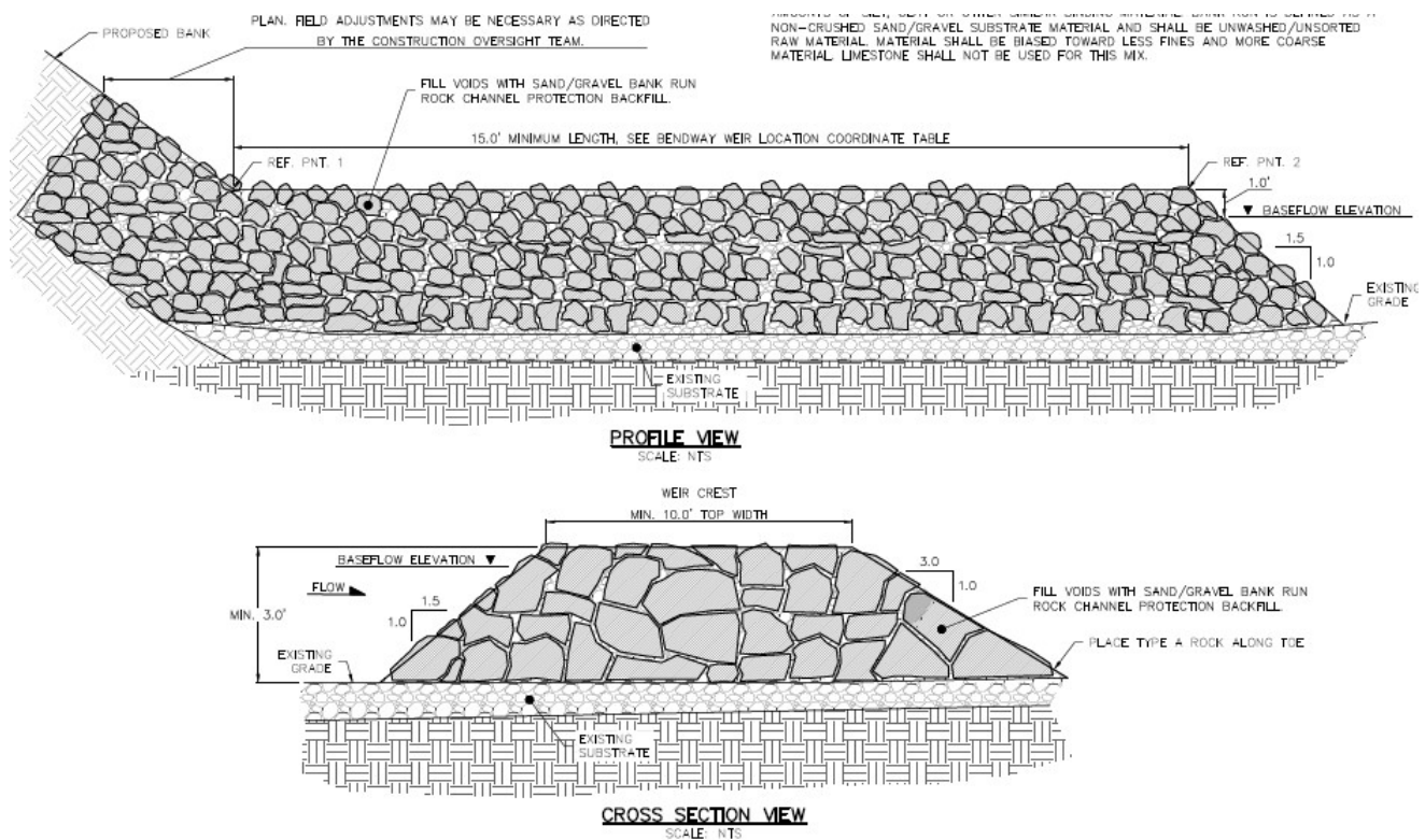
Figure 5. Bendway Structure Details. The structure is 3 feet high, 20 feet wide, and will extend more than 15 feet out into the river.
