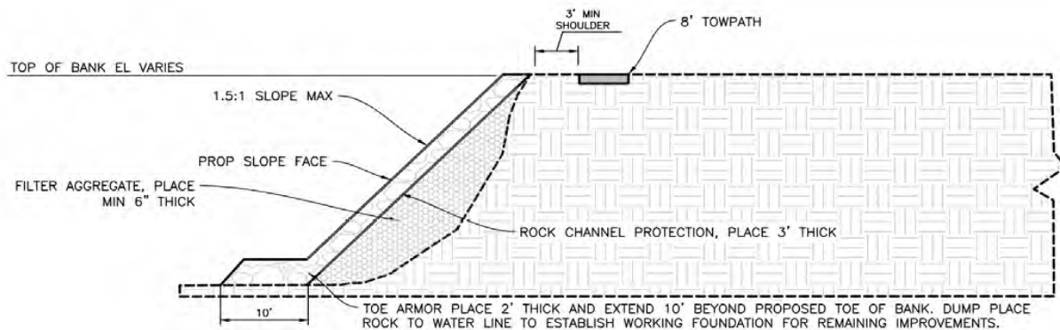
Figure 6: Durable Riprap Alternative
