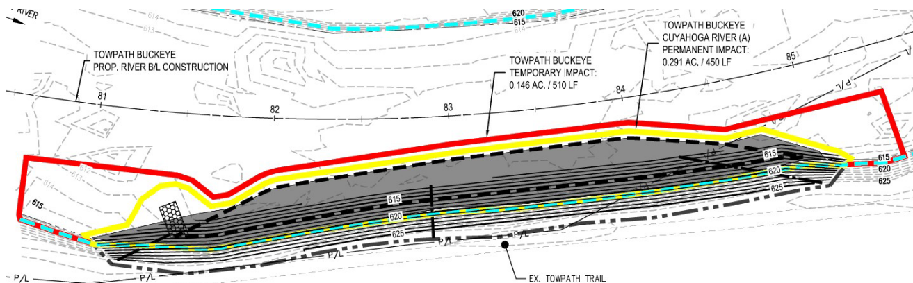
Figure 4. Buckeye Towpath project showing limits of disturbance (inside the red and yellow polygons) of permanent and temporary impacts (total 0.44 acre) to the riverine wetland.
