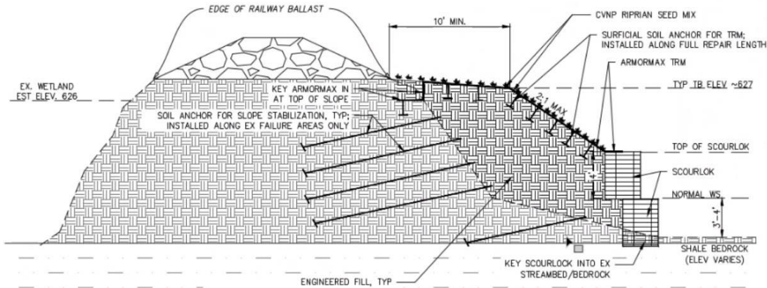
Figure 7: Armormax and Scourlok
