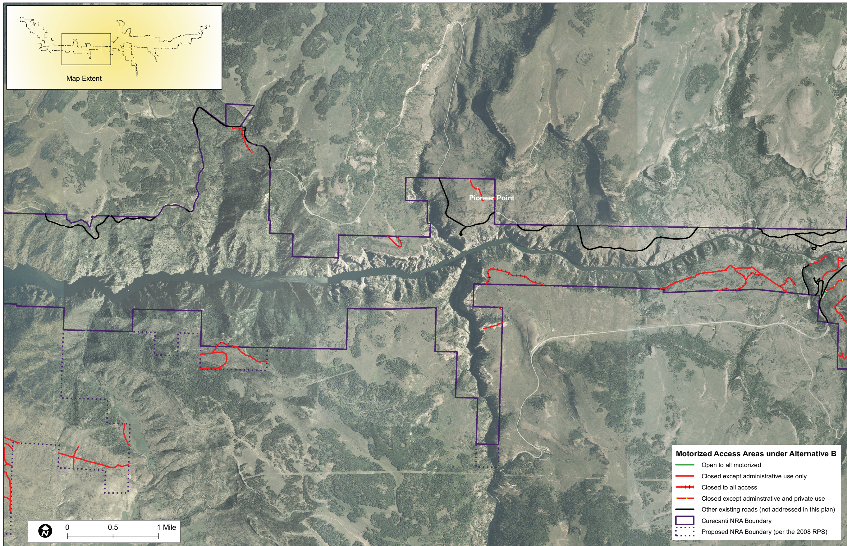
MAP 9. Alternative B: Designate Motorized Vehicle Access Consistent with the 1997 General Management Plan
