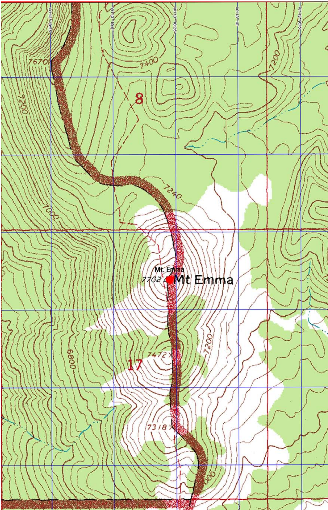
Mt. Emma Radio Site (Mt Logan 7.5 minute Quad Map)
