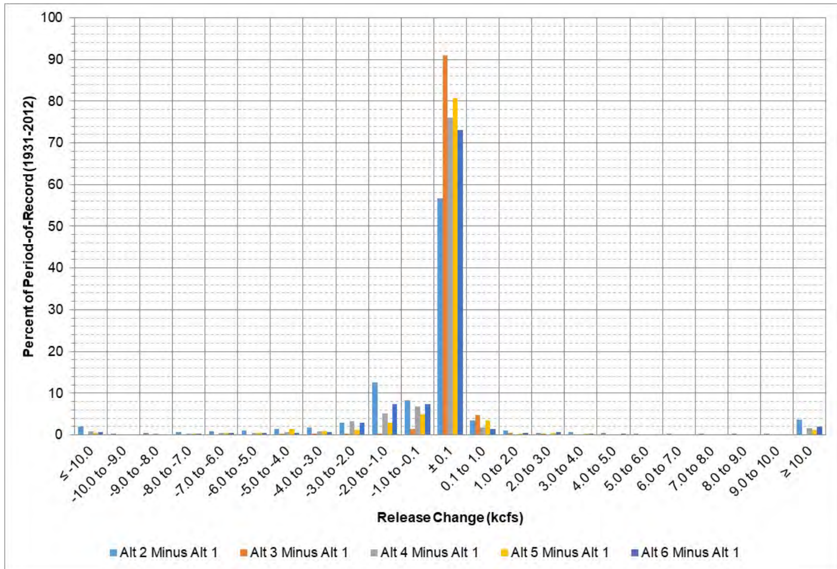
Figure 9-60: Gavins Point release change between each alternative and Alt 1 for all days in the period-of-record.
