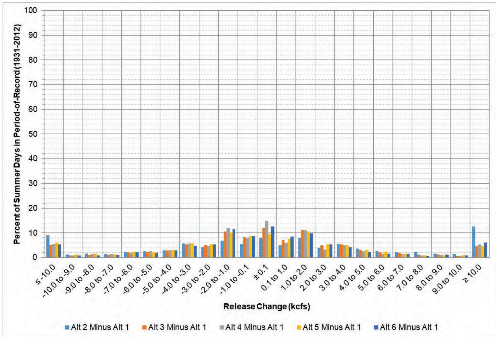
Figure 3-19: Oahe release change between each alternative and Alt 1 during May – August.
