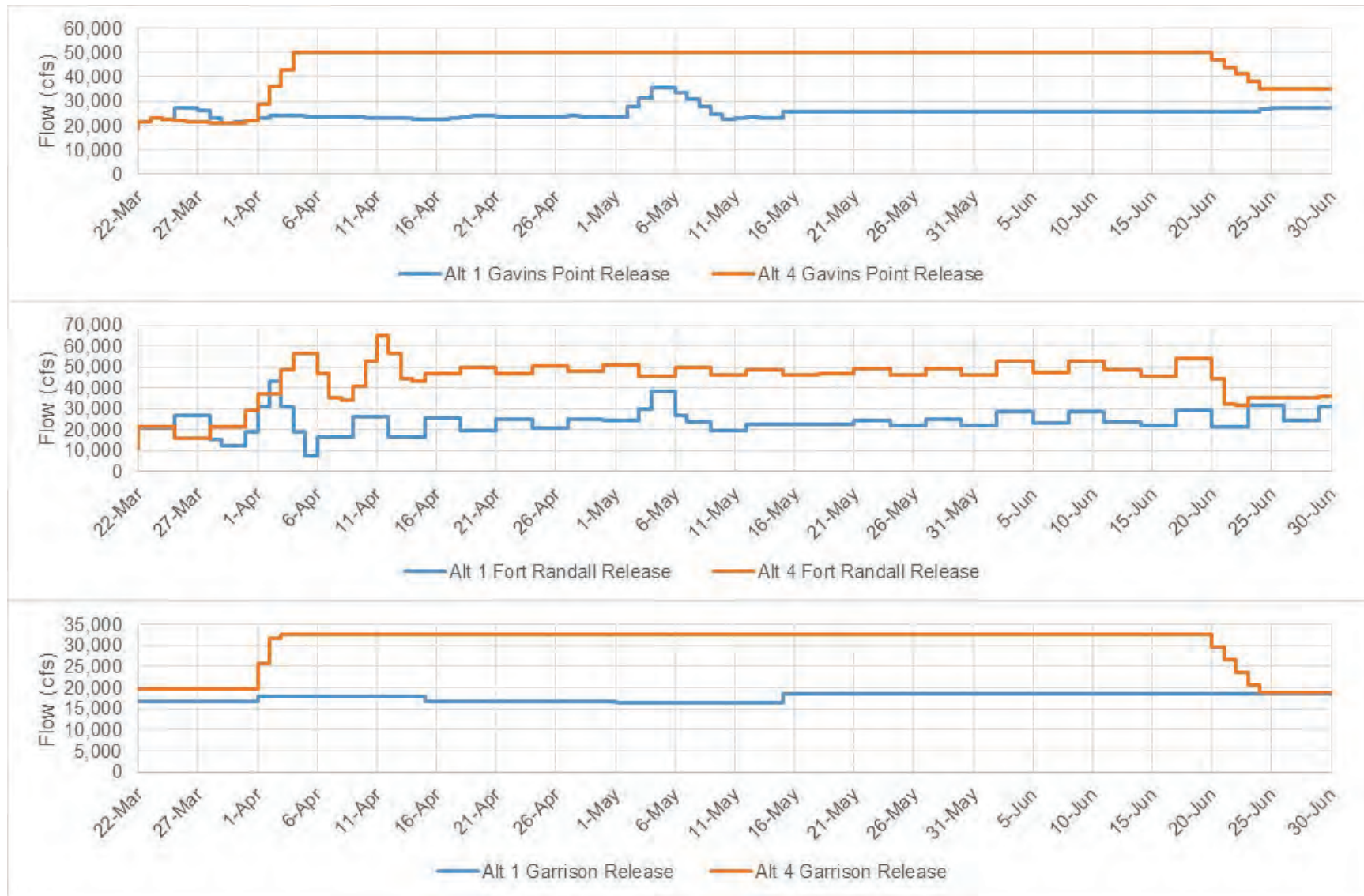
Figure 3-13: Comparison of Alt 1 vs Alt 4 Gavins Point, Fort Randall, and Garrison's releases during the ESH-creating release that extends into June.
