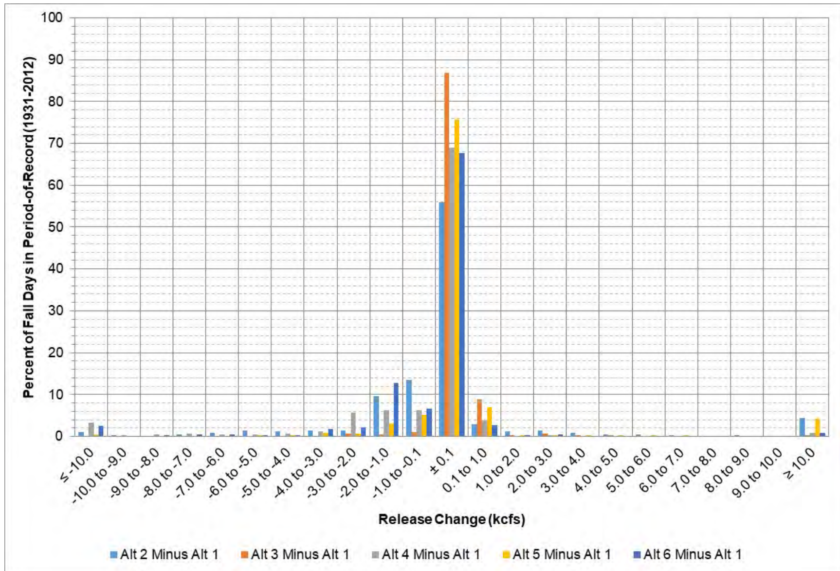
Figure 9-36: Gavins Point release change between each alternative and Alt 1 during September – November.
