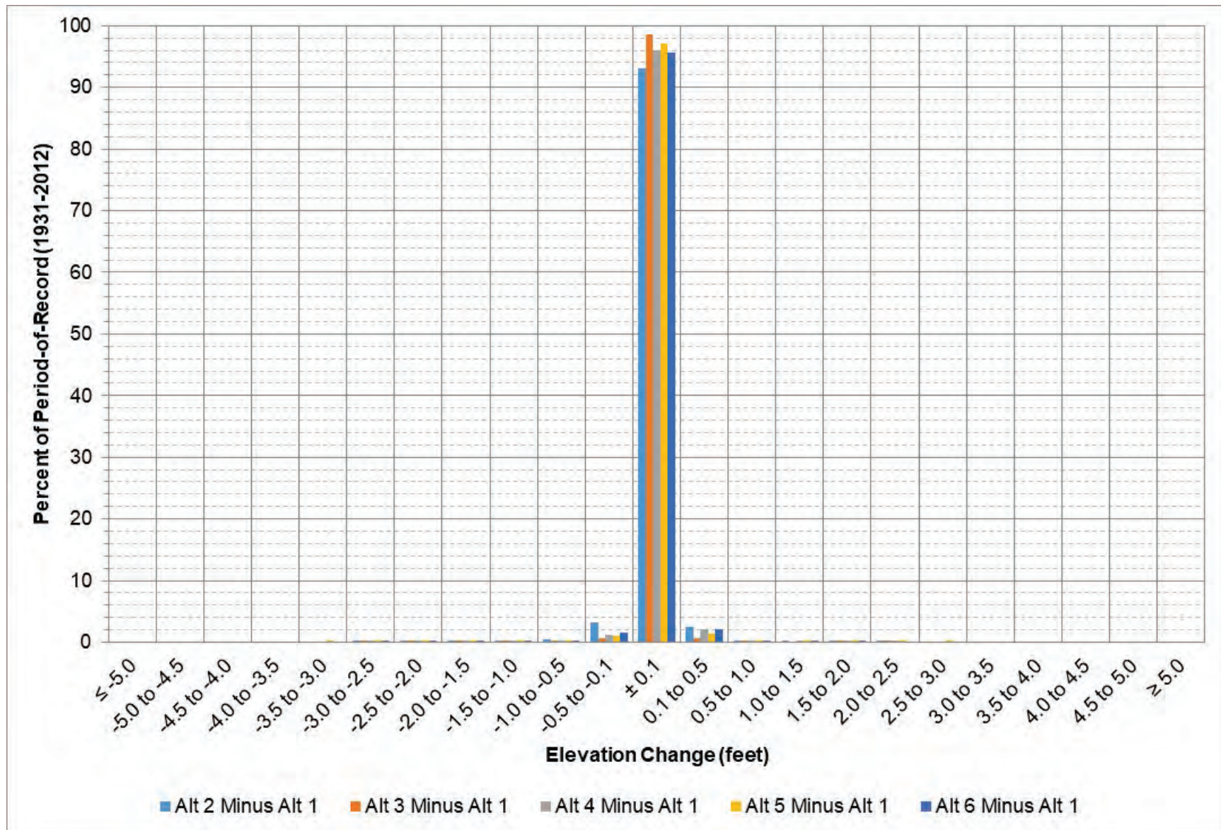
Figure 6-7: Big Bend elevation change between each alternative and Alt 1 for all days in the period-of-record.
