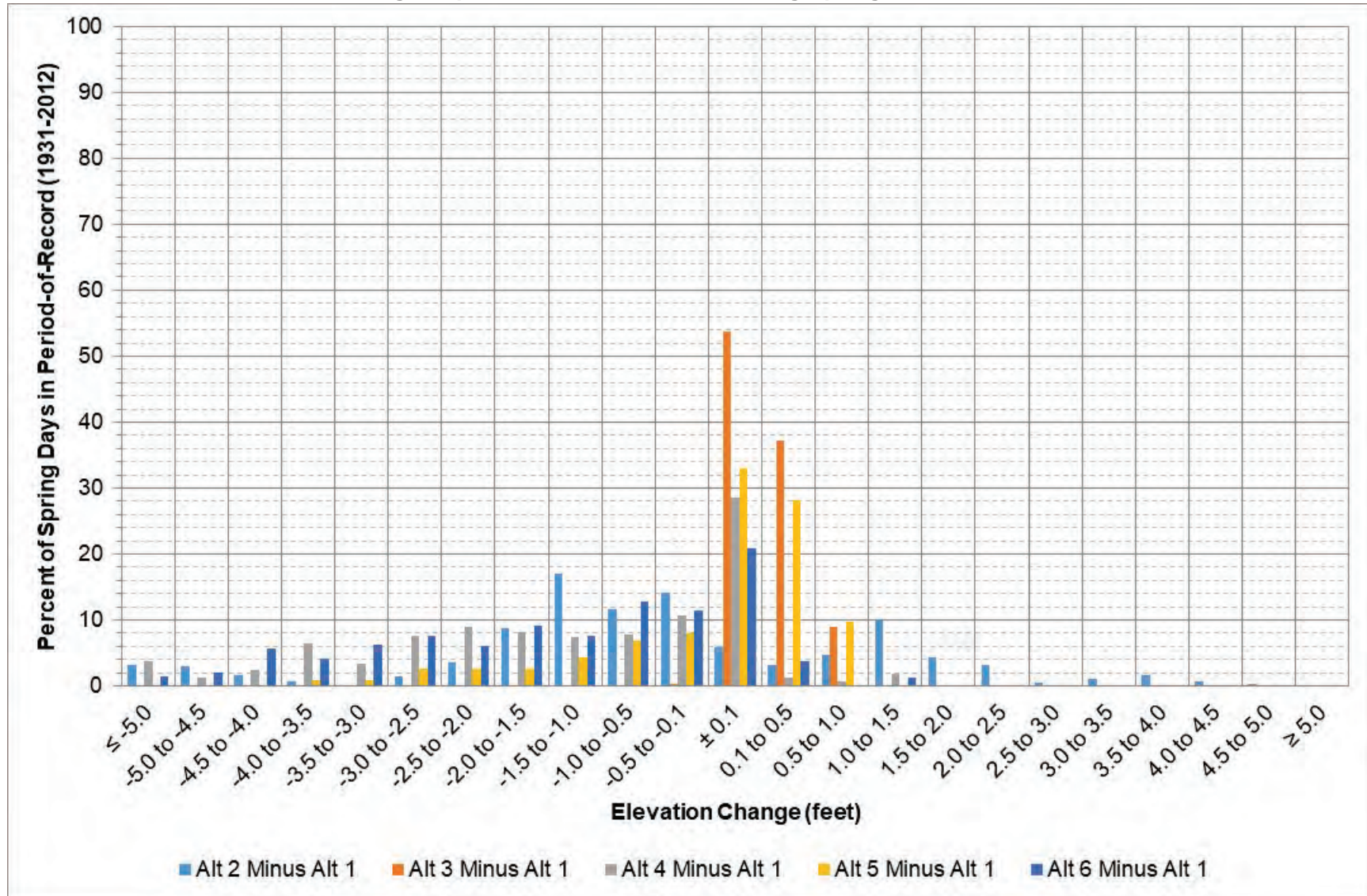
Figure 2-17: Fort Peck elevation change between each alternative and Alt 1 during March – April.
