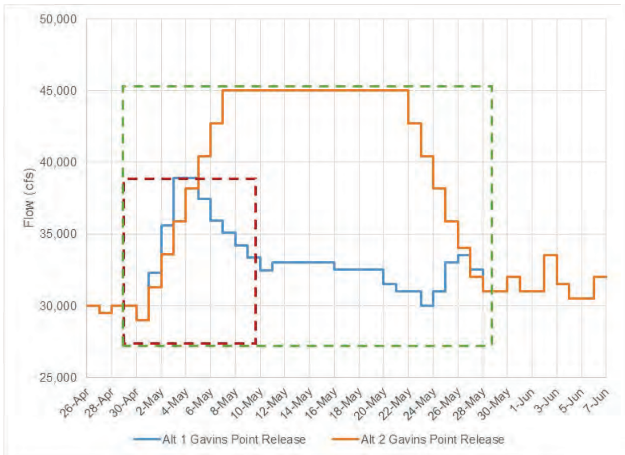
Figure 3-5: Alt 1 vs Alt 2 early spring spawning cue.
