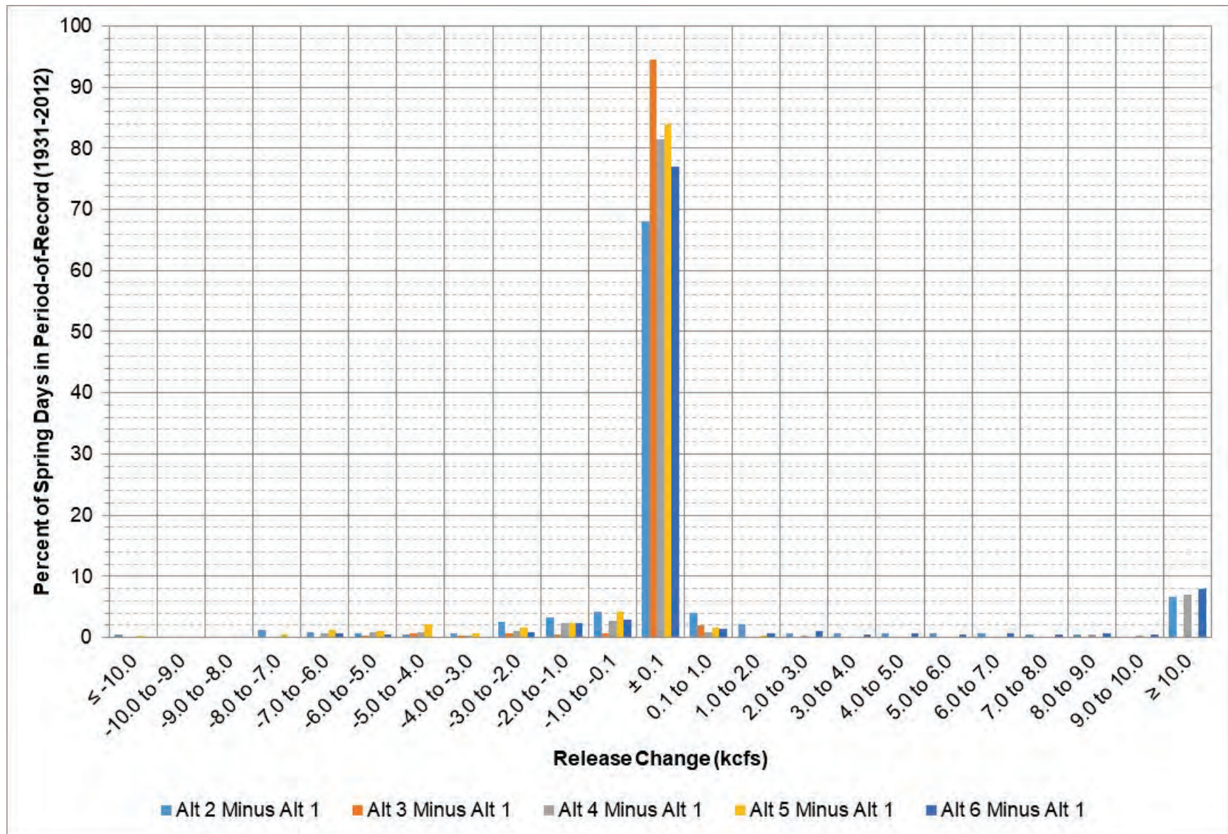
Figure 2-12: Gavins Point release change between each alternative and Alt 1 during March – April.
