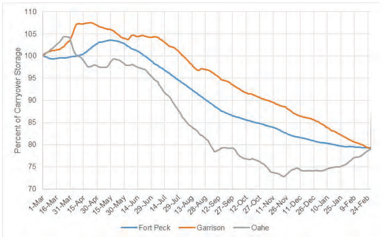
Figure 2-13: Storage balancing at Fort Peck, Garrison, and Oahe.
