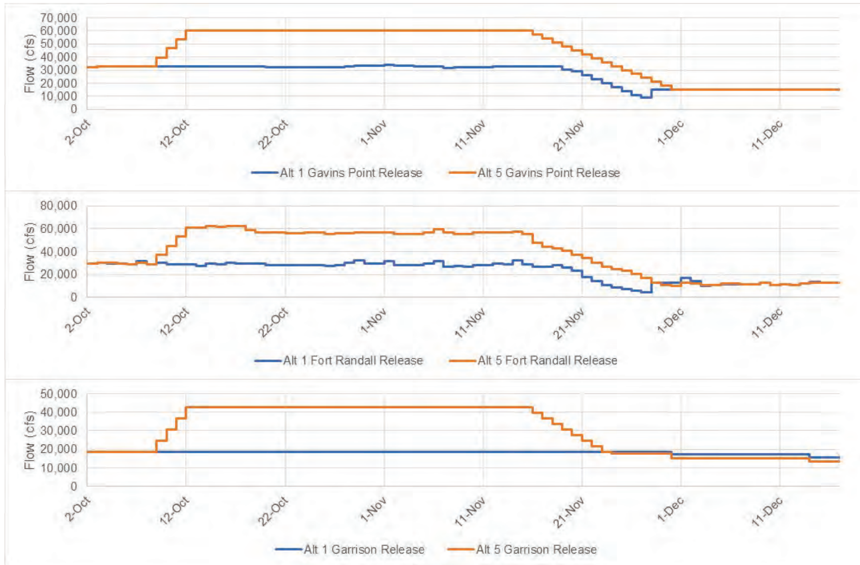
Figure 4-9: Comparison of Alt 1 vs Alt 5 Gavins Point, Fort Randall, and Garrison's releases during the ESH-creating release shown in Figure 4-8.
