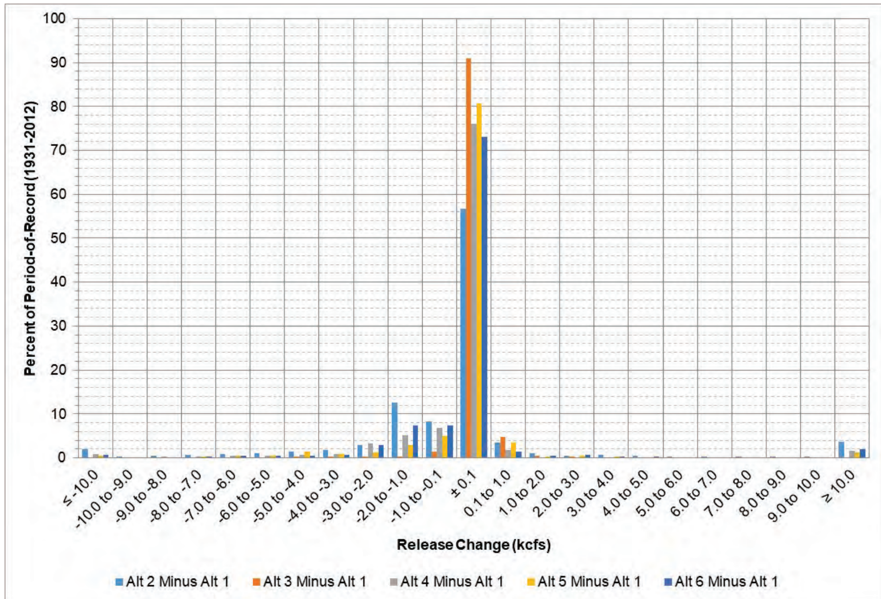
Figure 6-12: Gavins Point release change between each alternative and Alt 1 for all days in the period-of-record.
