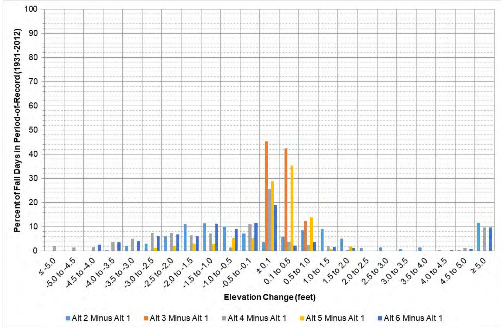
Figure 9-25: Fort Peck elevation change between each alternative and Alt 1 during September – November.
