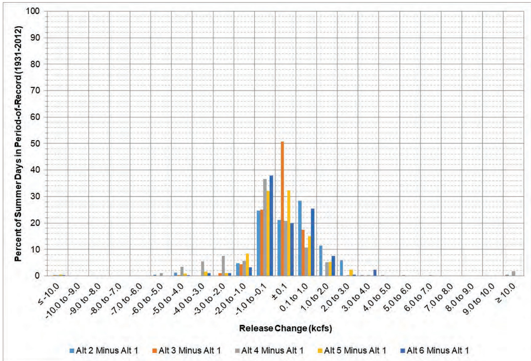
Figure 3-17: Garrison release change between each alternative and Alt 1 during May – August.
