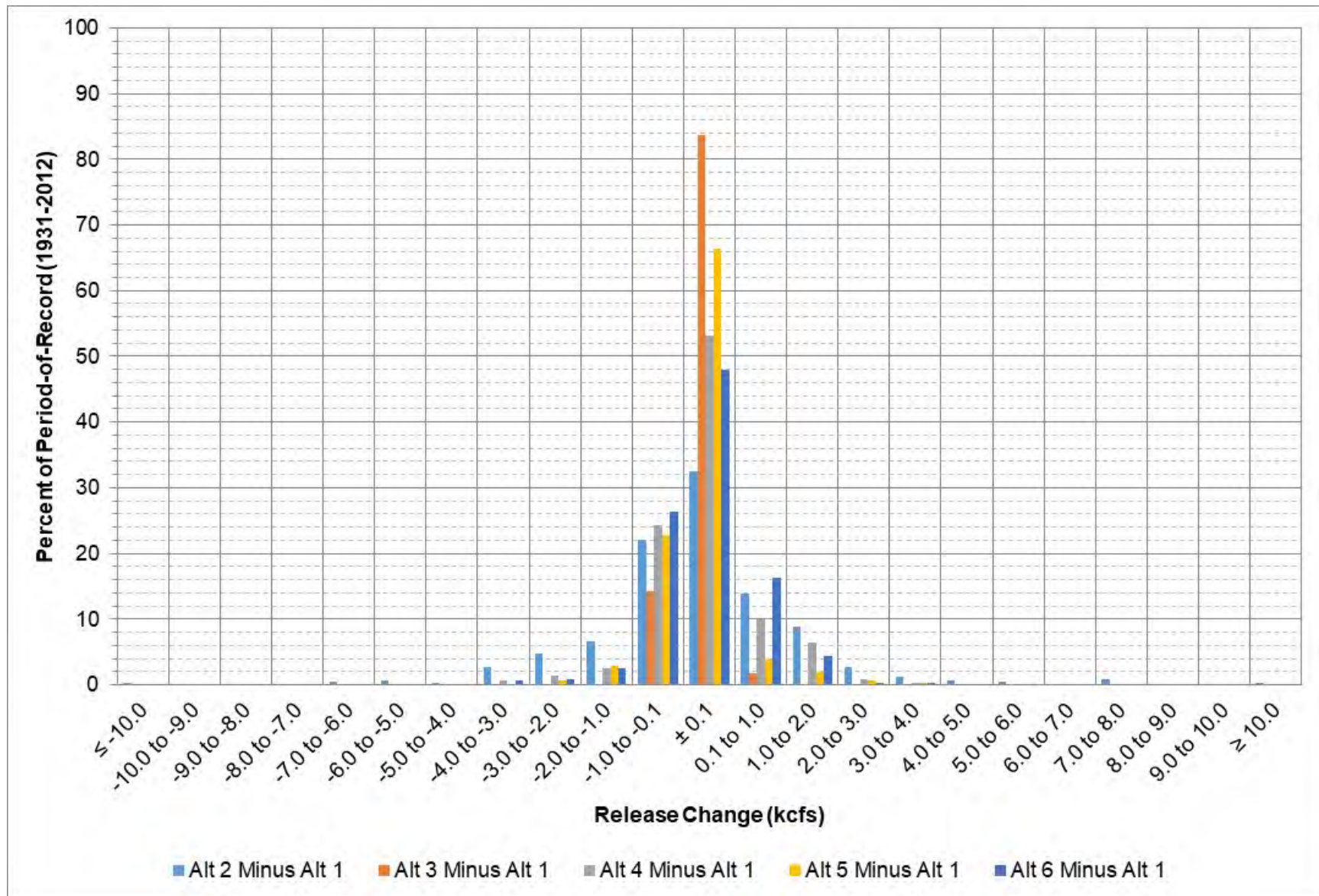
Figure 9-50: Fort Peck release change between each alternative and Alt 1 for all days in the period-of-record.
