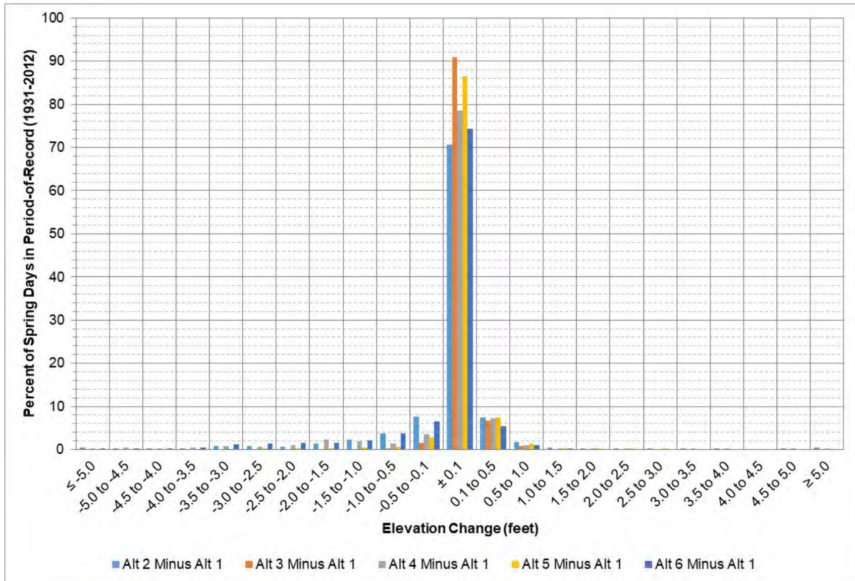
Figure 9-9: Fort Randall elevation change between each alternative and Alt 1 during March – April.
