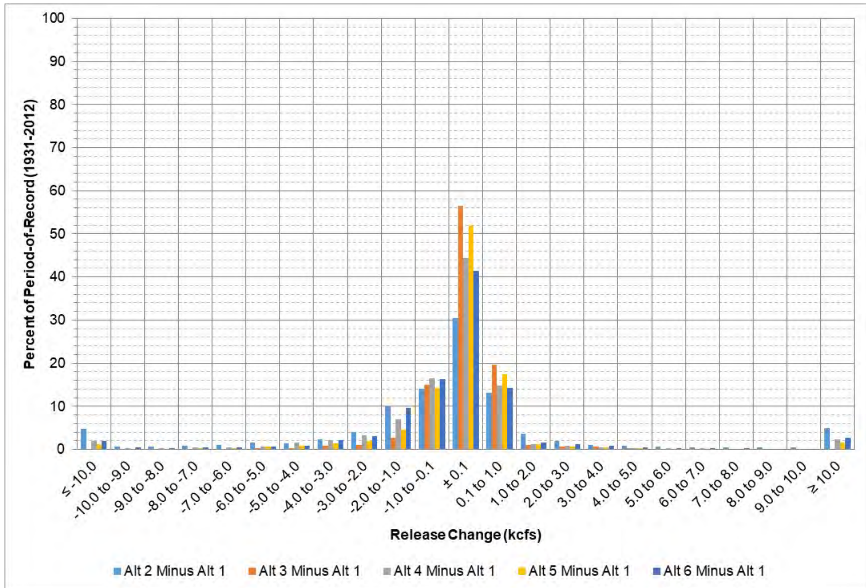
Figure 9-54: Oahe release change between each alternative and Alt 1 for all days in the period-of-record.
