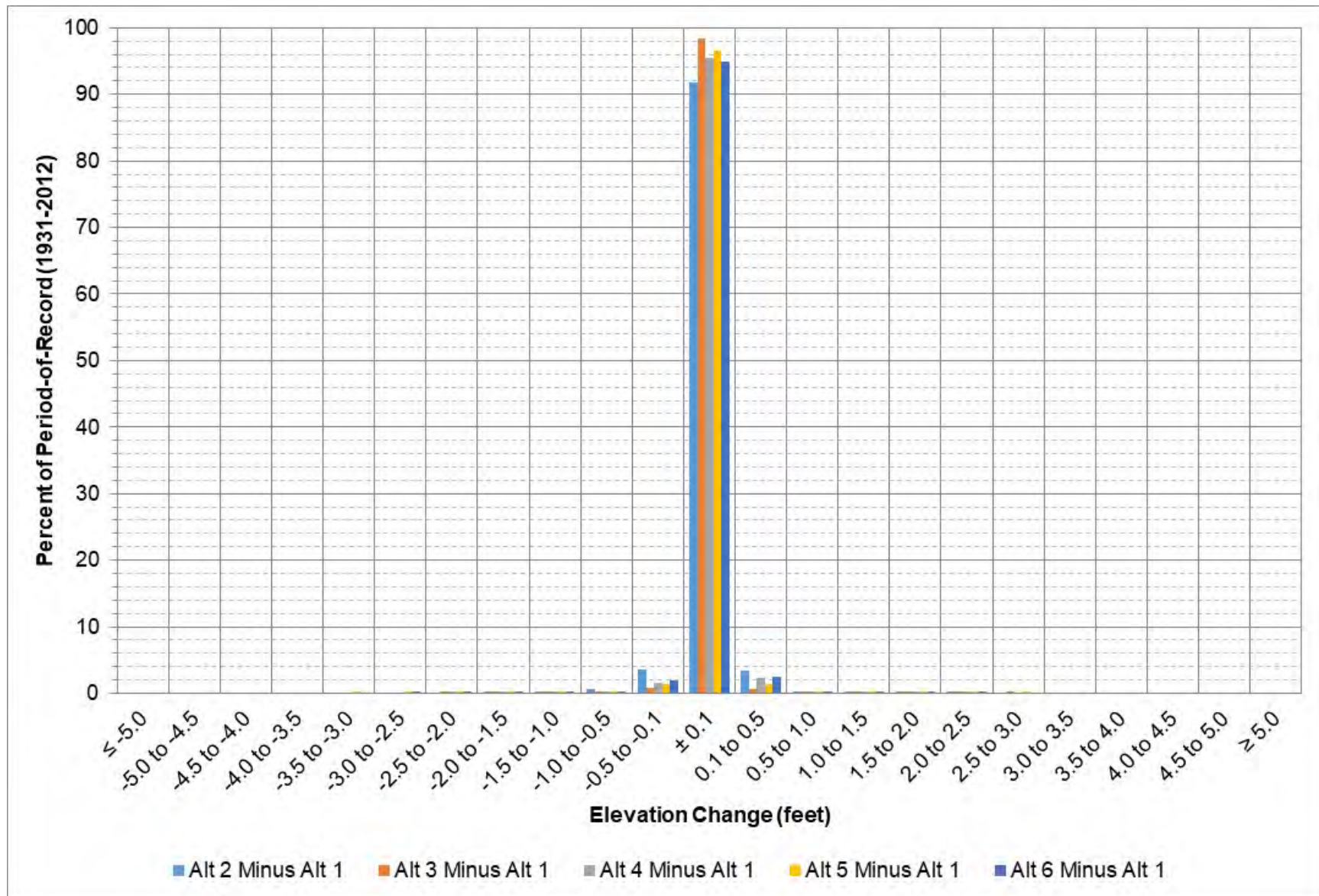
Figure 9-55: Big Bend elevation change between each alternative and Alt 1 for all days in the period-of-record.
