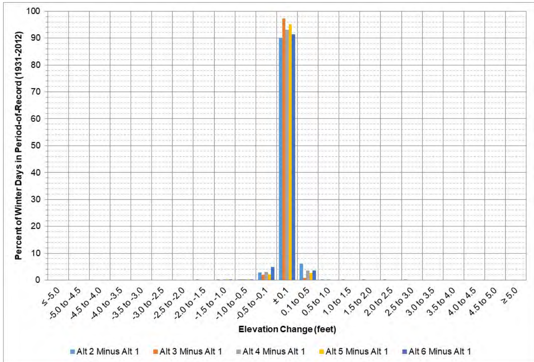
Figure 9-47: Gavins Point elevation change between each alternative and Alt 1 during December – February.
