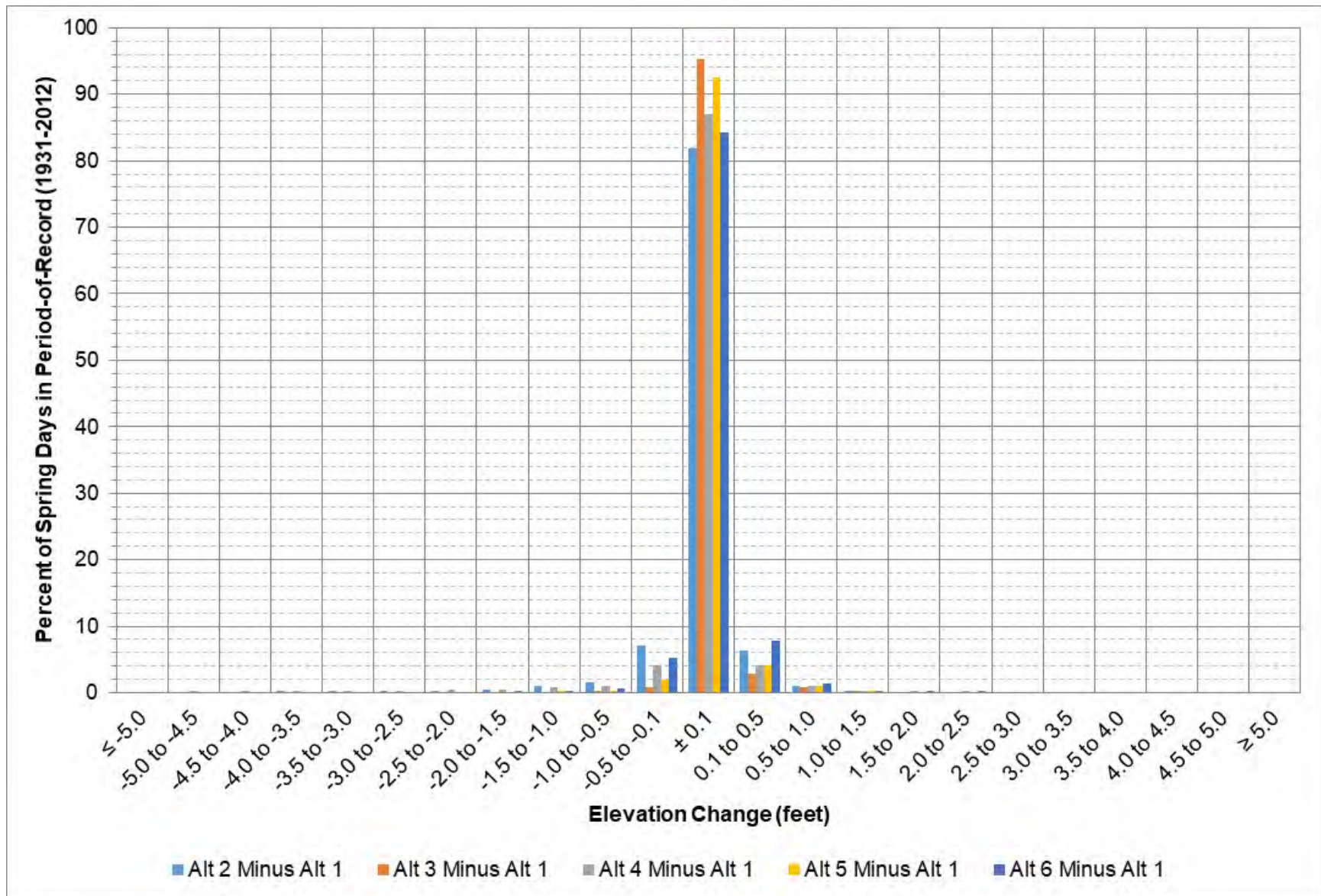
Figure 9-11: Gavins Point elevation change between each alternative and Alt 1 during March – April.
