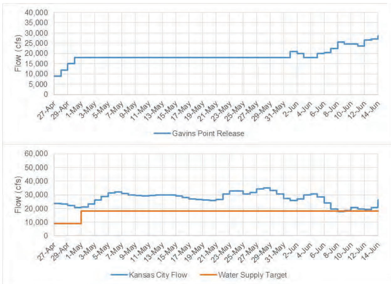
Figure 3-4: Summer water supply operations.
