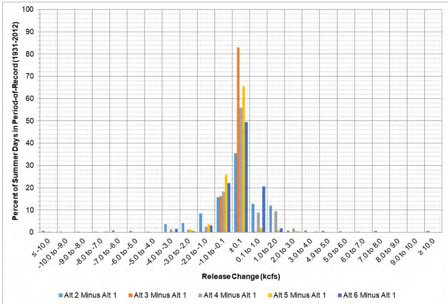
Figure 9-14: Fort Peck release change between each alternative and Alt 1 during May – August.
