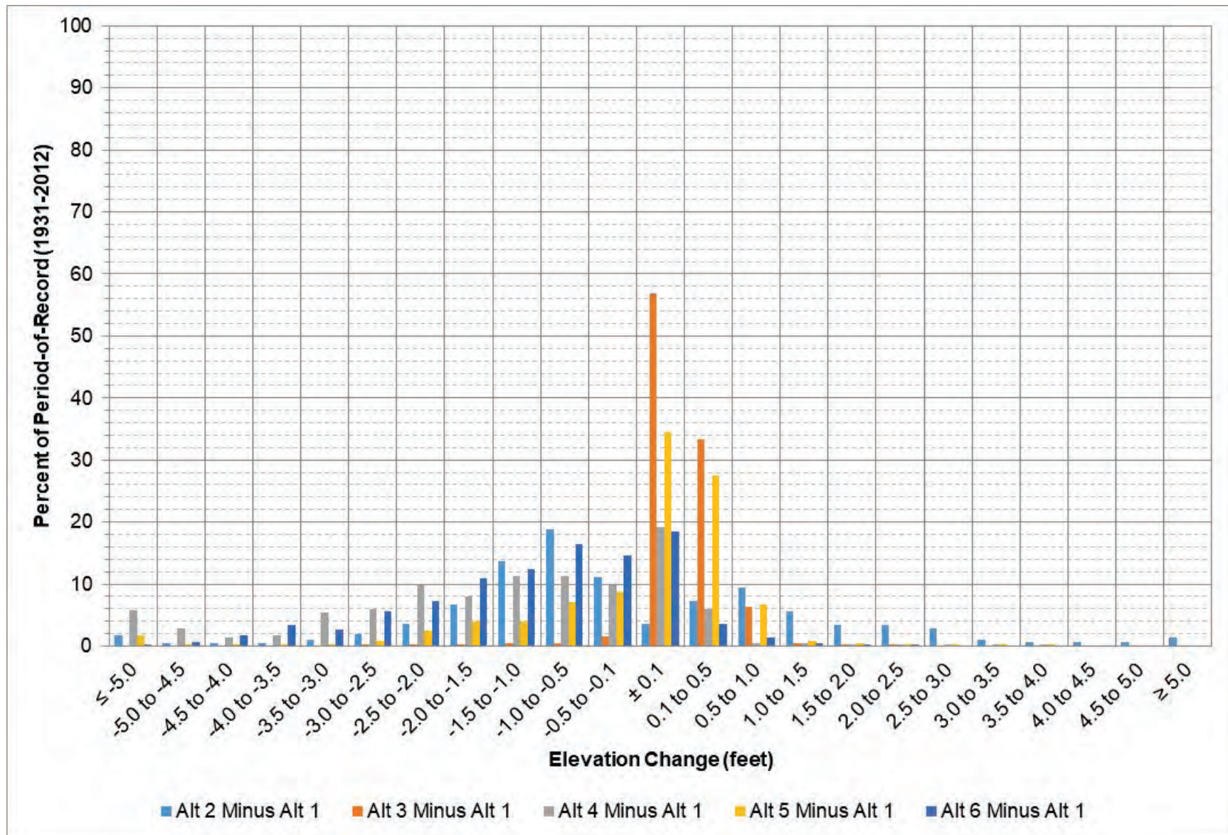
Figure 6-3: Garrison elevation change between each alternative and Alt 1 for all days in the period-of-record.
