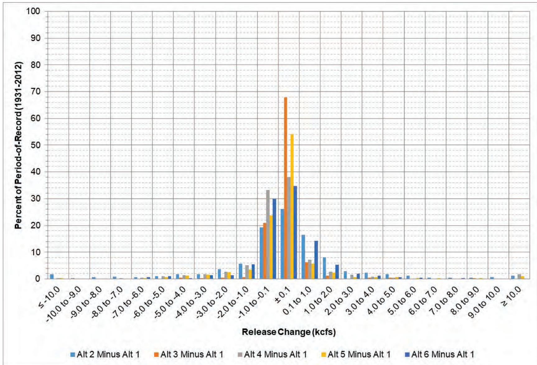
Figure 6-4: Garrison release change between each alternative and Alt 1 for all days in the period-of-record.
