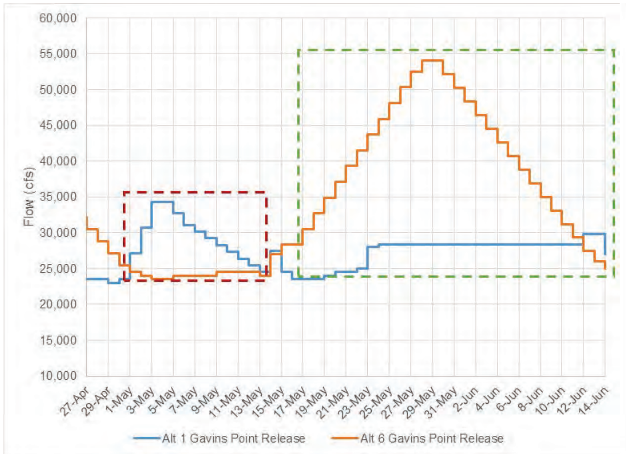
Figure 3-9: Alt 1 vs Alt 6 late spring spawning cue.
