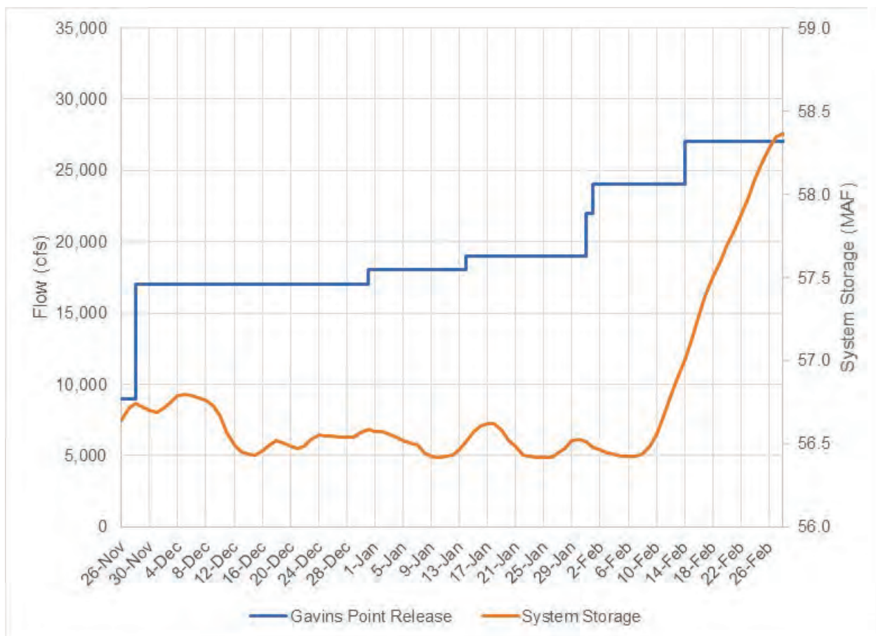
Figure 5-1: High winter releases from Gavins Point Dam.
