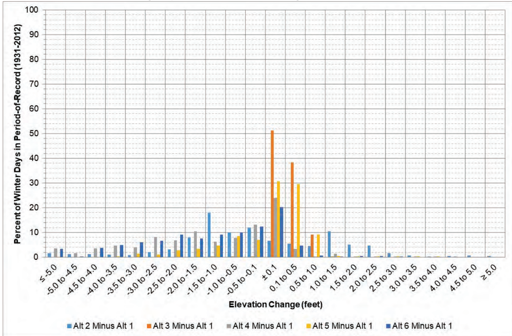
Figure 5-6: Fort Peck elevation change between each alternative and Alt 1 during December – February.
