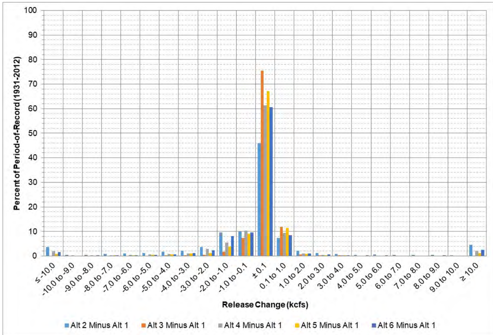
Figure 9-58: Fort Randall release change between each alternative and Alt 1 for all days in the period-of-record.
