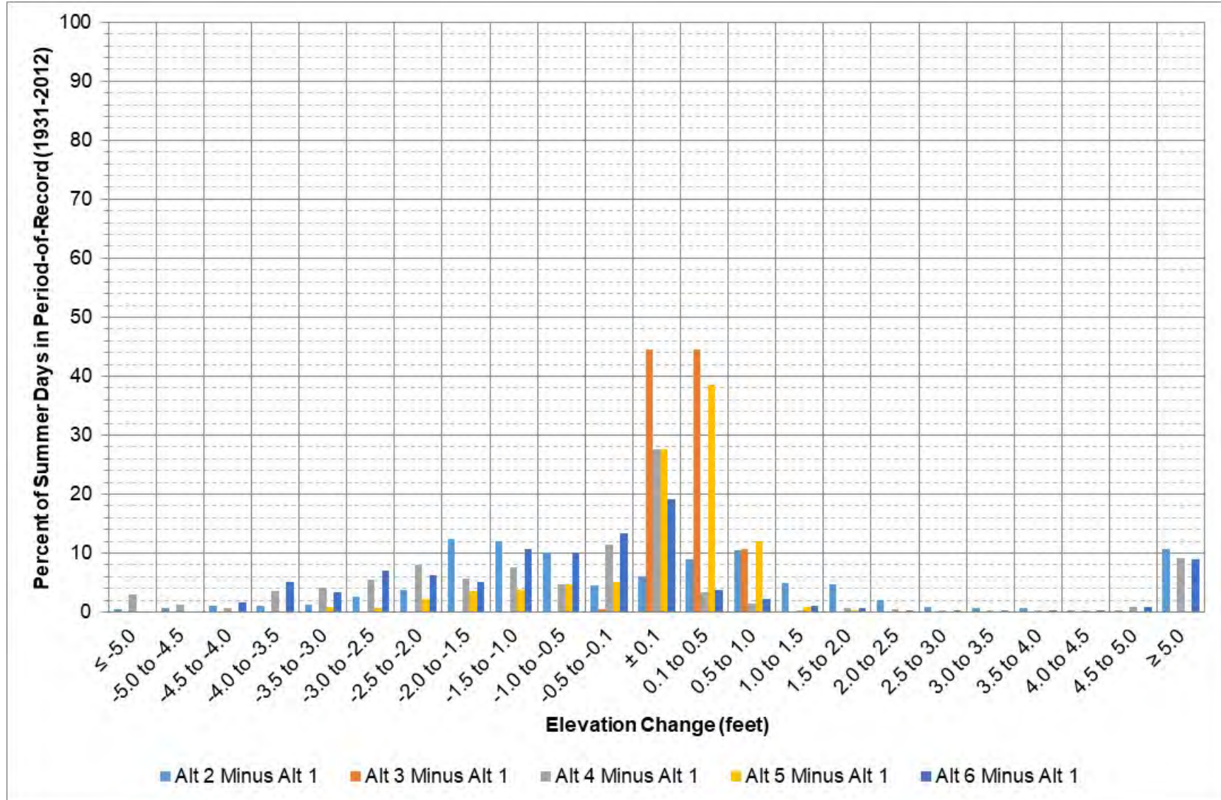
Figure 9-13: Fort Peck elevation change between each alternative and Alt 1 during May – August.
