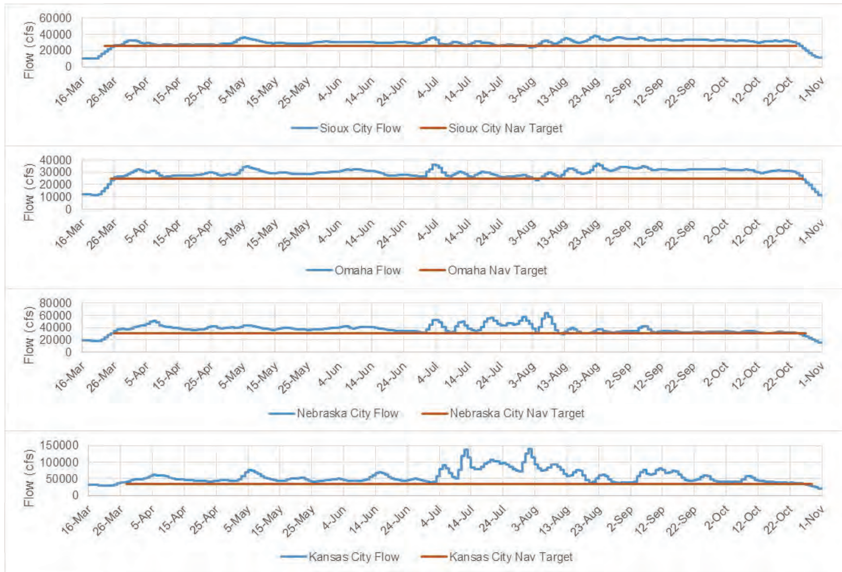
Figure 2-3: Navigation target locations with target and simulated flows.
