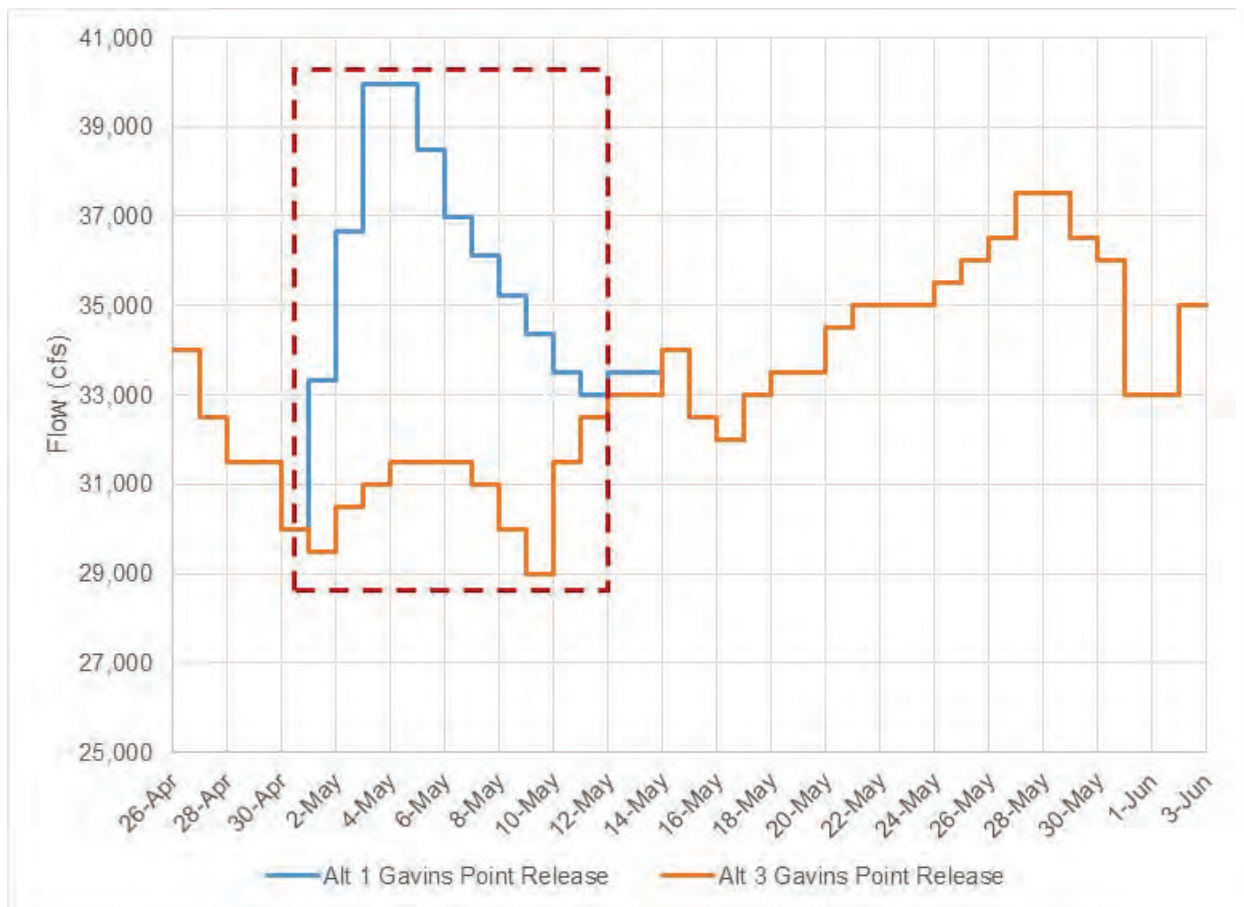
Figure 3-7: Alt 1 late spring spawning cue vs Alt 3 FTT navigation releases.
