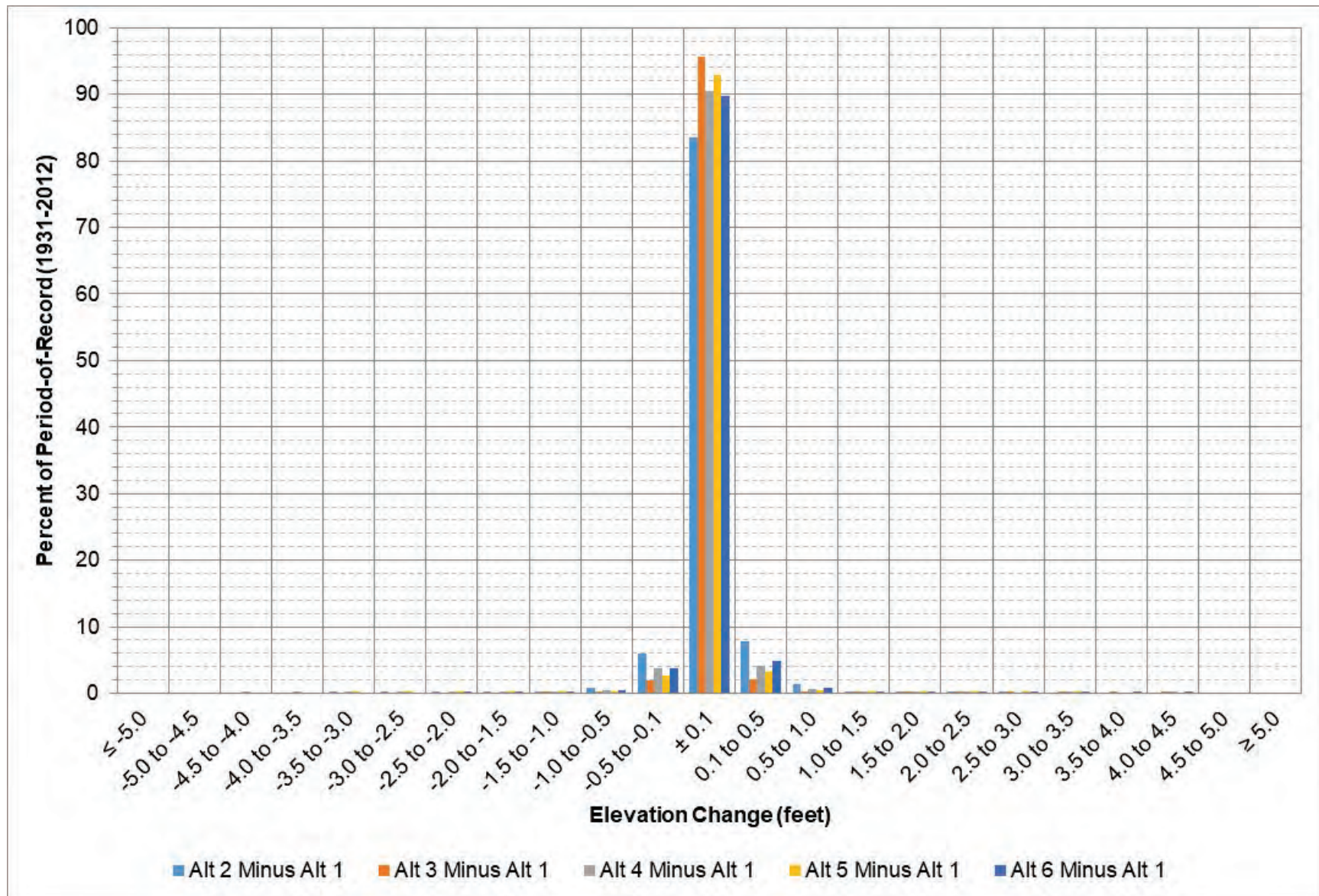
Figure 6-11: Gavins Point elevation change between each alternative and Alt 1 for all days in the period-of-record.
