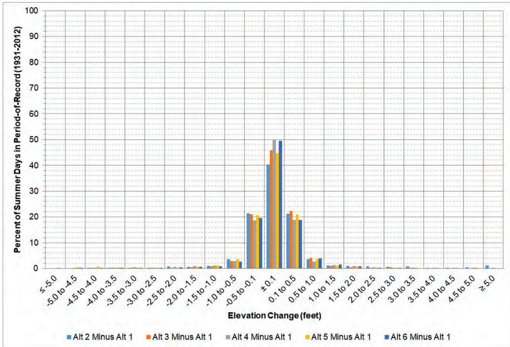
Figure 3-22: Fort Randall elevation change between each alternative and Alt 1 during May – August.
