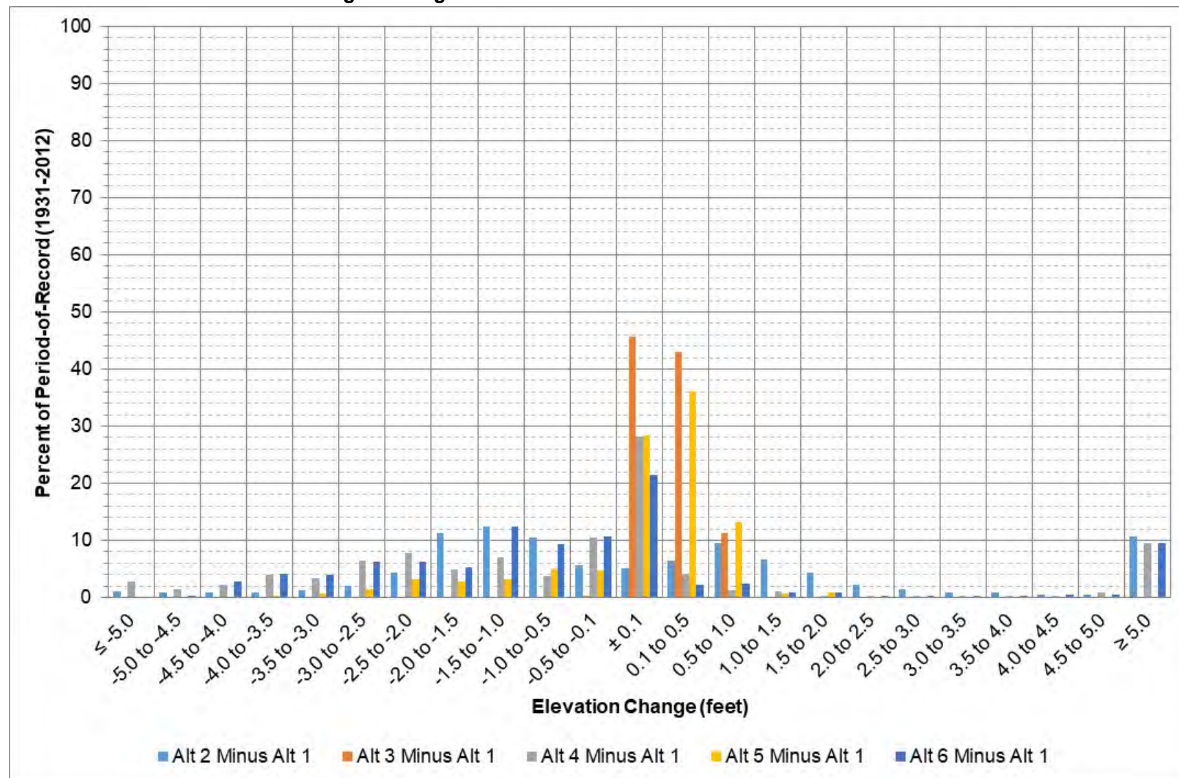
Figure 9-49: Fort Peck elevation change between each alternative and Alt 1 for all days in the period-of-record.
