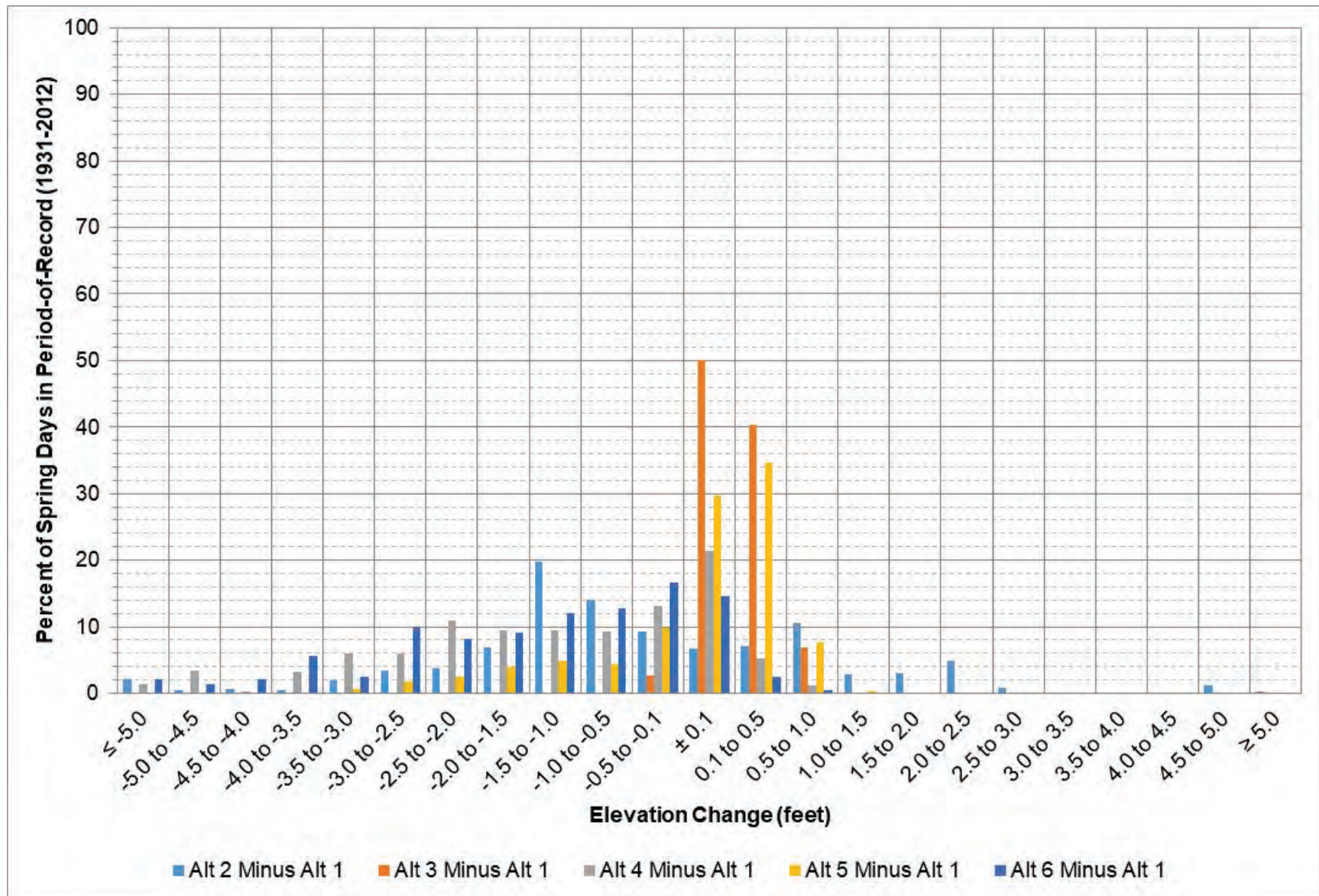
Figure 2-21: Oahe elevation change between each alternative and Alt 1 during March – April.
