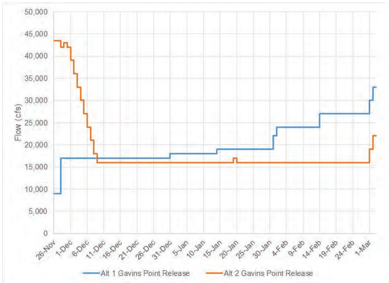
Figure 5-3: Alt 2's vs Alt 1's winter release during a flood evacuation winter.
