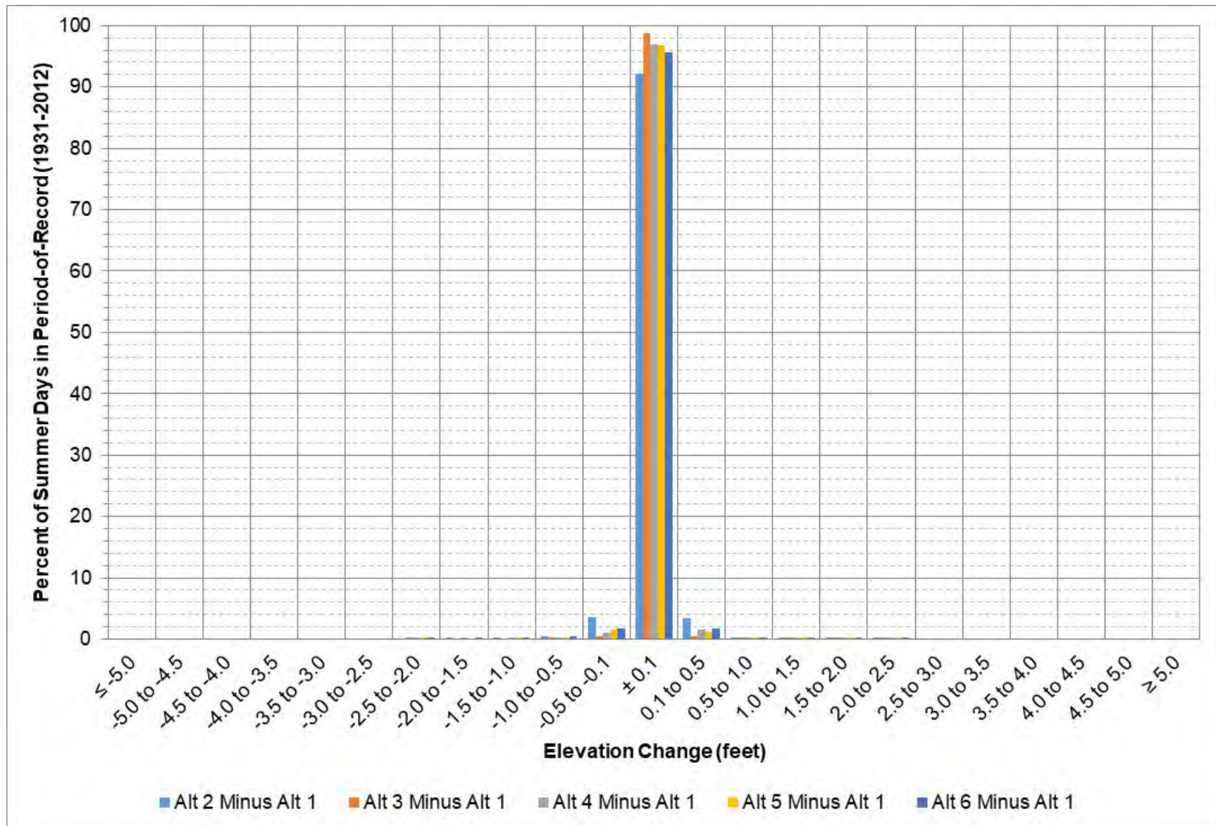
Figure 9-19: Big Bend elevation change between each alternative and Alt 1 during May – August.
