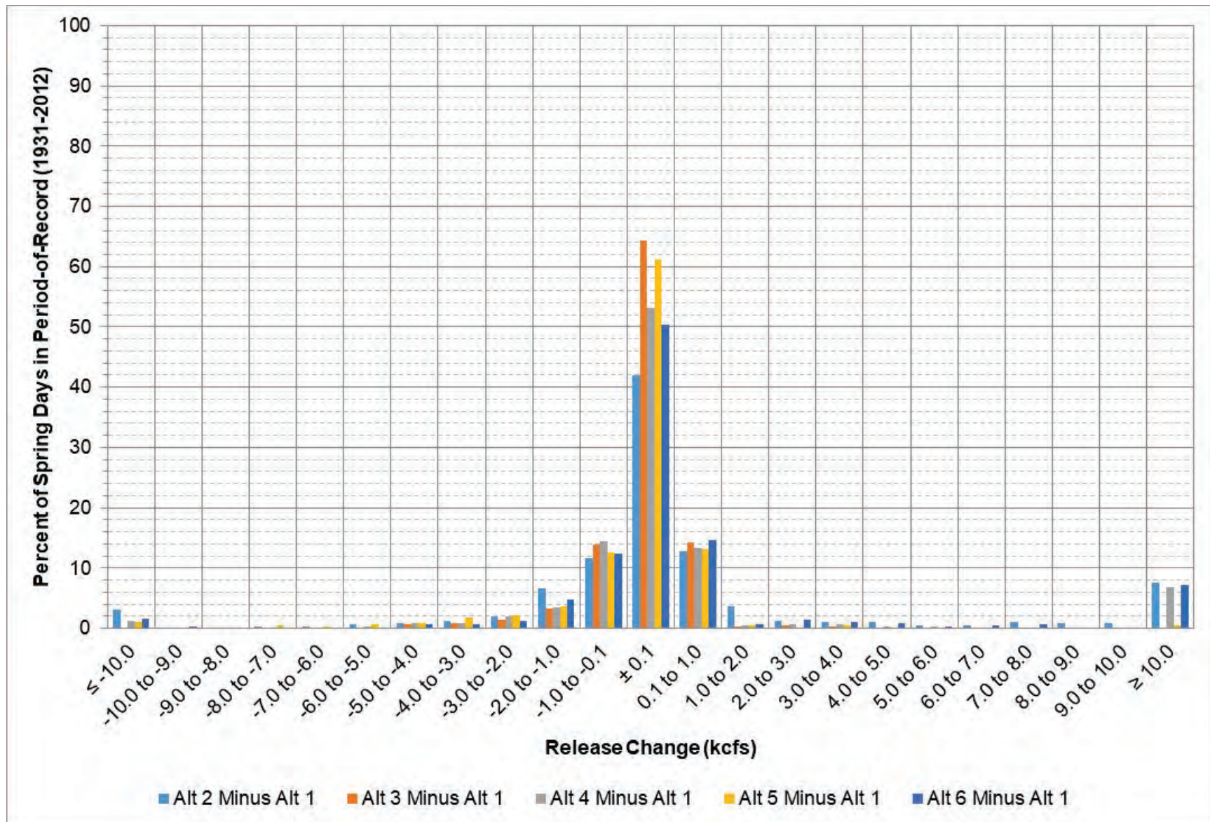
Figure 9-6: Oahe release change between each alternative and Alt 1 during March – April.
