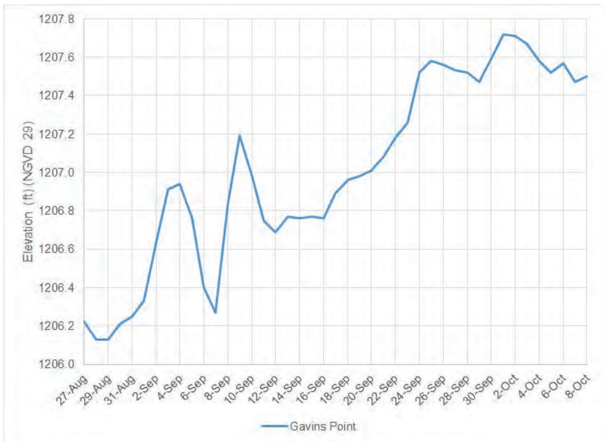
Figure 3-12: Gavins Point summer pool elevation rise.
