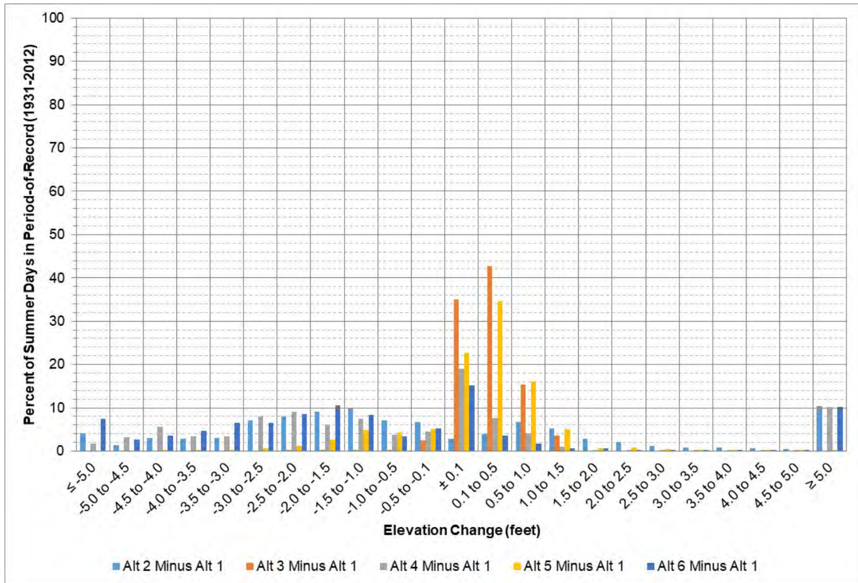
Figure 9-17: Oahe elevation change between each alternative and Alt 1 during May – August.
