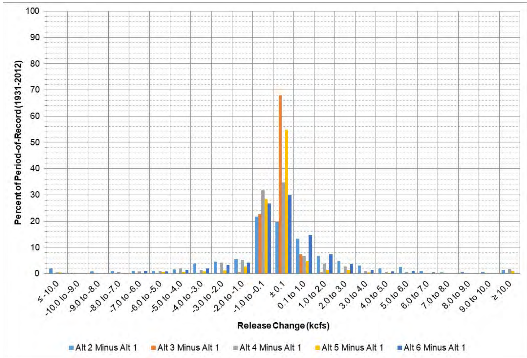
Figure 9-52: Garrison release change between each alternative and Alt 1 for all days in the period-of-record.
