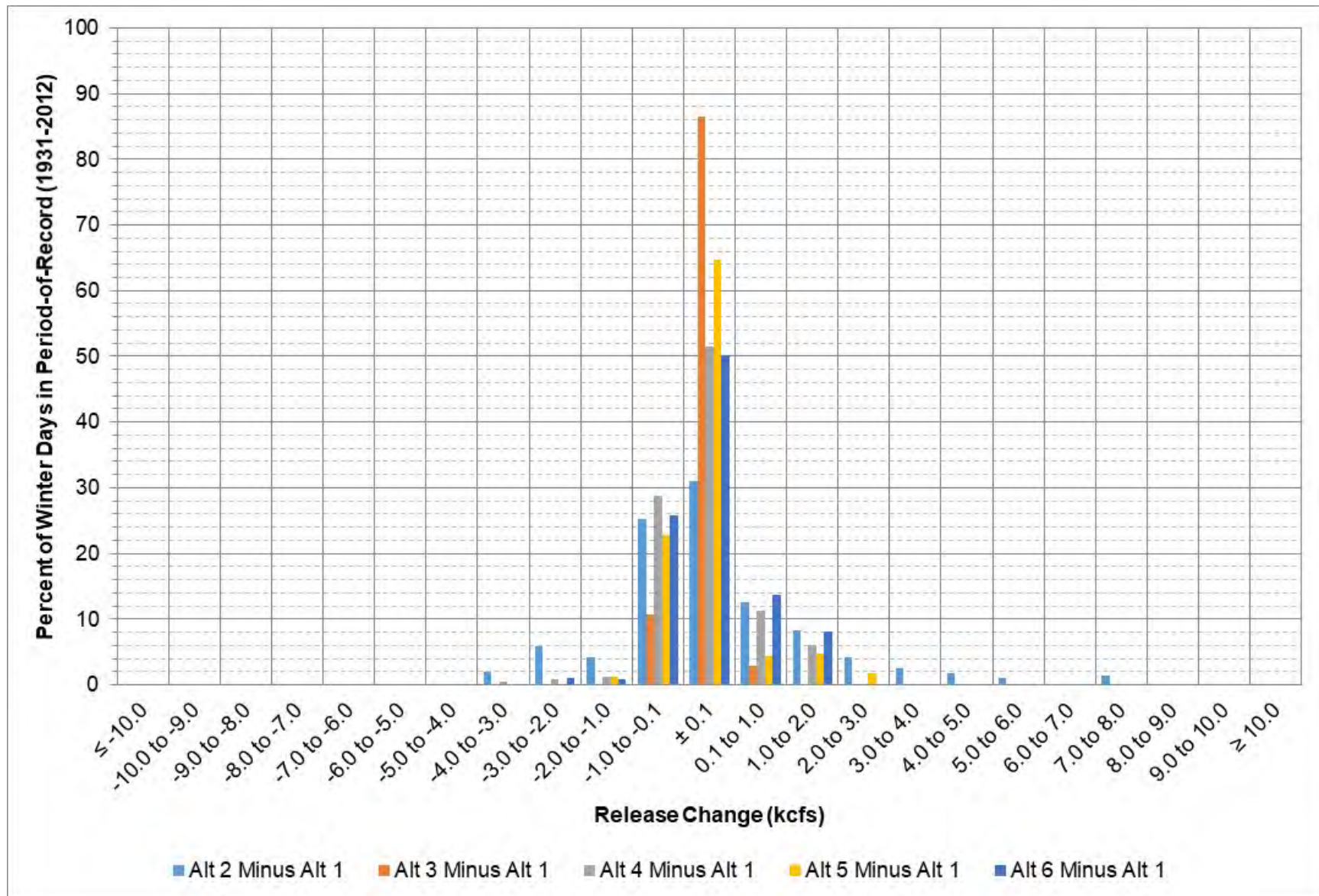
Figure 9-38: Fort Peck release change between each alternative and Alt 1 during December – February.
