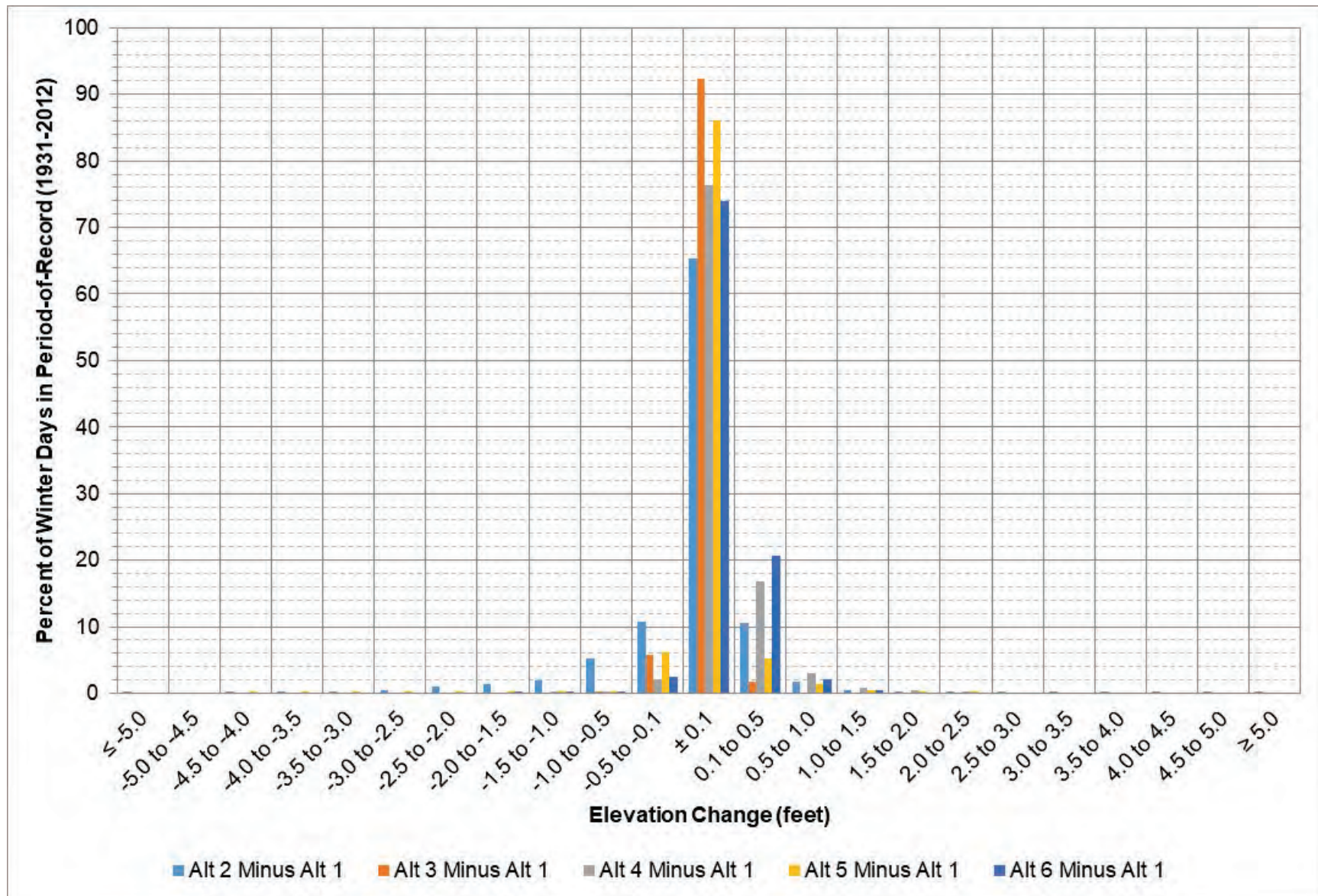
Figure 5-14: Fort Randall elevation change between each alternative and Alt 1 during December – February.
