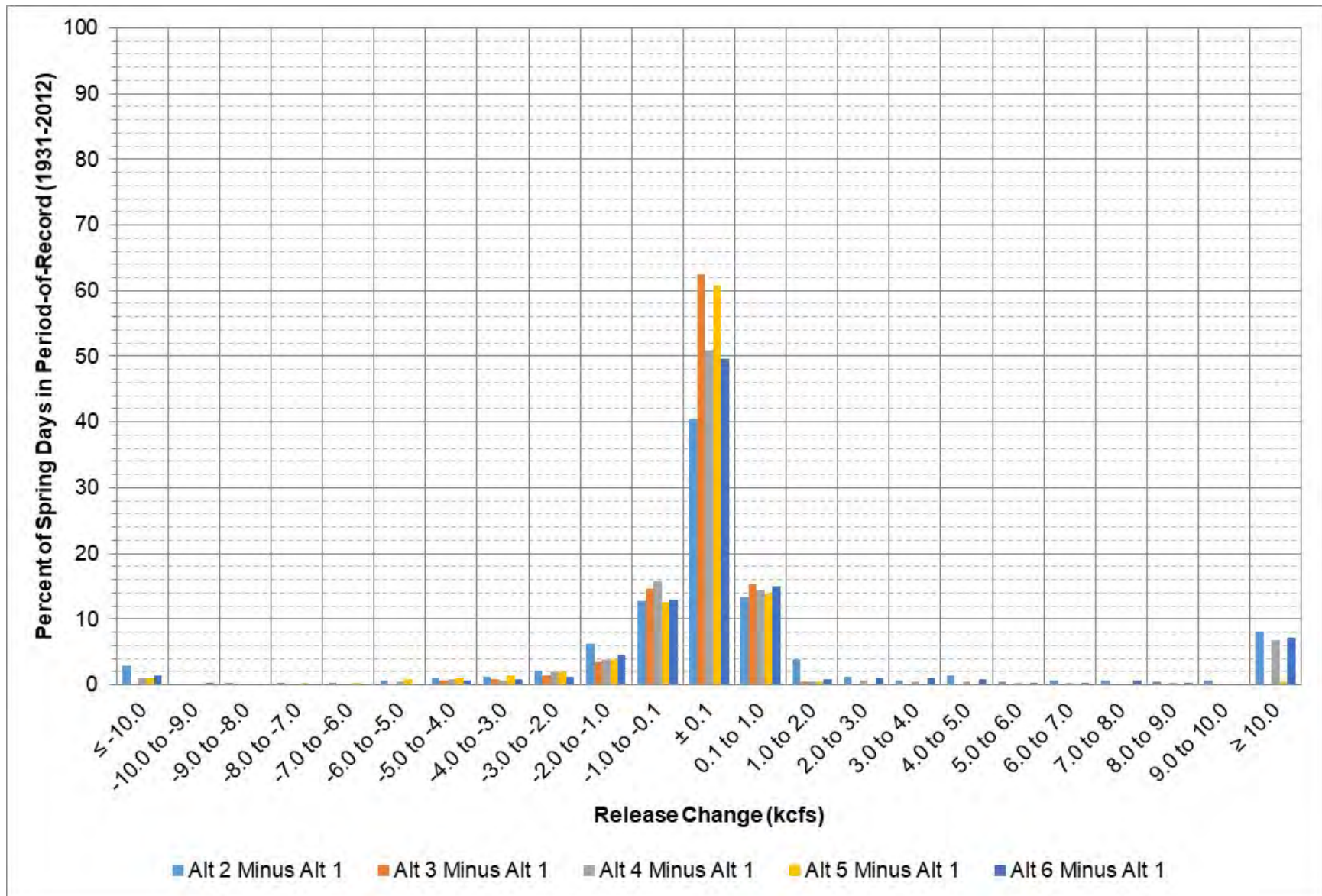
Figure 9-8: Big Bend release change between each alternative and Alt 1 during March – April.
