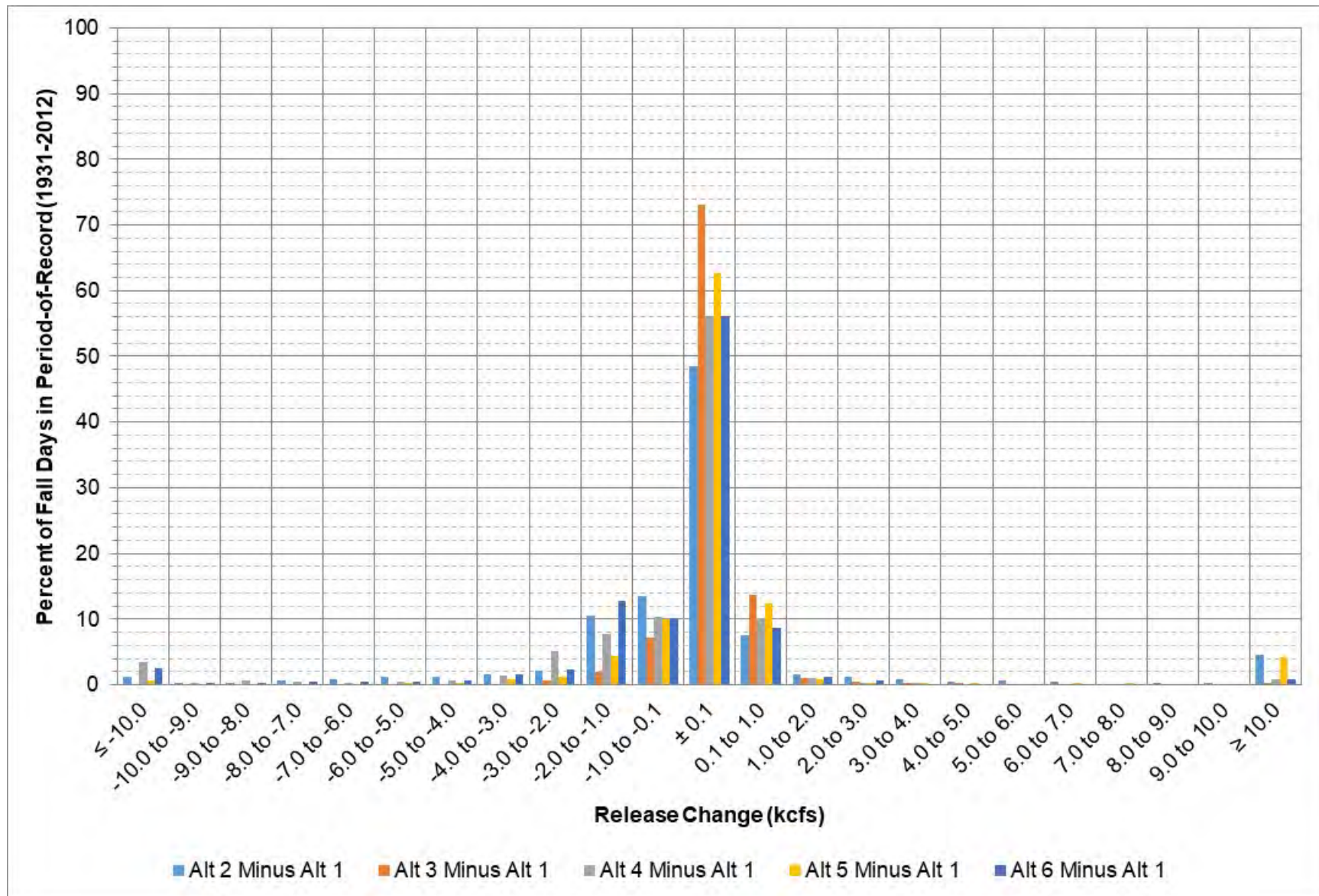
Figure 9-34: Fort Randall release change between each alternative and Alt 1 during September – November.
