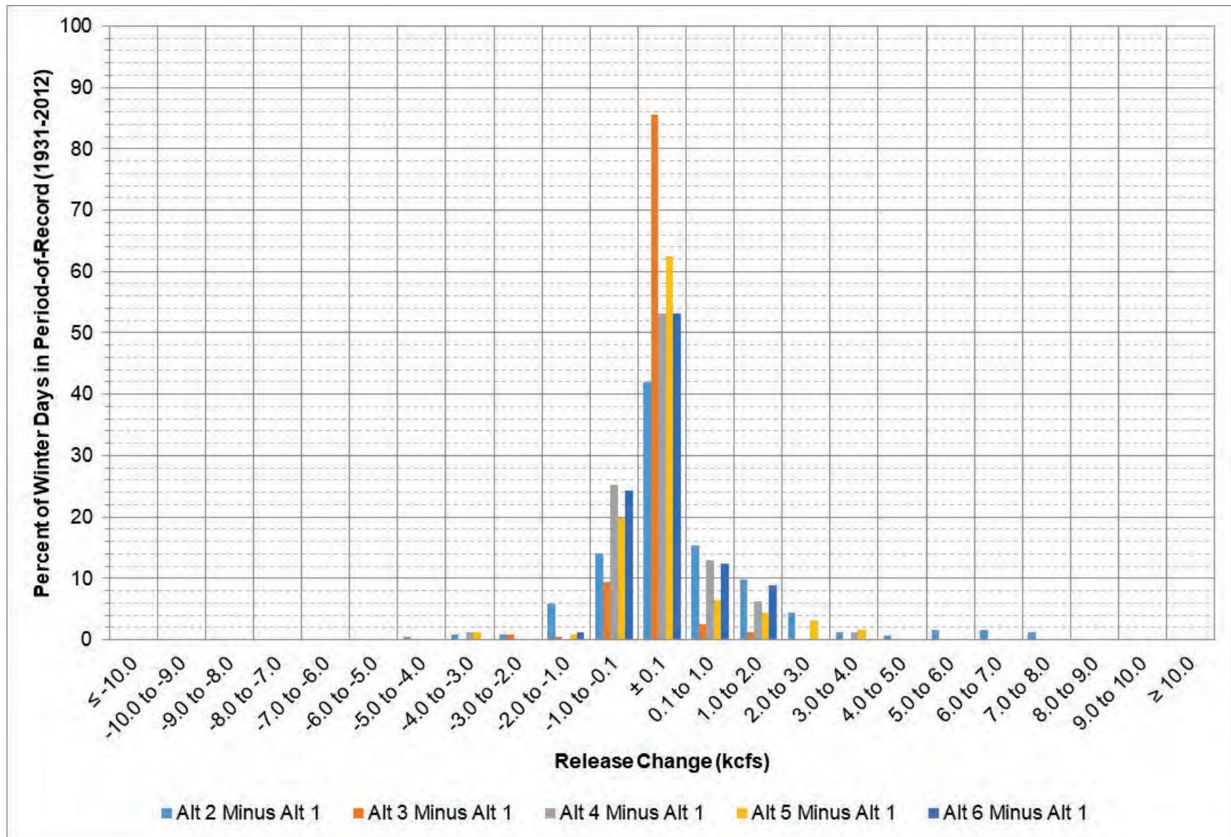
Figure 5-7: Fort Peck release change between each alternative and Alt 1 during December – February.
