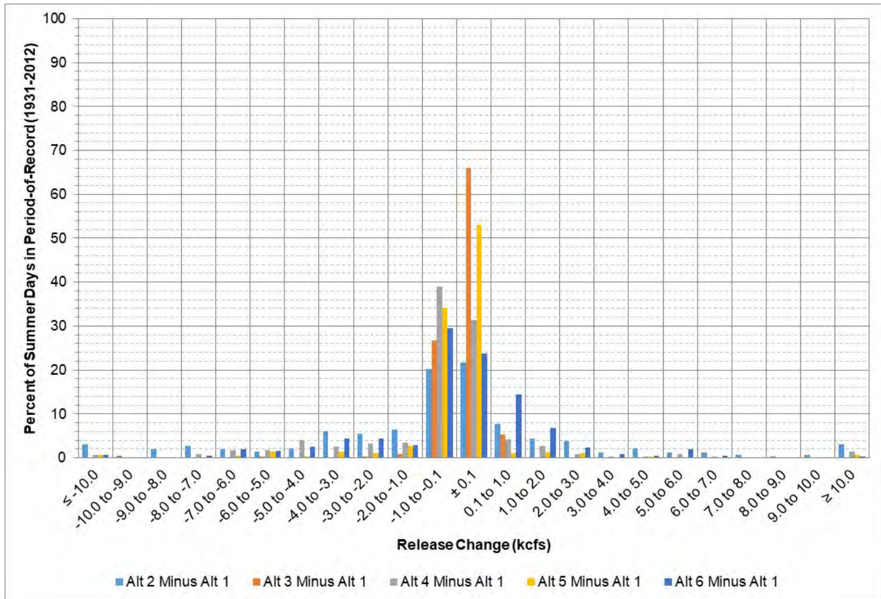
Figure 9-16: Garrison release change between each alternative and Alt 1 during May – August.
