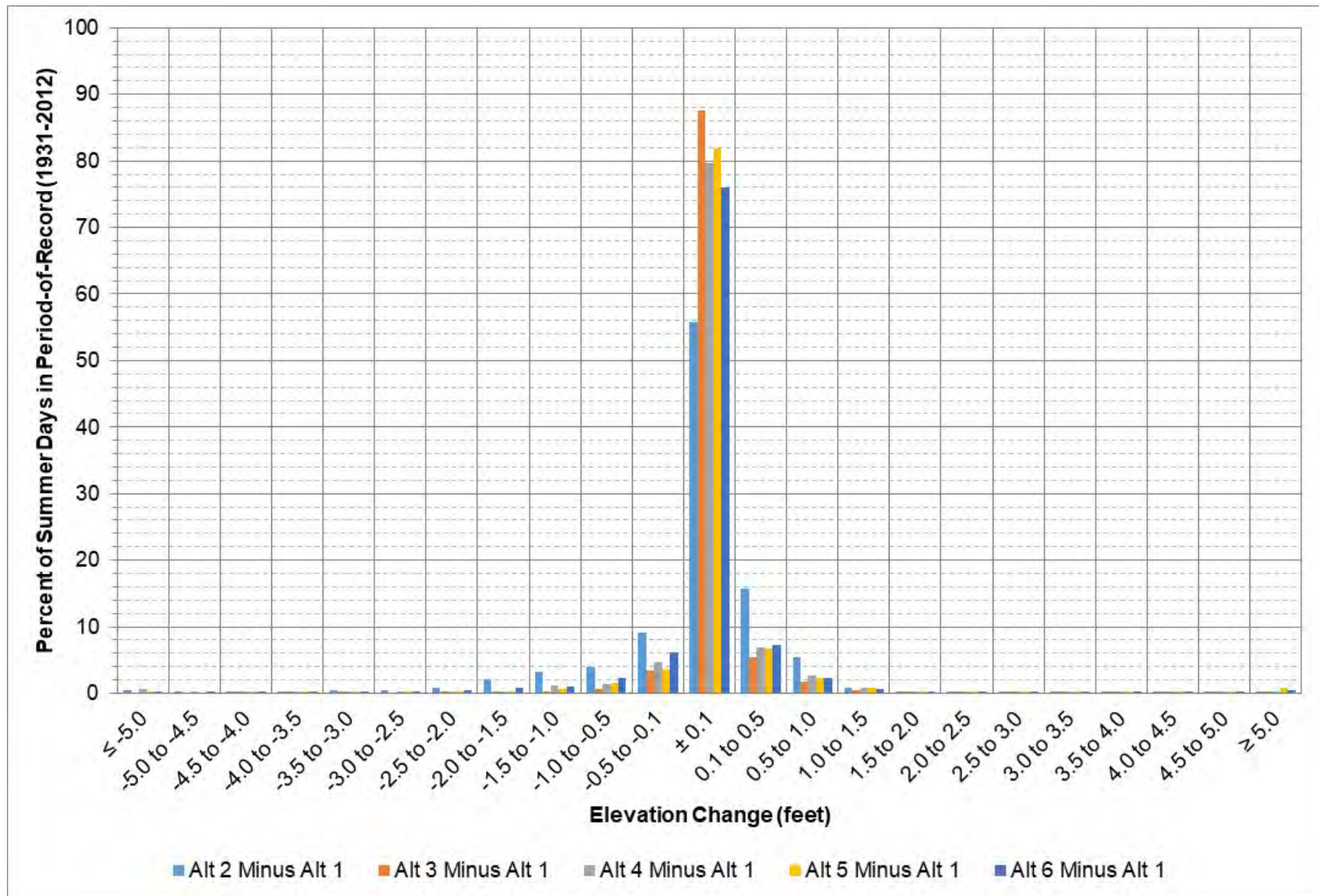
Figure 9-21: Fort Randall elevation change between each alternative and Alt 1 during May – August.
