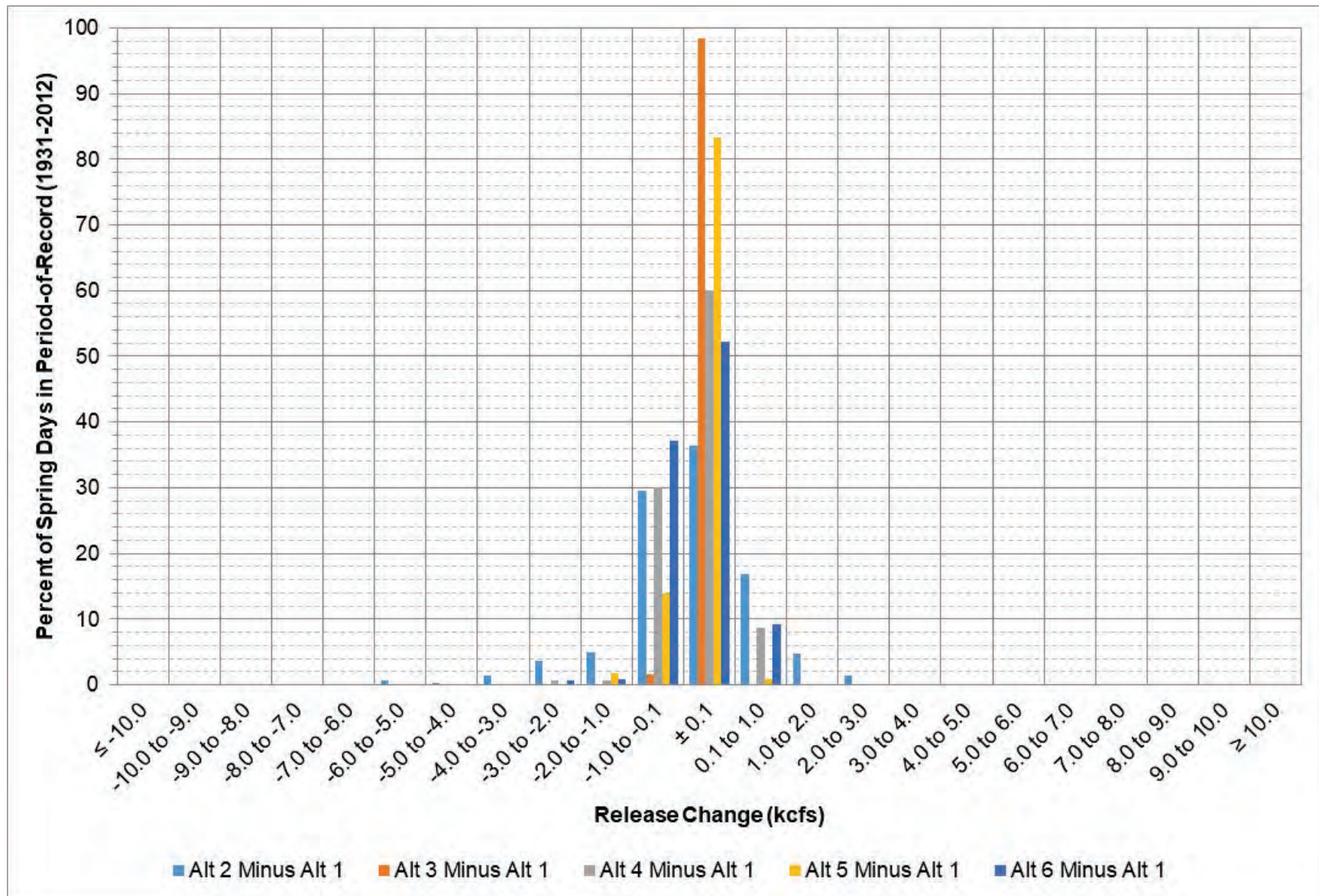
Figure 9-2: Fort Peck release change between each alternative and Alt 1 during March – April.
