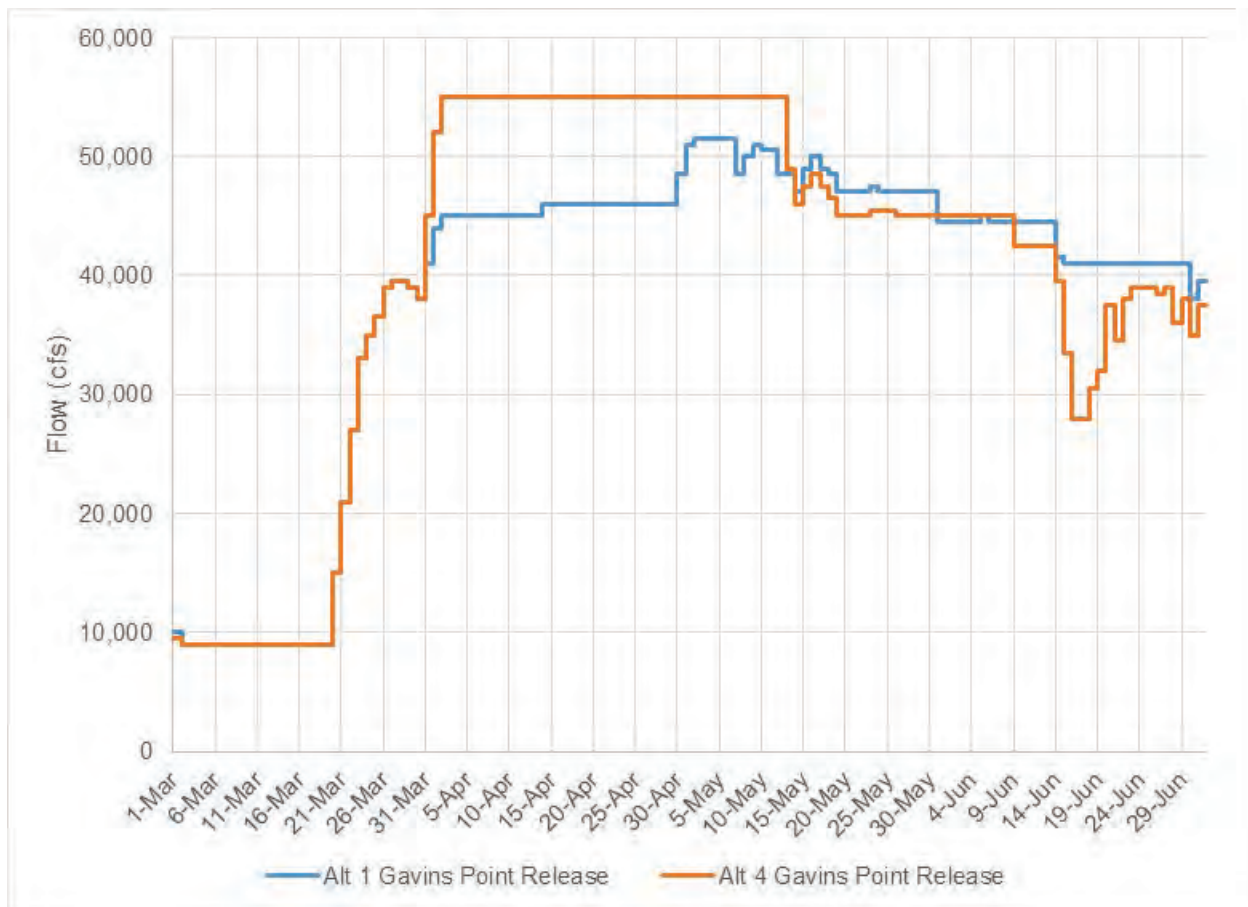
Figure 3-8: Comparison of Gavins Point releases in Alt 1 and Alt 4 during an extended ESH-creating release.
