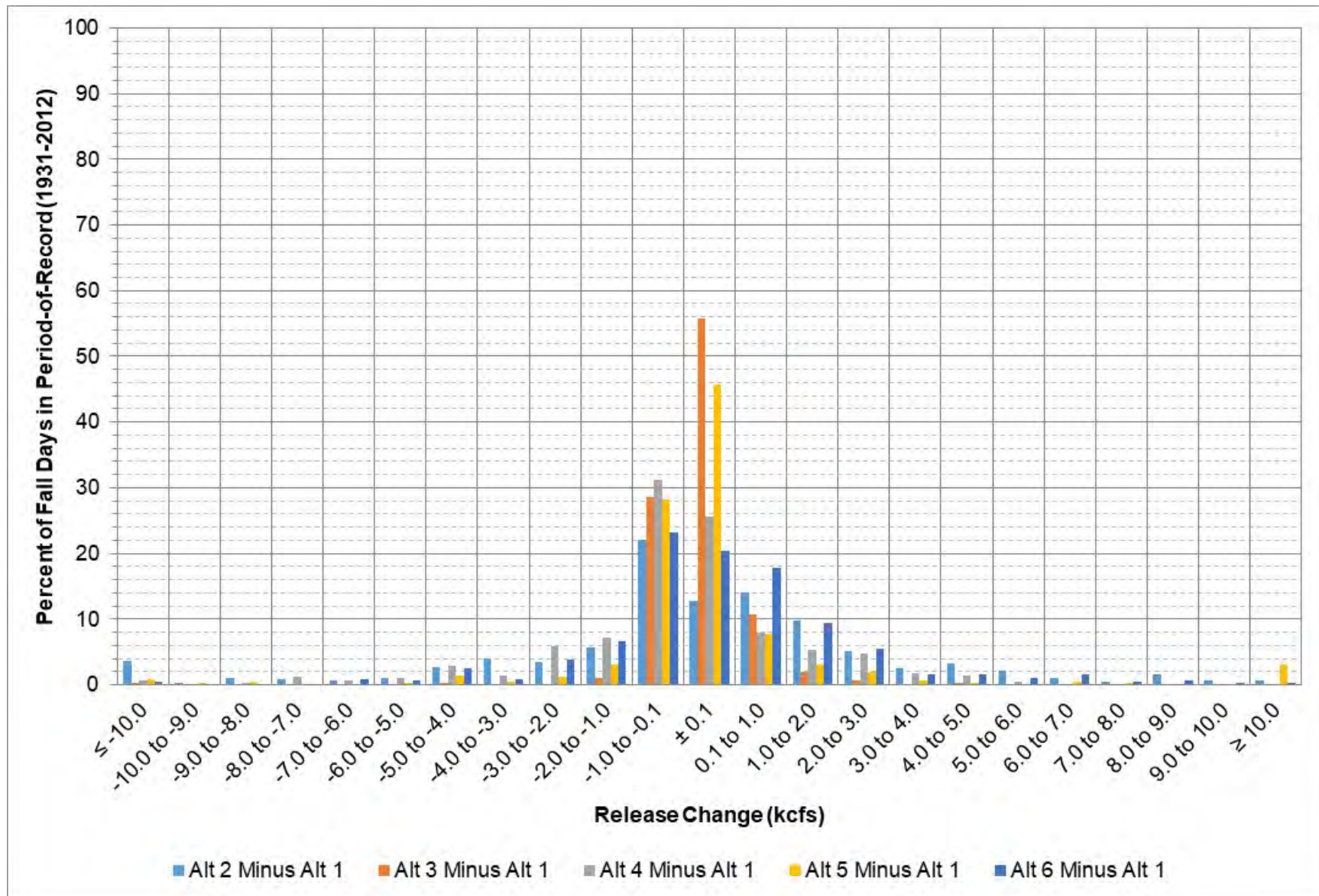
Figure 9-28: Garrison release change between each alternative and Alt 1 during September – November.
