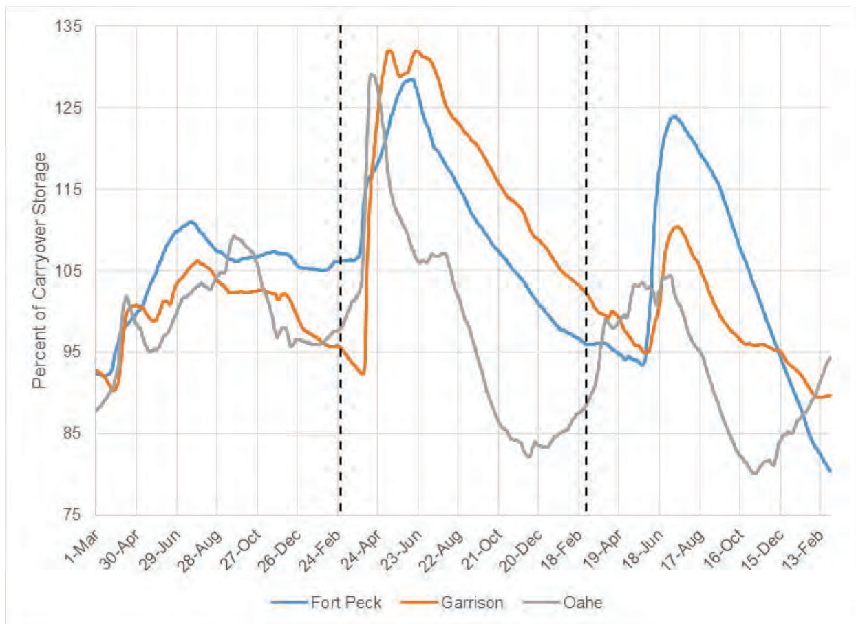
Figure 2-14: Storage unbalancing at Fort Peck, Garrison, and Oahe. Year 1: Fort Peck high, Garrison low, Oahe float. Year 2: Fort Peck float, Garrison high, Oahe low. Year 3: Fort Peck low, Garrison float, Oahe high.
