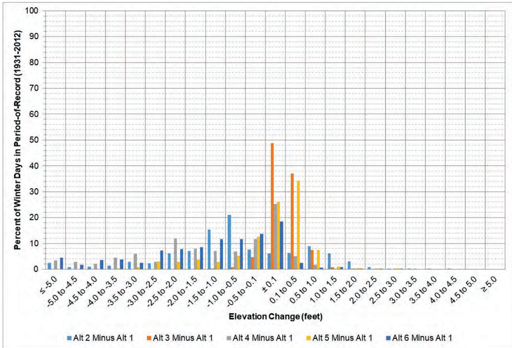
Figure 5-10: Oahe elevation change between each alternative and Alt 1 during December – February.
