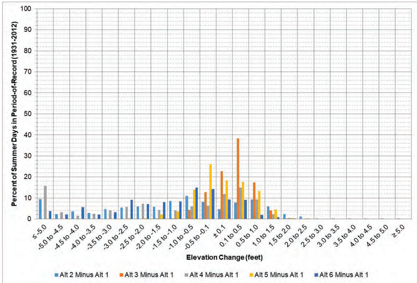
Figure 3-18: Oahe elevation change between each alternative and Alt 1 during May – August.
