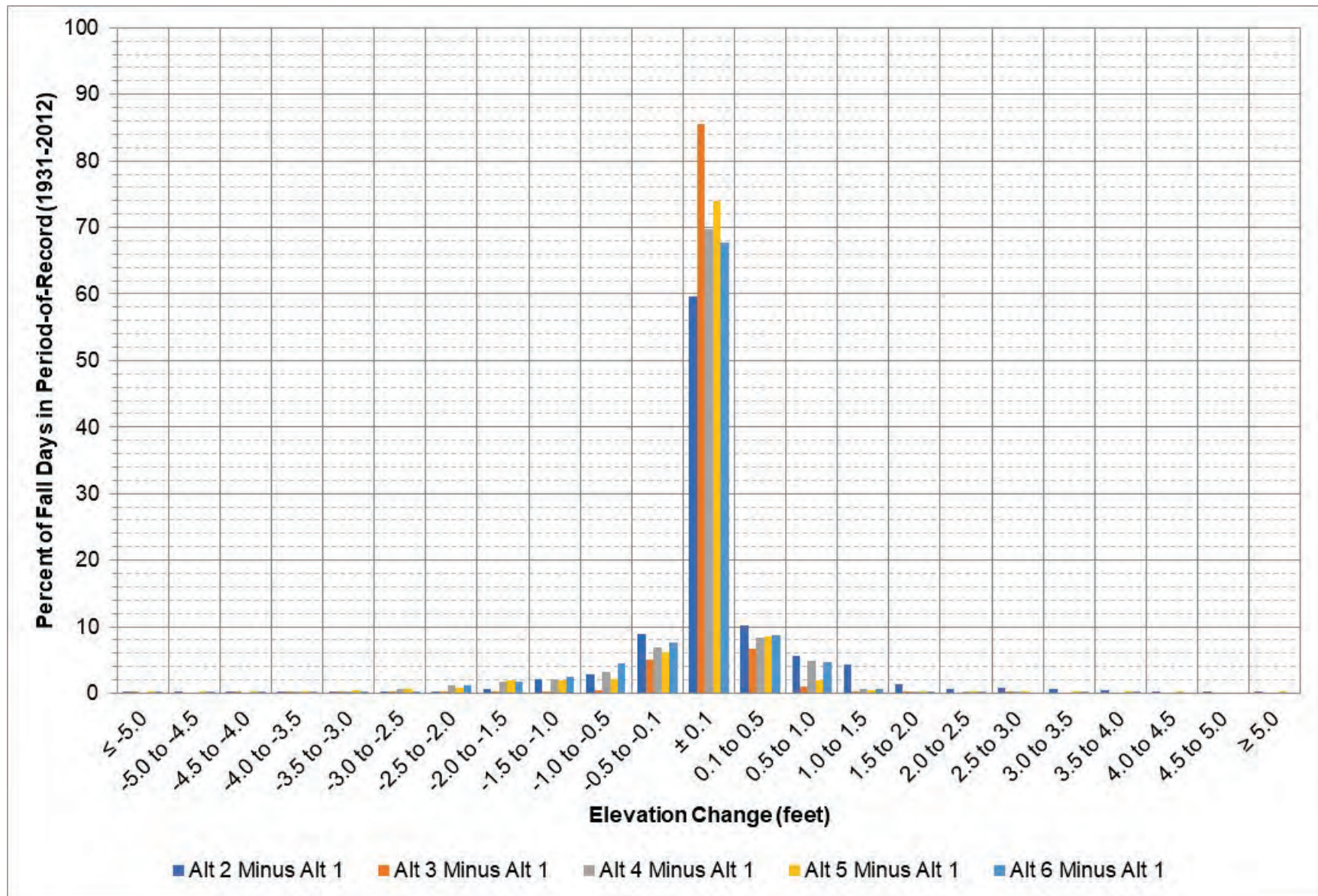
Figure 4-18: Fort Randall elevation change between each alternative and Alt 1 during September – November.
