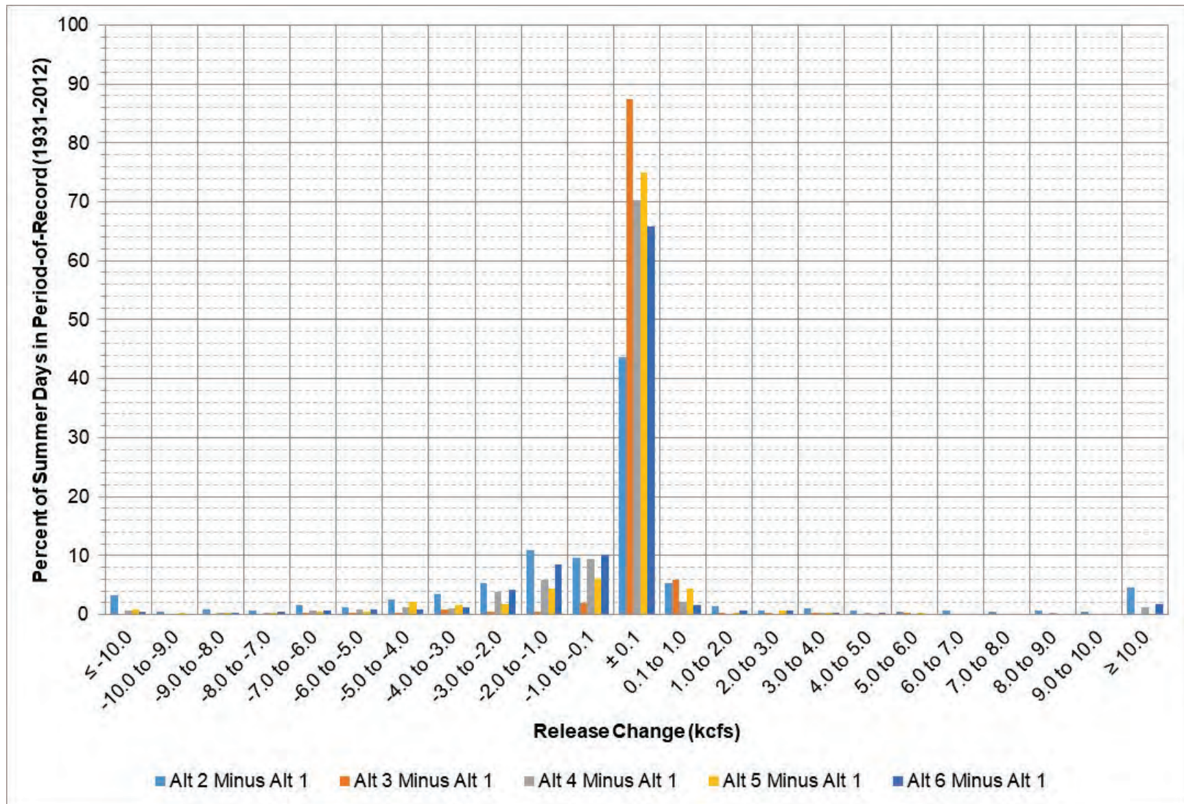
Figure 3-11: Gavins Point release change between each alternative and Alt 1 during May – August.
