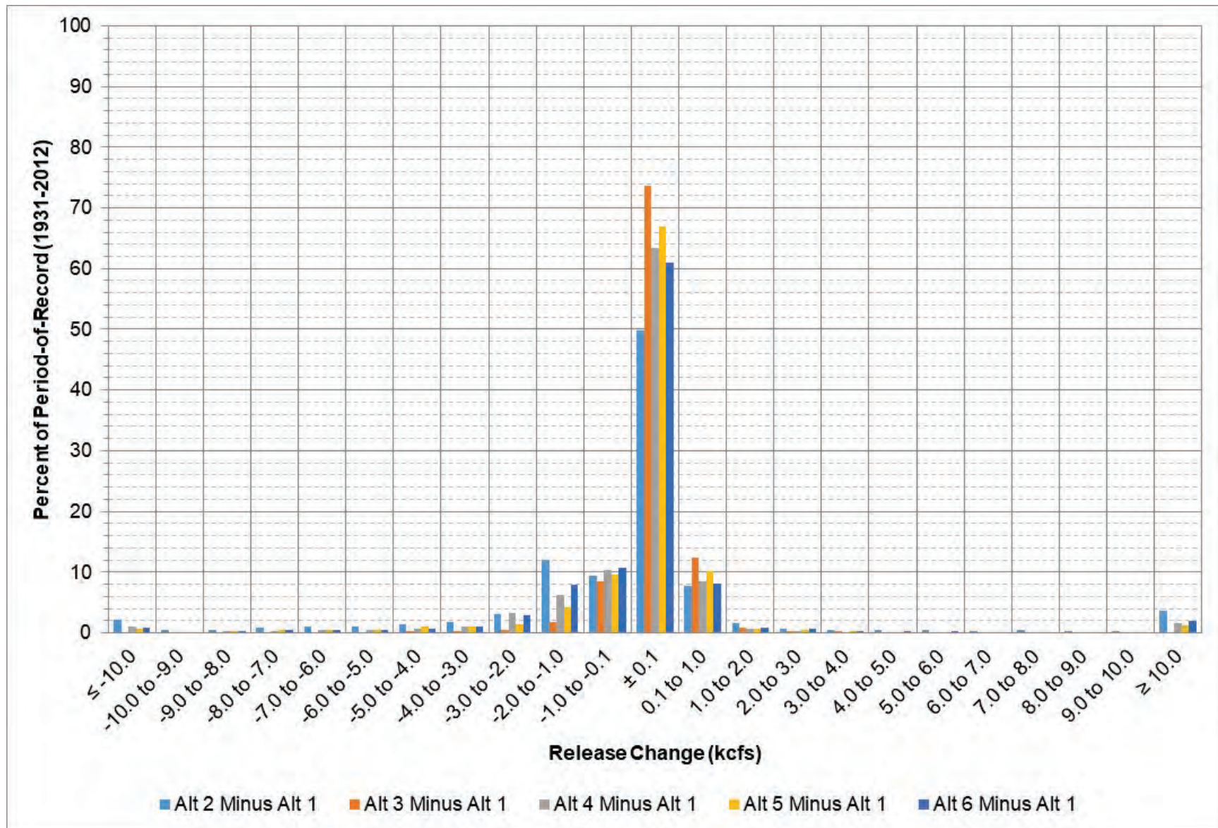
Figure 6-10: Fort Randall release change between each alternative and Alt 1 for all days in the period-of-record.
