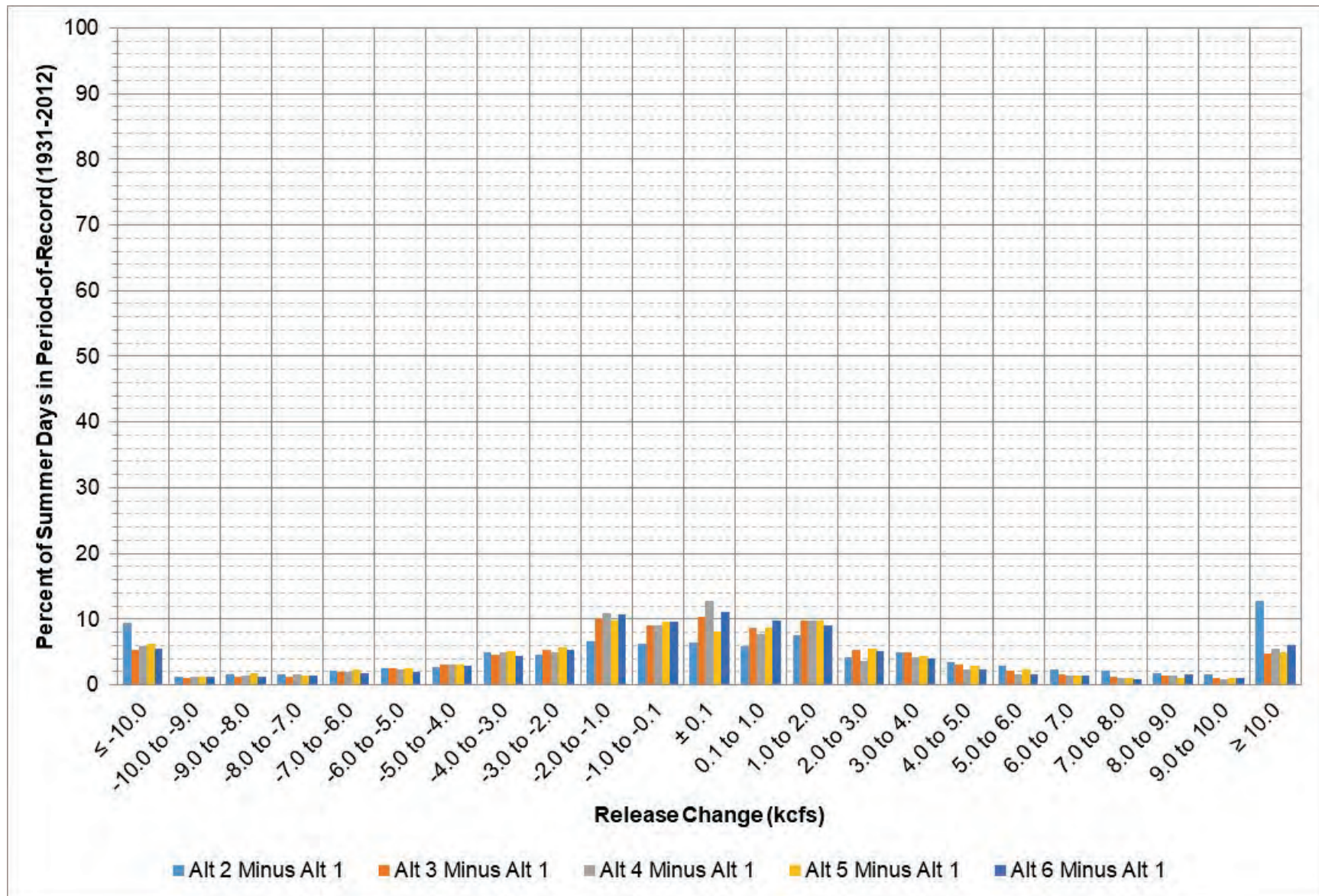
Figure 3-21: Big Bend release change between each alternative and Alt 1 during May – August.
