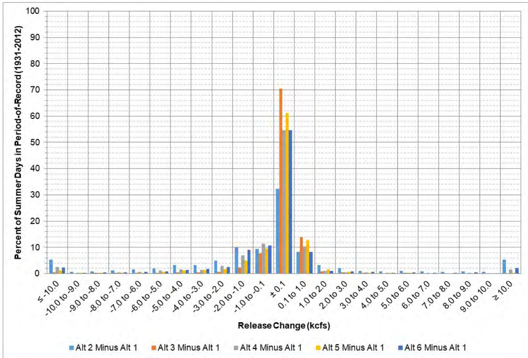
Figure 9-22: Fort Randall release change between each alternative and Alt 1 during May – August.
