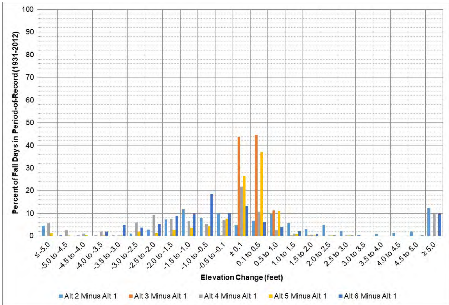
Figure 9-27: Garrison elevation change between each alternative and Alt 1 during September – November.
