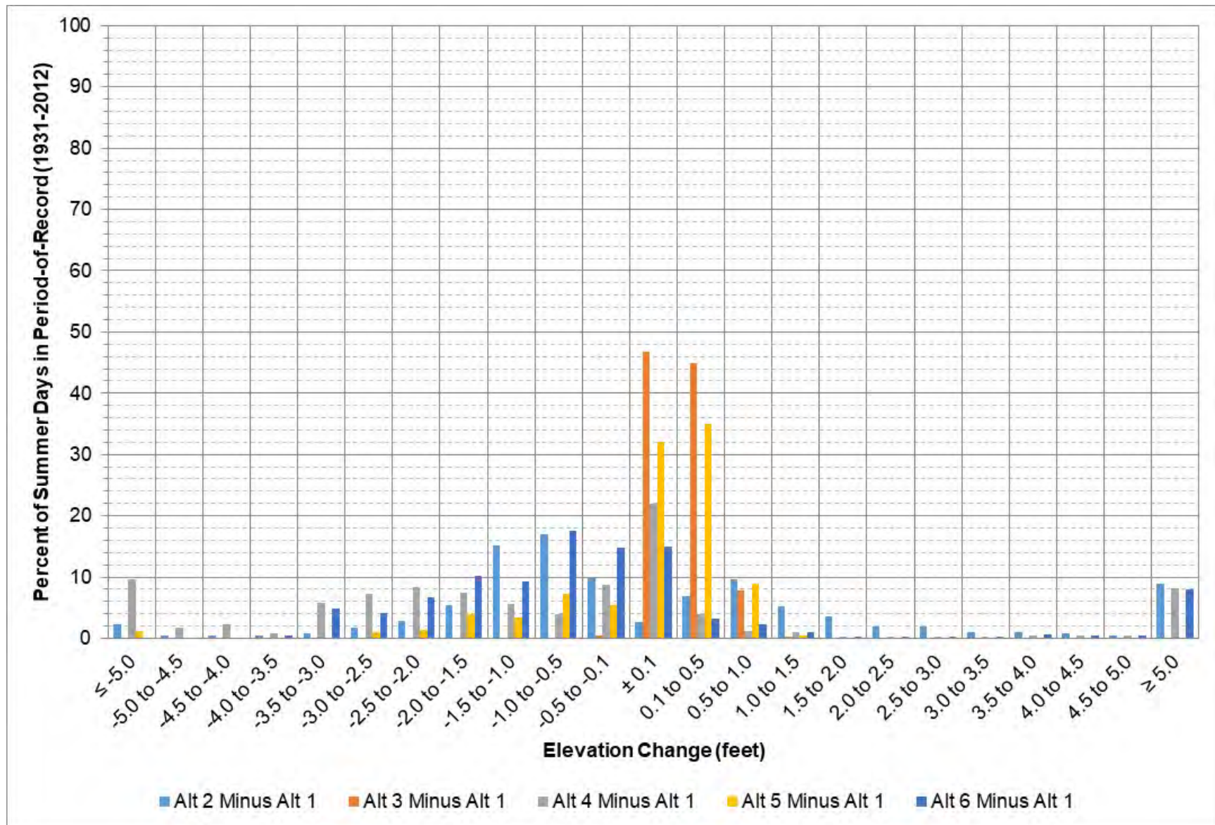
Figure 9-15: Garrison elevation change between each alternative and Alt 1 during May – August.
