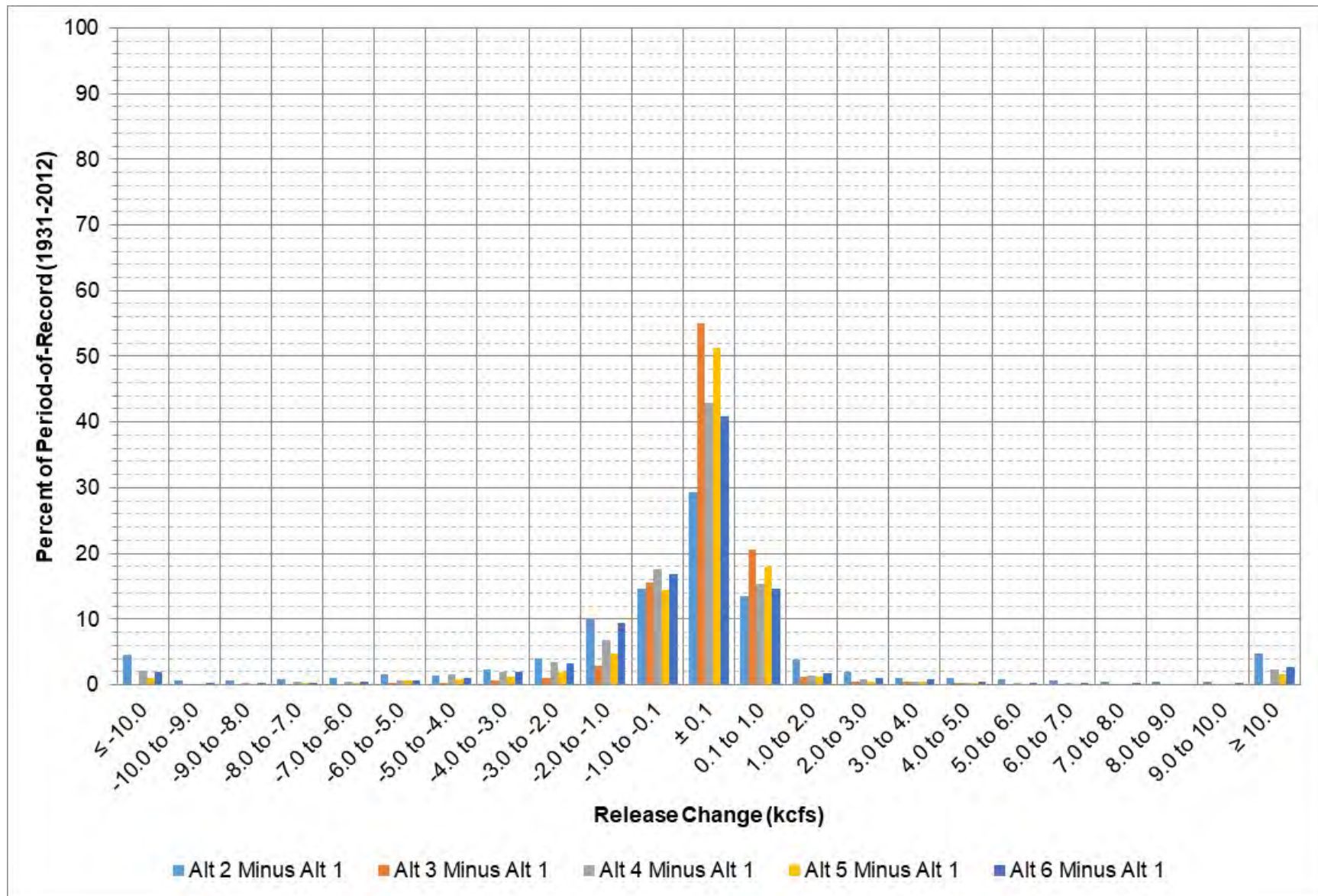
Figure 9-56: Big Bend release change between each alternative and Alt 1 for all days in the period-of-record.
