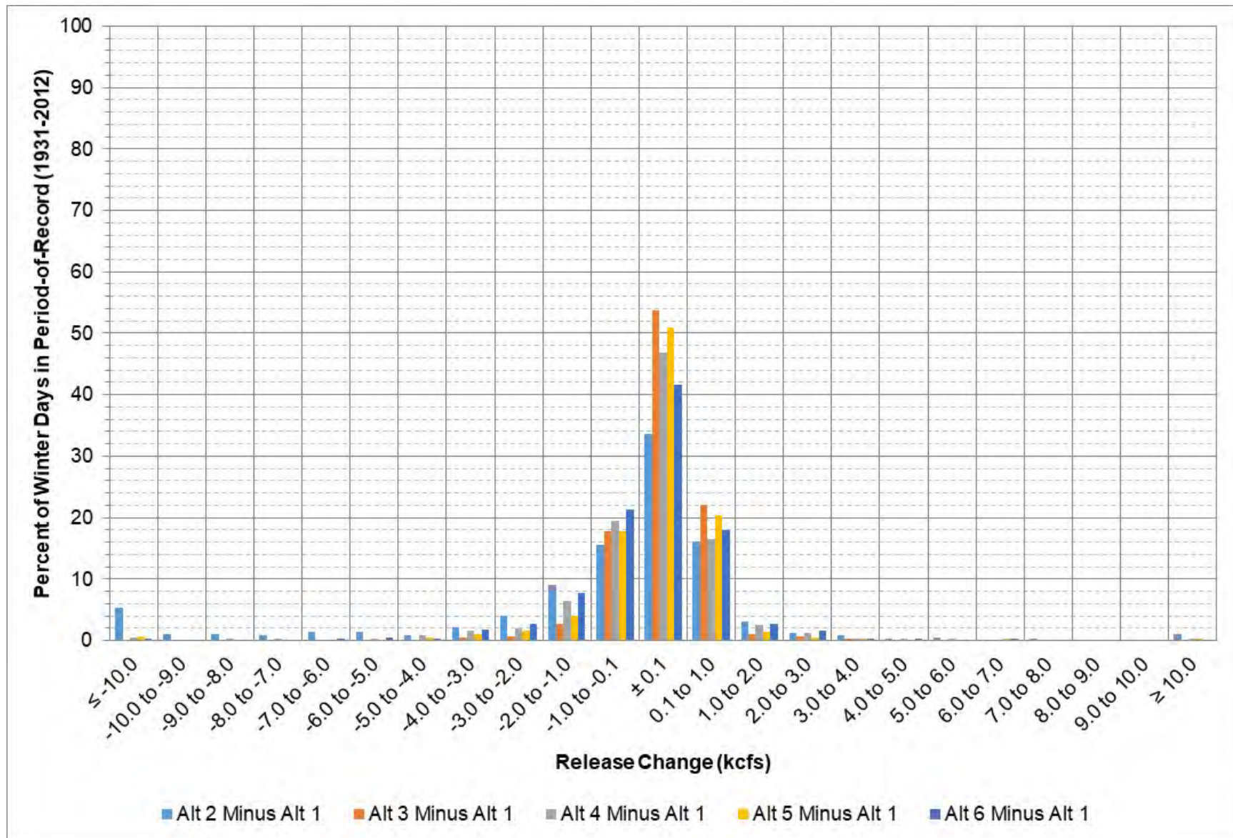
Figure 9-42: Oahe release change between each alternative and Alt 1 during December – February.
