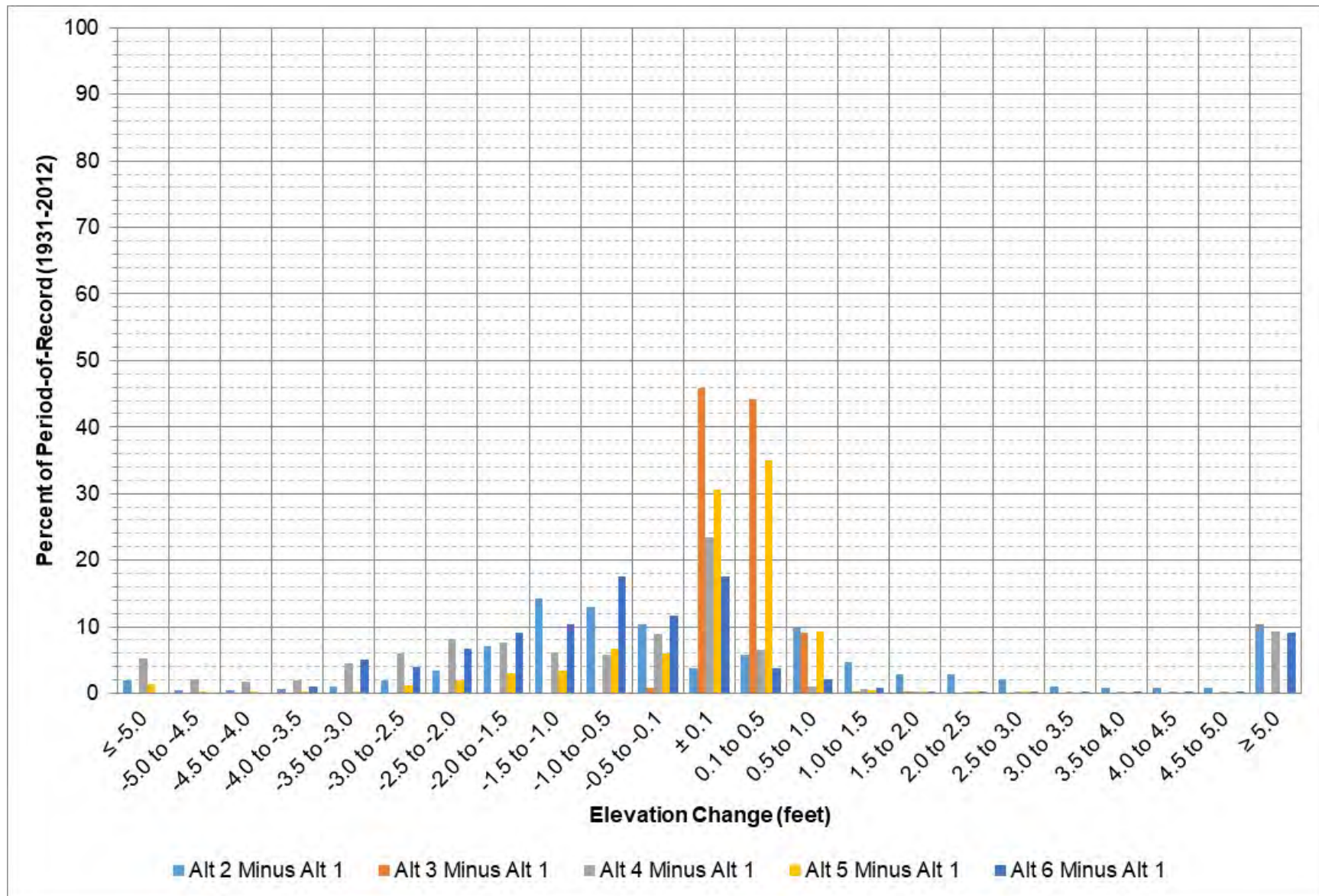
Figure 9-51: Garrison elevation change between each alternative and Alt 1 for all days in the period-of-record.
