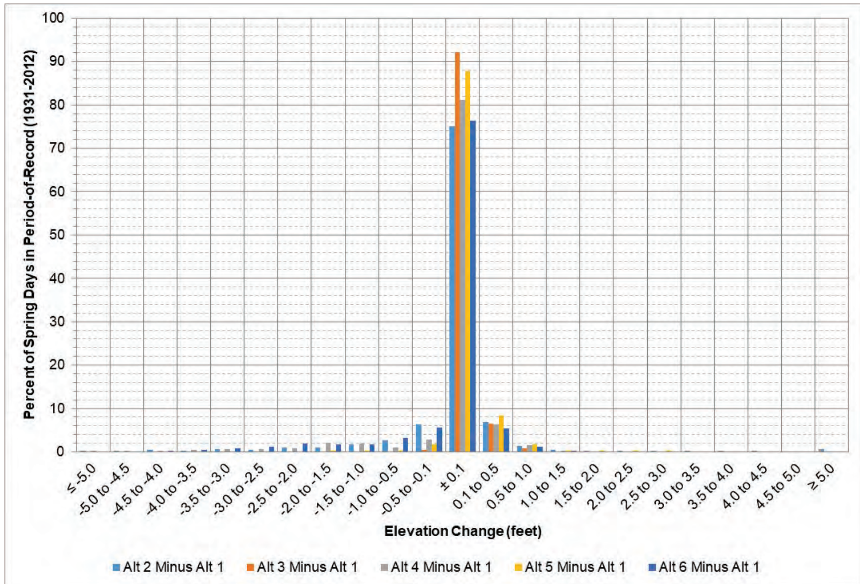
Figure 2-25: Fort Randall elevation change between each alternative and Alt 1 during March – April.
