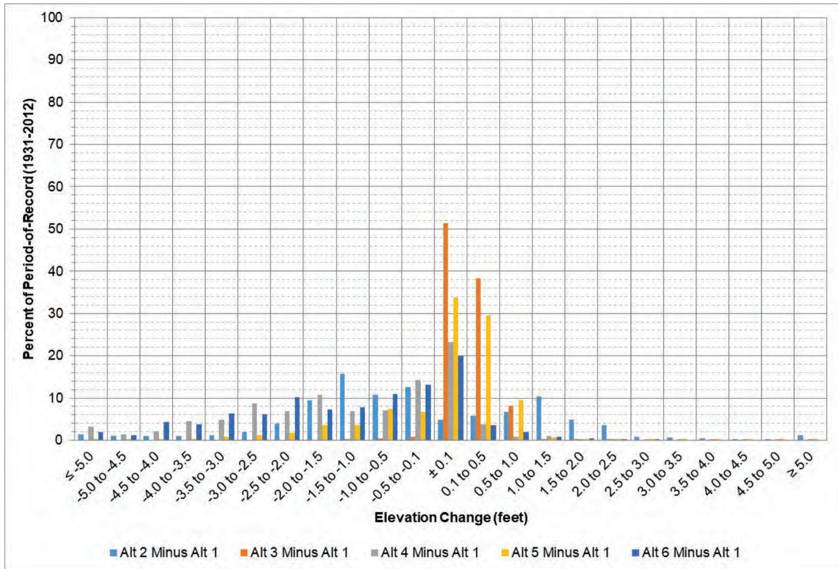
Figure 6-1: Fort Peck elevation change between each alternative and Alt 1 for all days in the period-of-record.
