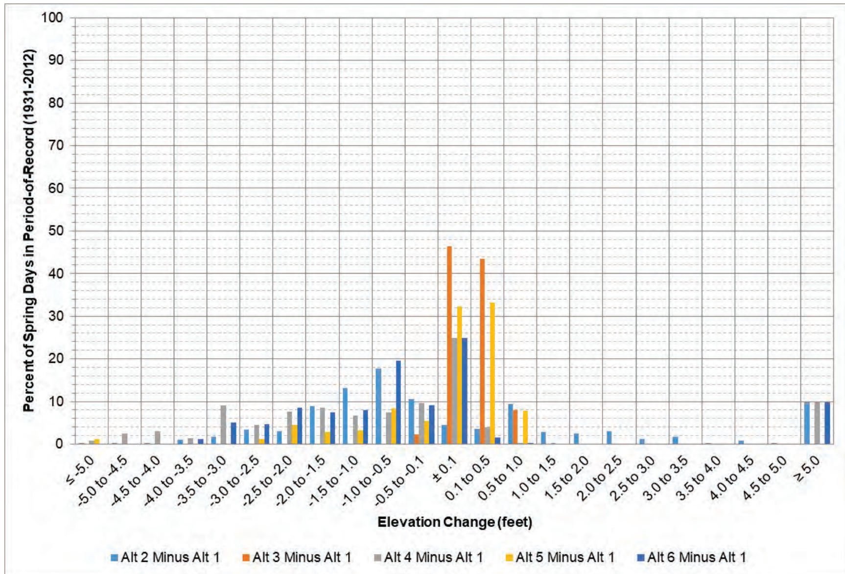
Figure 9-3: Garrison elevation change between each alternative and Alt 1 during March – April.
