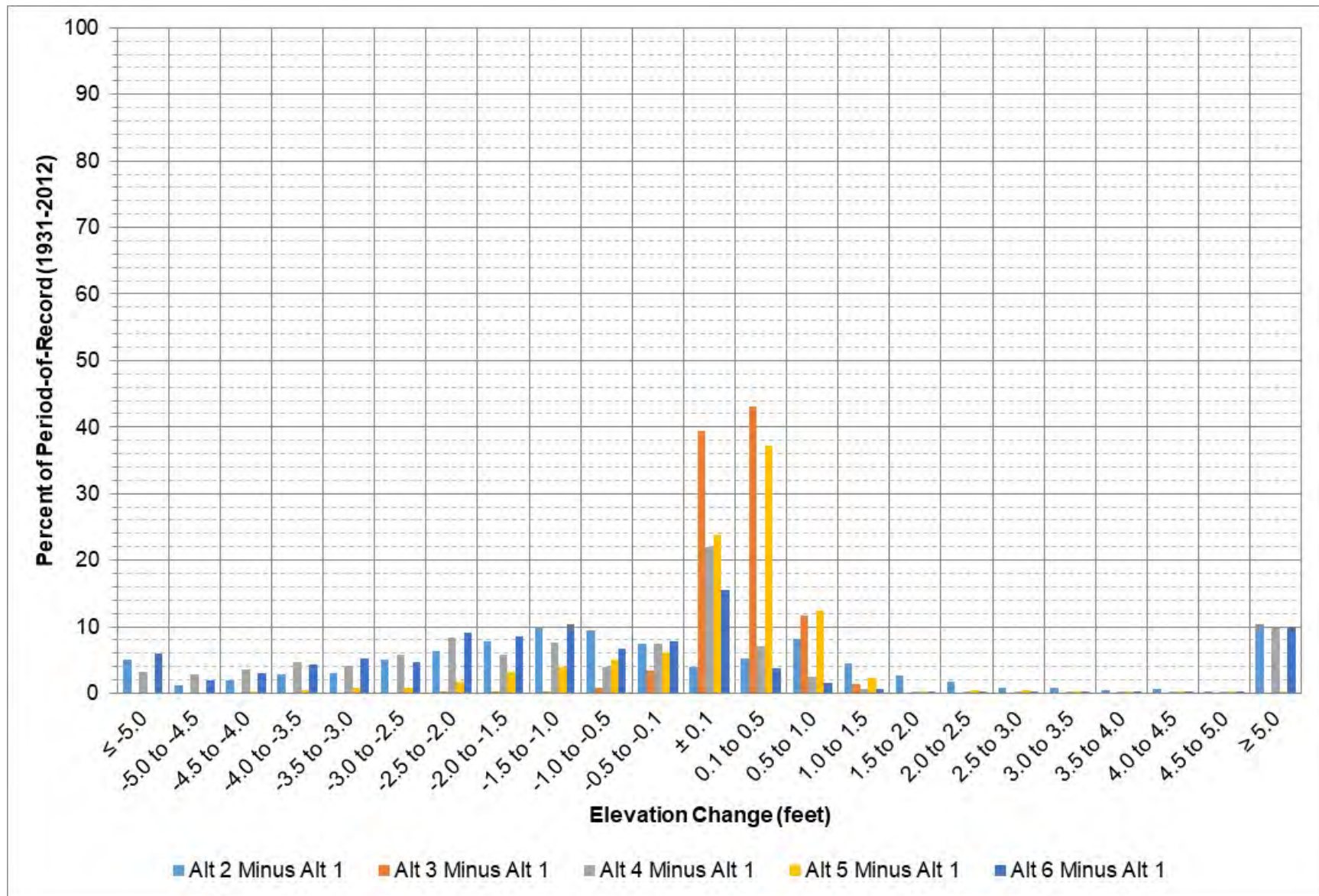
Figure 9-53: Oahe elevation change between each alternative and Alt 1 for all days in the period-of-record.
