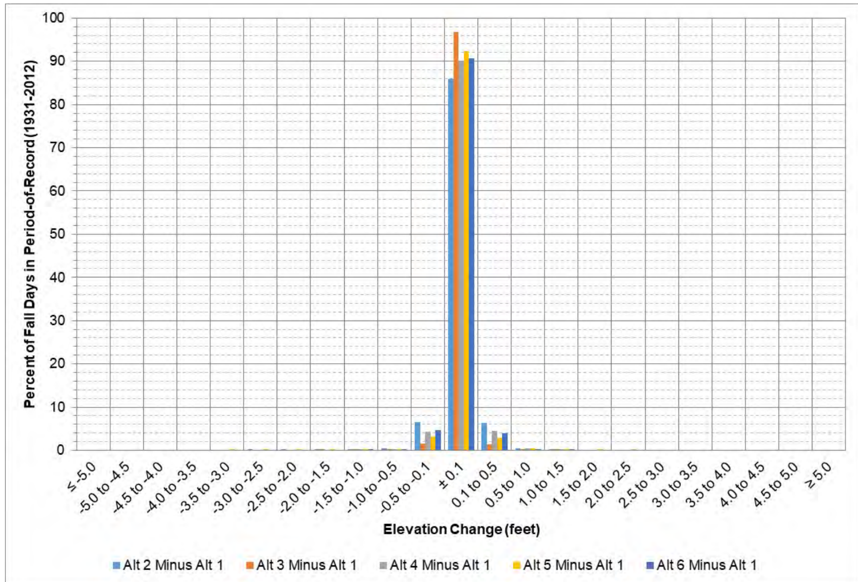
Figure 9-35: Gavins Point elevation change between each alternative and Alt 1 during September – November.
