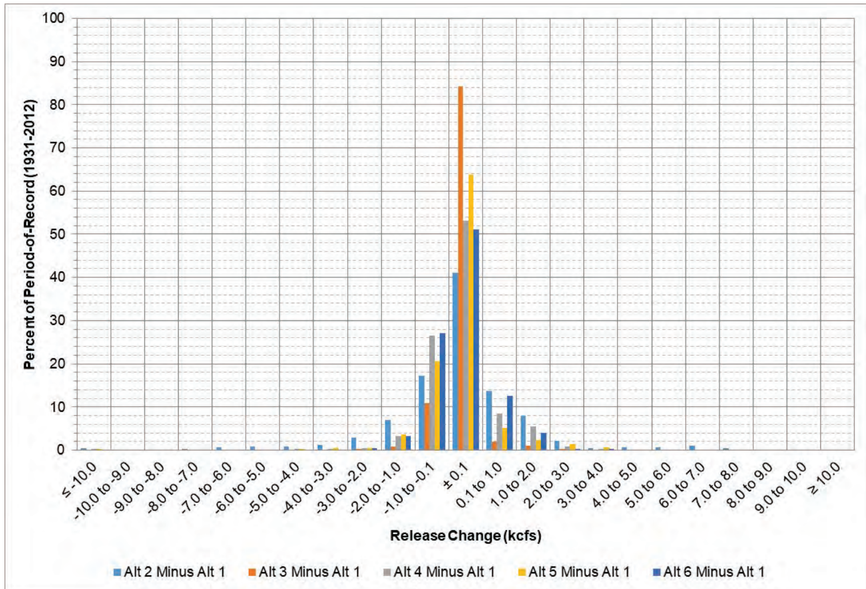
Figure 6-2: Fort Peck release change between each alternative and Alt 1 for all days in the period-of-record.
