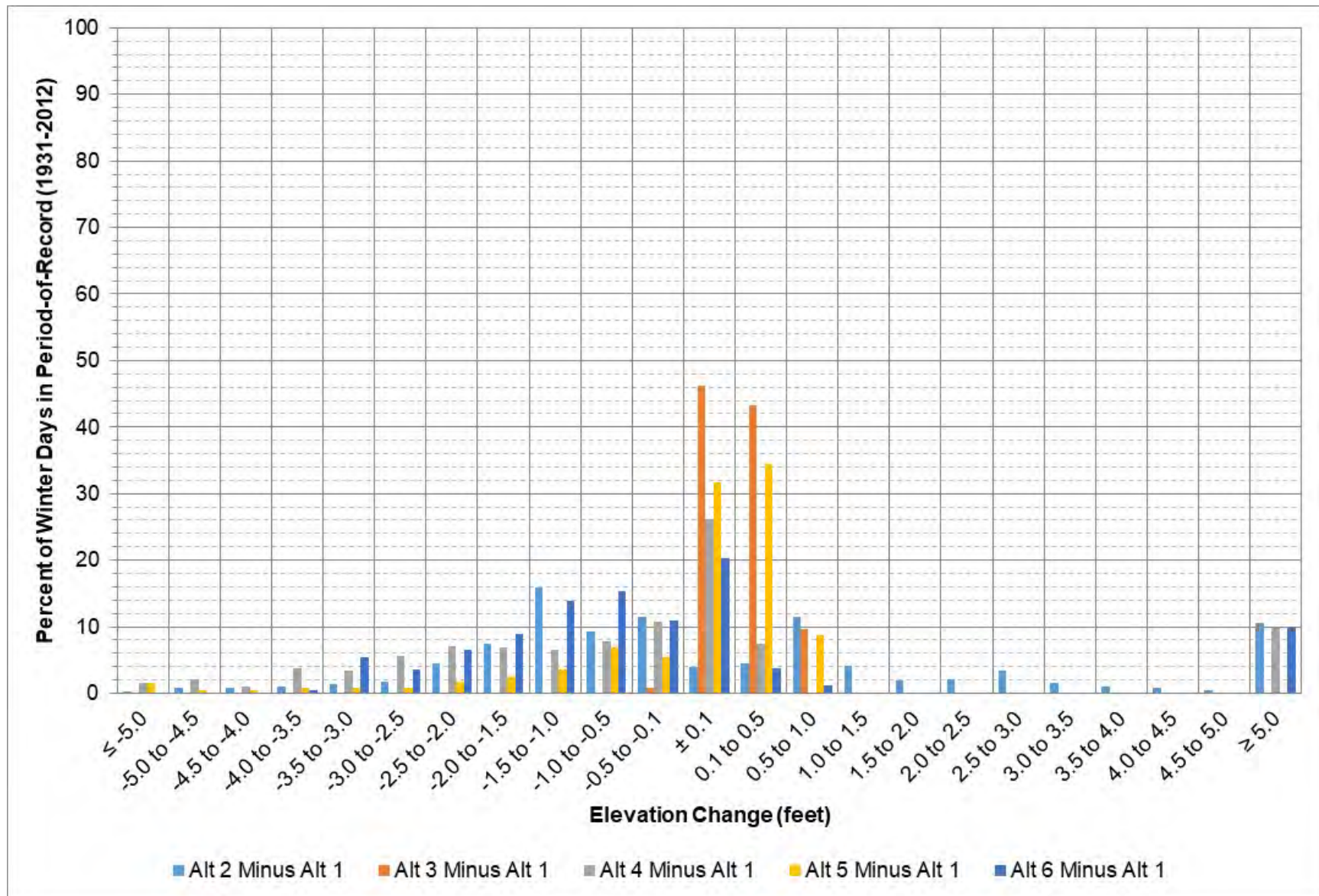
Figure 9-39: Garrison elevation change between each alternative and Alt 1 during December – February.
