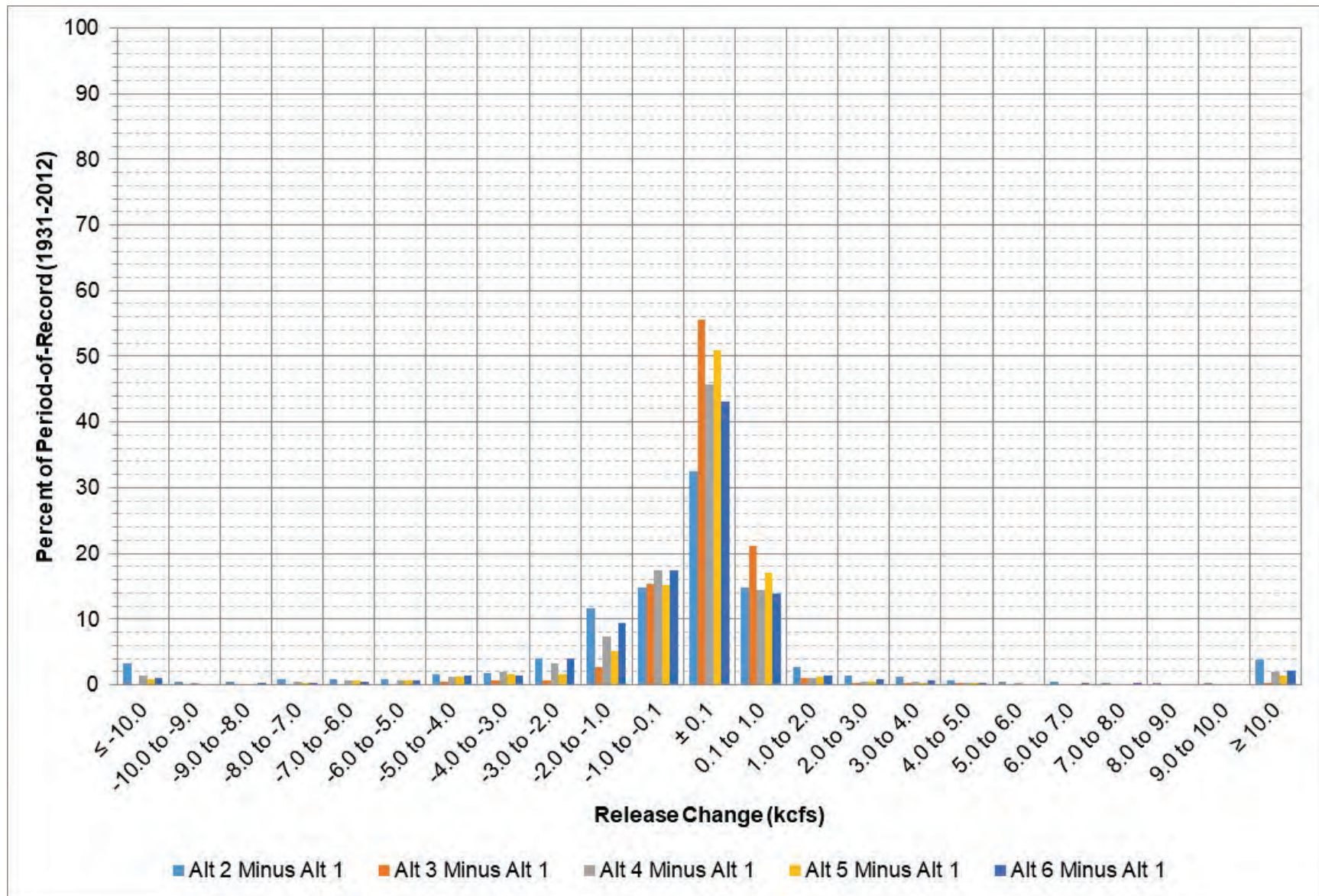
Figure 6-8: Big Bend release change between each alternative and Alt 1 for all days in the period-of-record.
