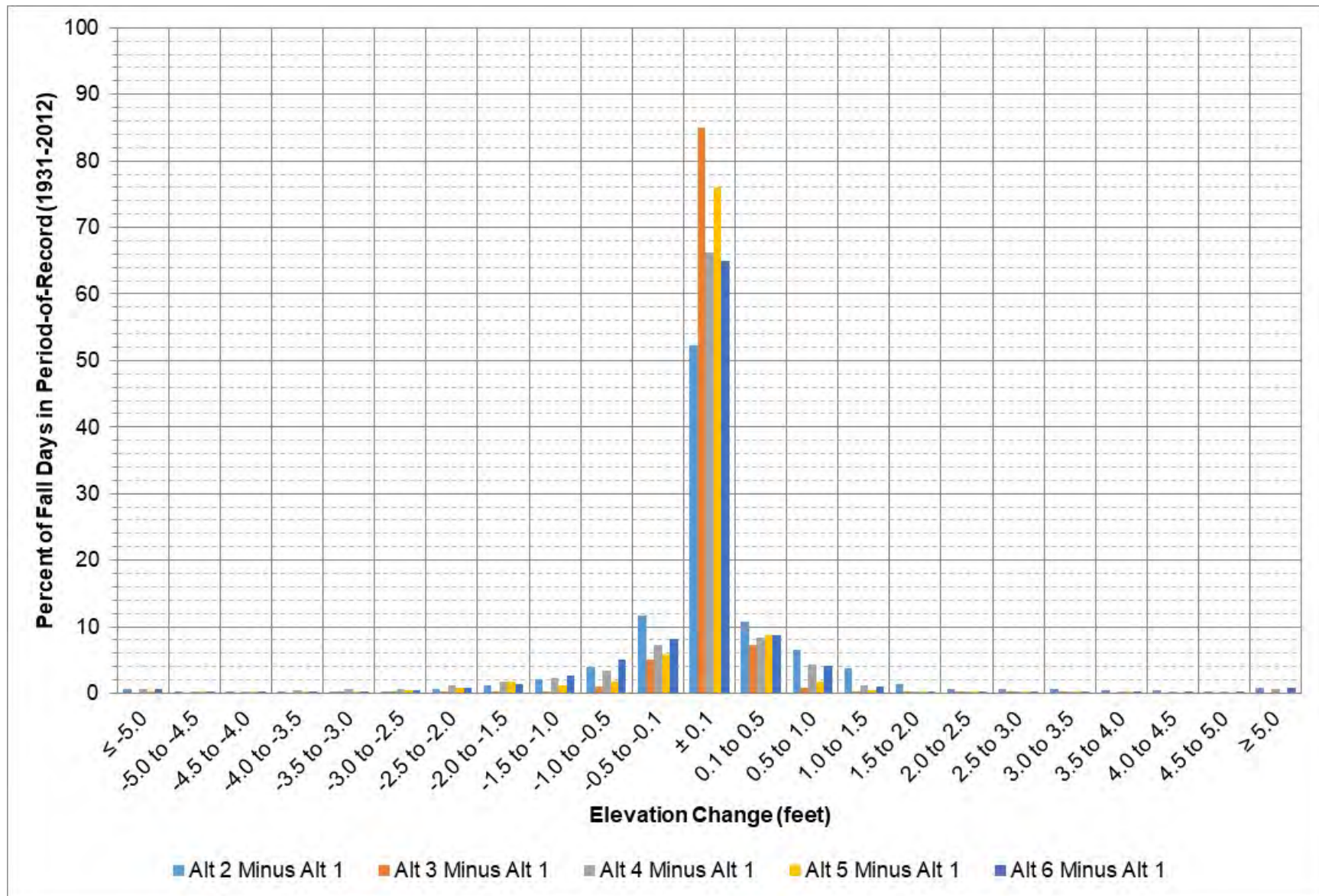
Figure 9-33: Fort Randall elevation change between each alternative and Alt 1 during September – November.
