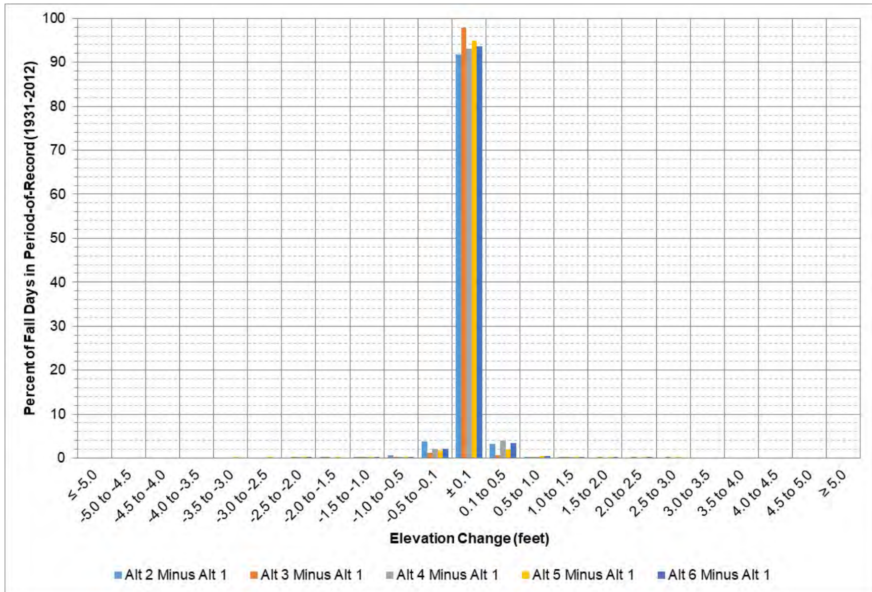
Figure 9-31: Big Bend elevation change between each alternative and Alt 1 during September – November.
