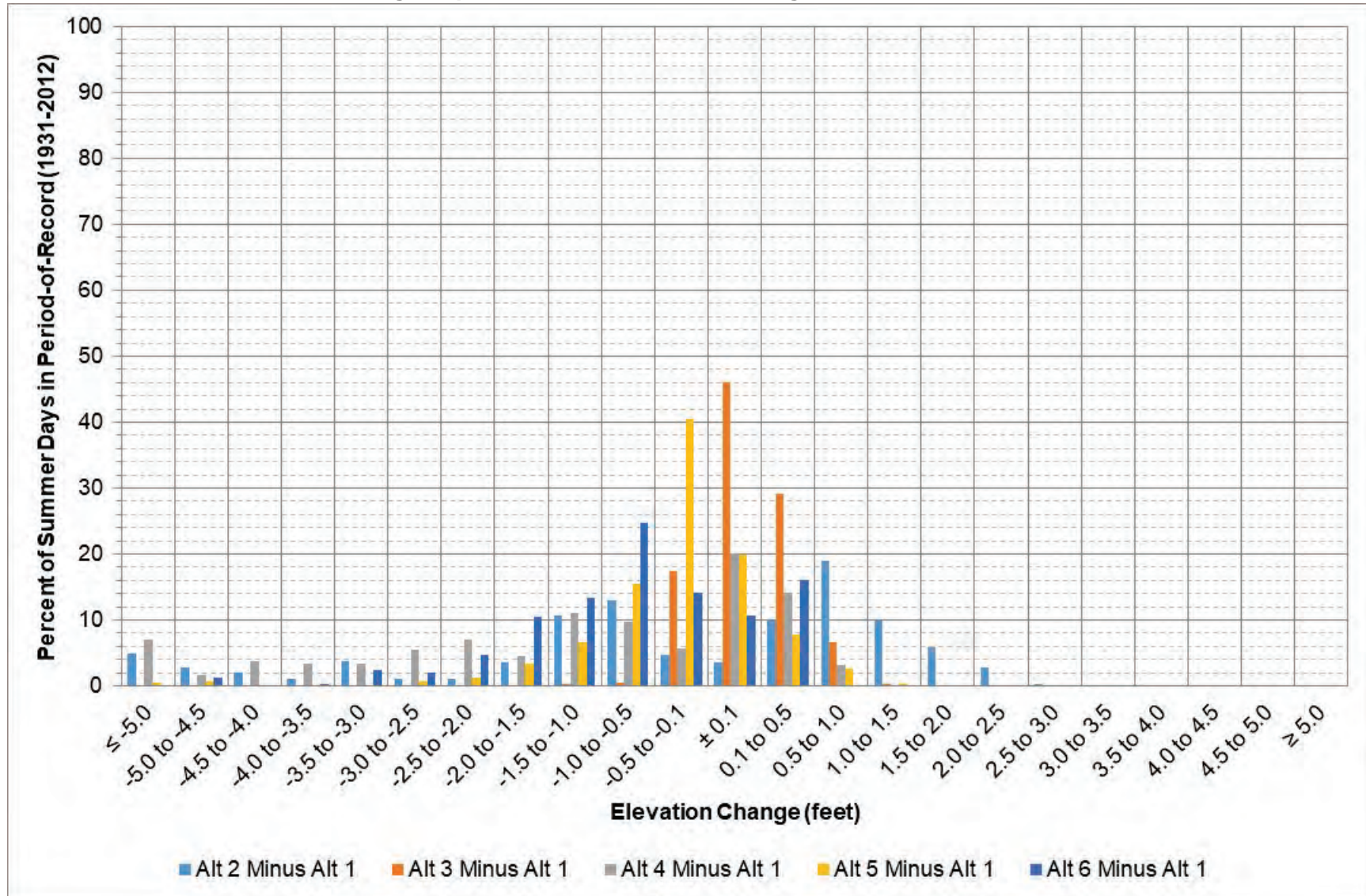
Figure 3-14: Fort Peck elevation change between each alternative and Alt 1 during May – August.
