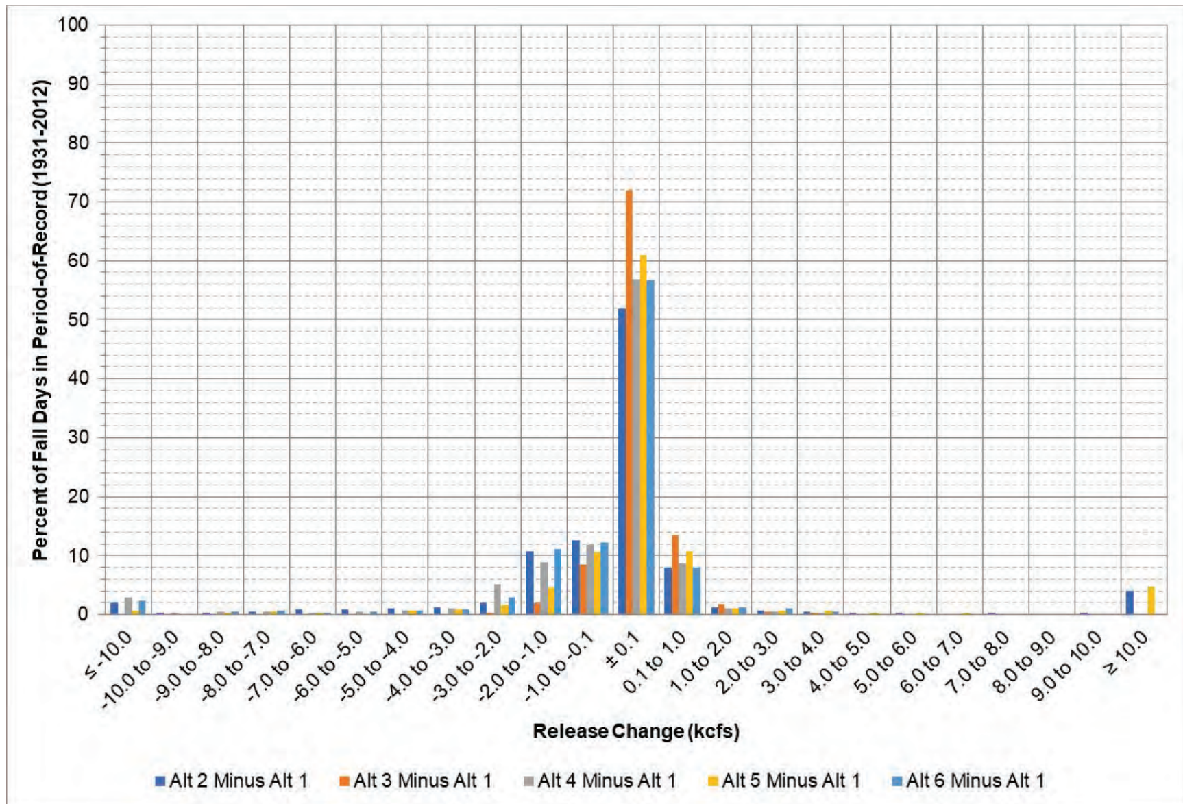
Figure 4-19: Fort Randall release change between each alternative and Alt 1 during September – November.
