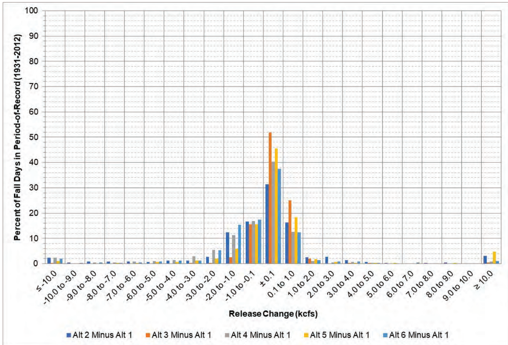
Figure 4-17: Big Bend release change between each alternative and Alt 1 during September – November.
