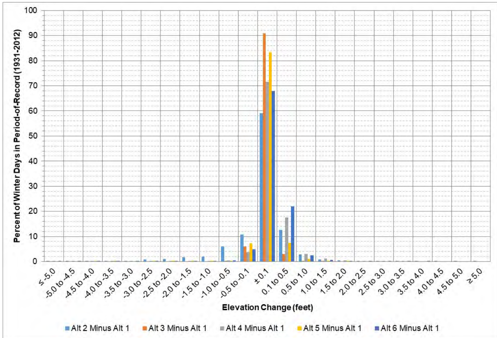
Figure 9-45: Fort Randall elevation change between each alternative and Alt 1 during December – February.
