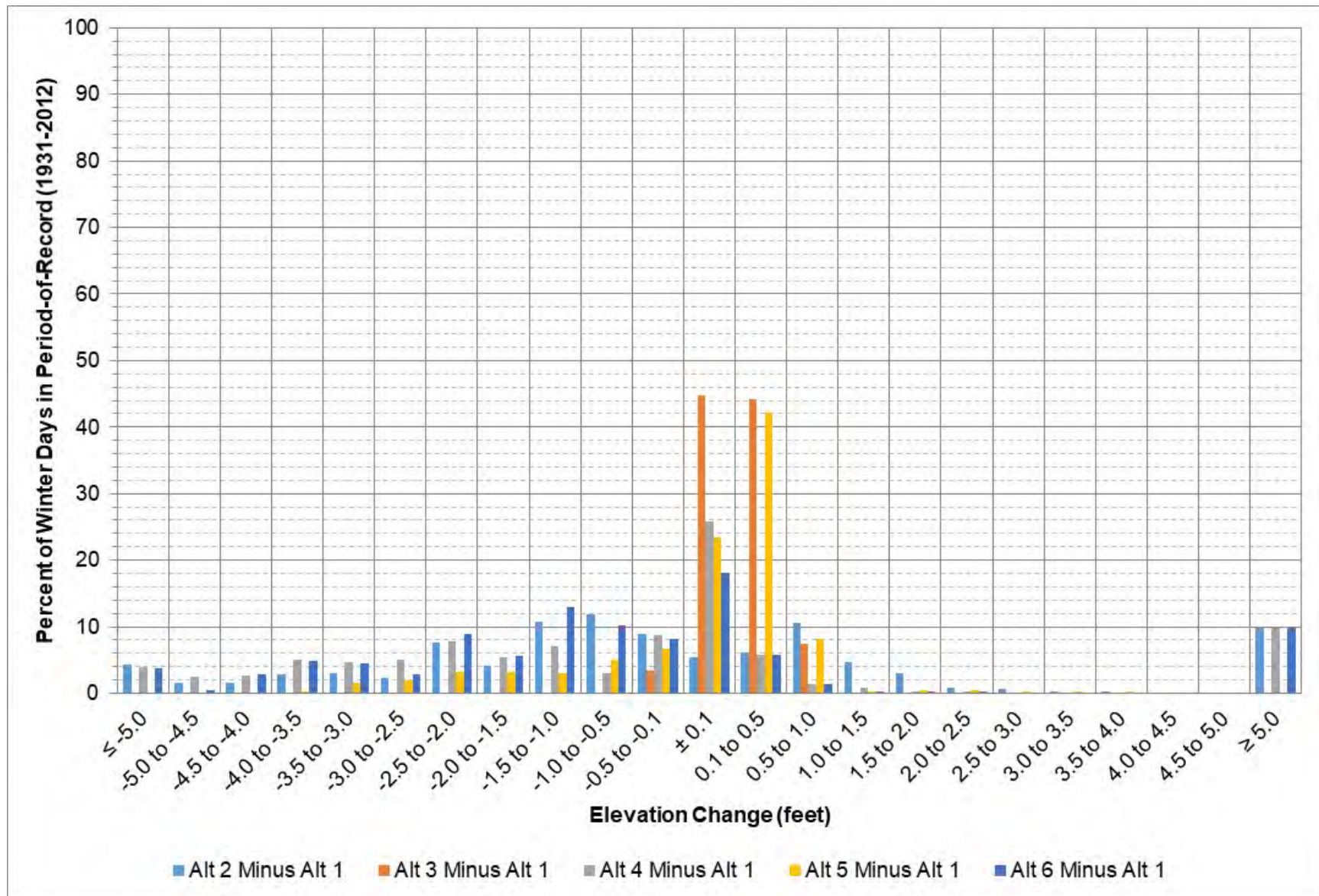
Figure 9-41: Oahe elevation change between each alternative and Alt 1 during December – February.
