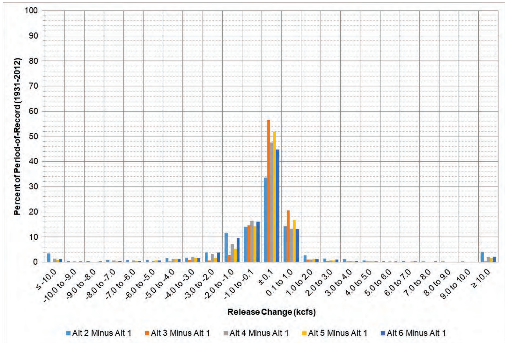
Figure 6-6: Oahe release change between each alternative and Alt 1 for all days in the period-of-record.
