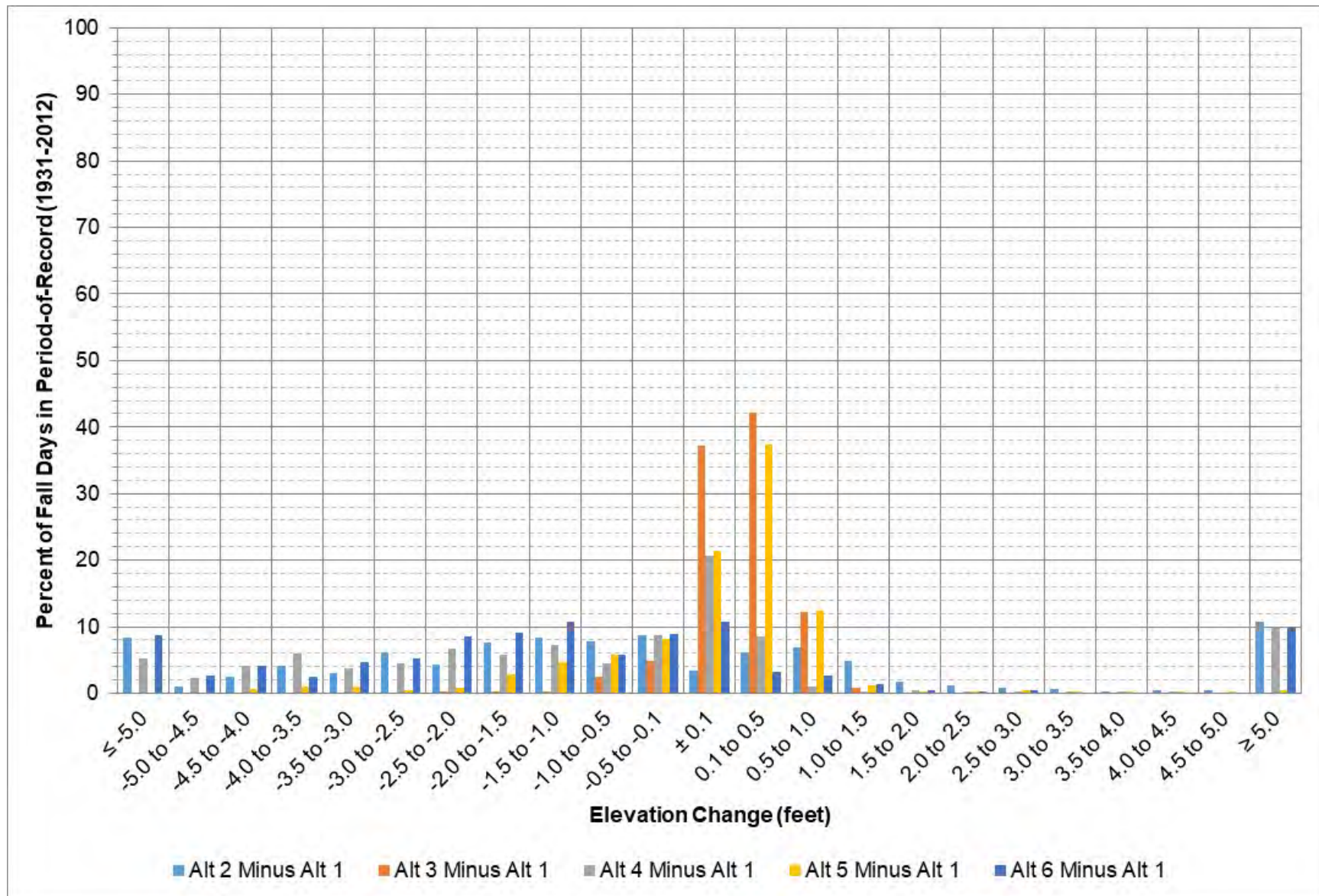
Figure 9-29: Oahe elevation change between each alternative and Alt 1 during September – November.
