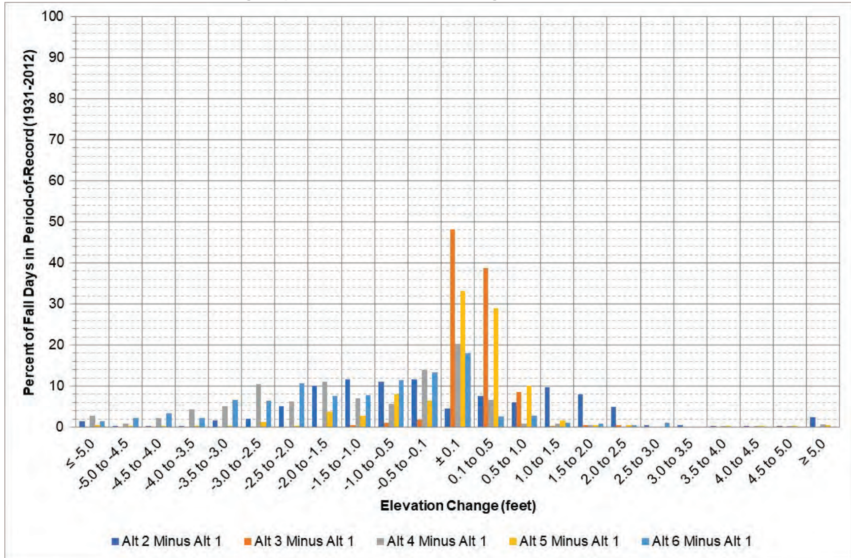
Figure 4-10: Fort Peck elevation change between each alternative and Alt 1 during September – November.
