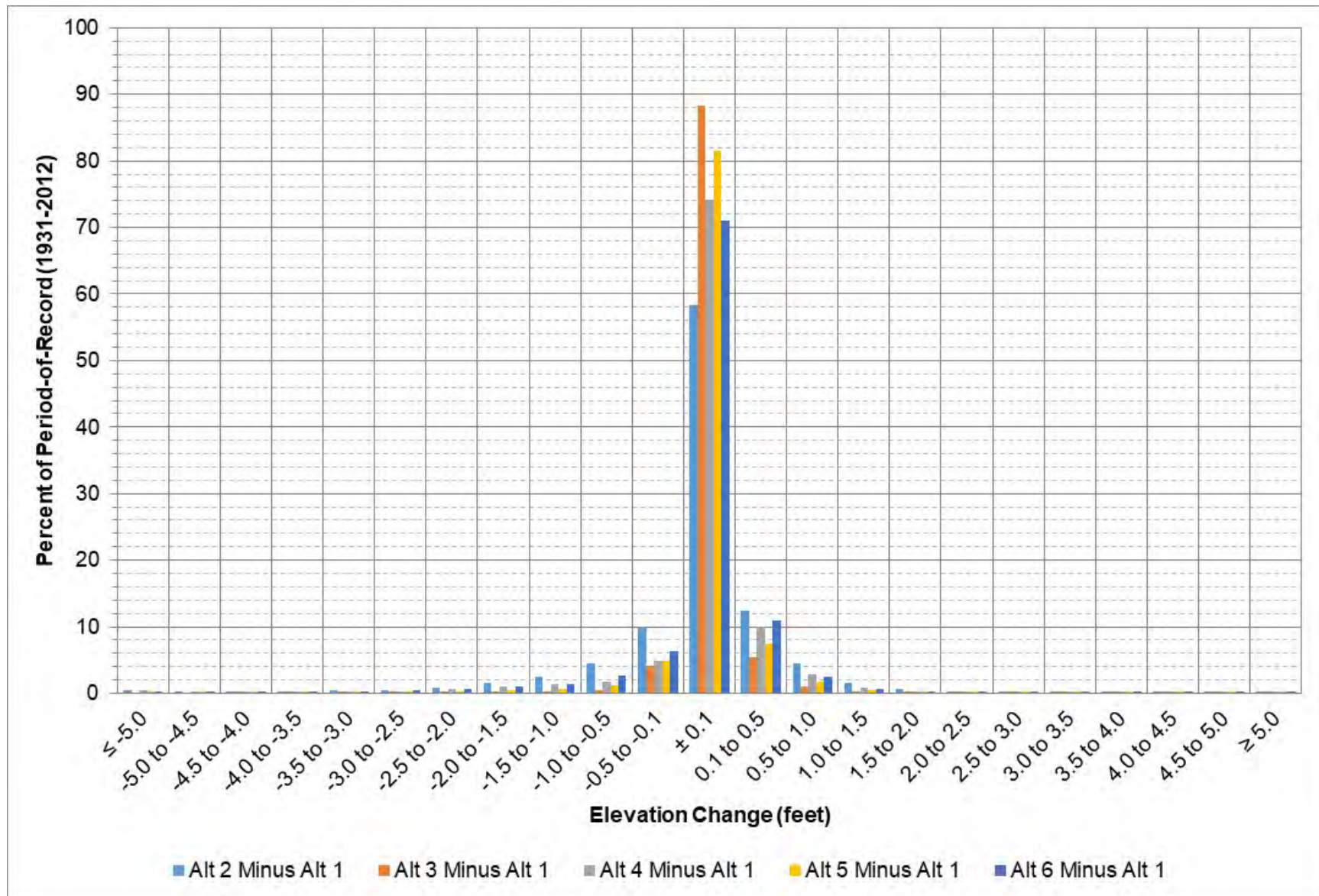
Figure 9-57: Fort Randall elevation change between each alternative and Alt 1 for all days in the period-of-record.
