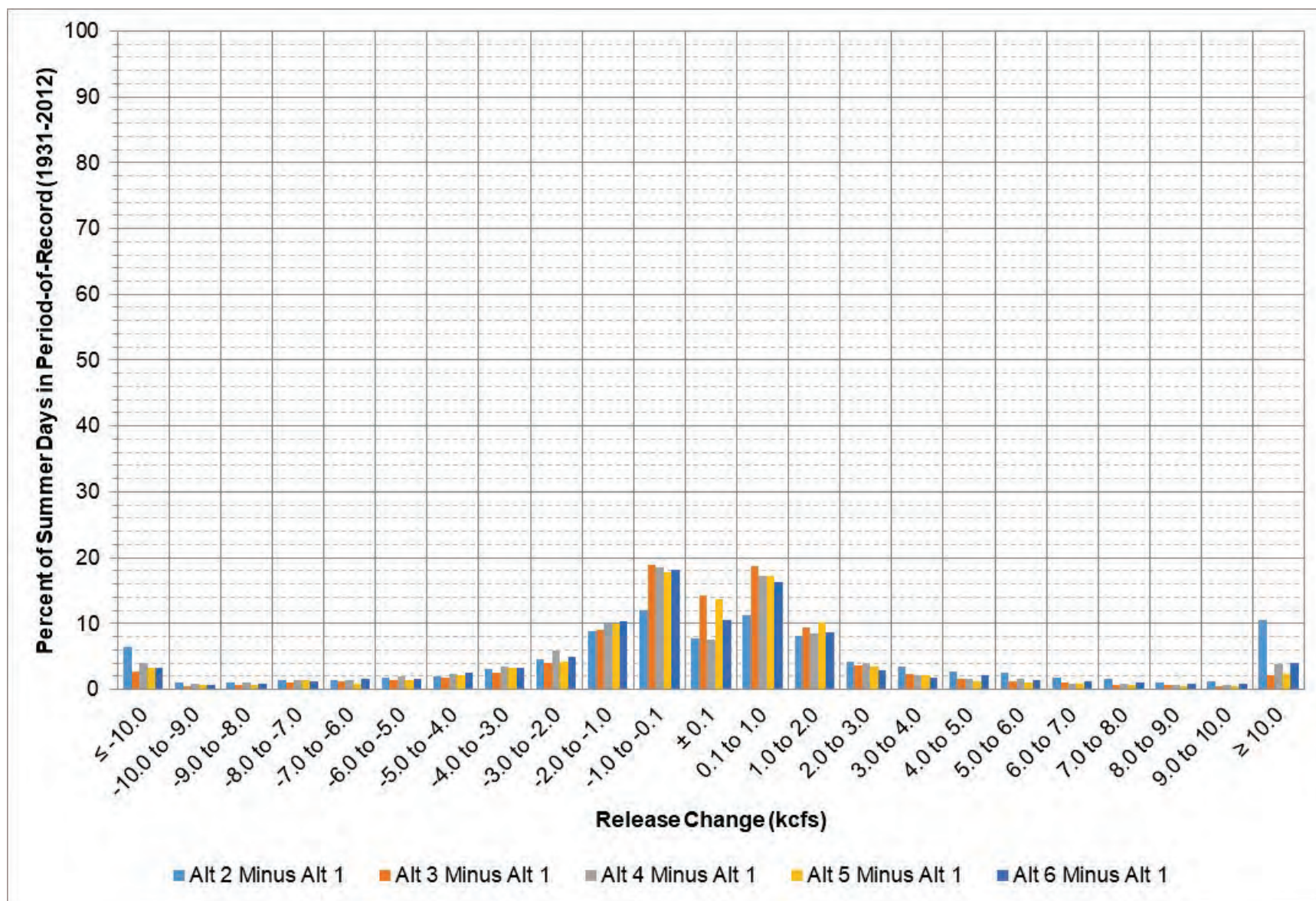
Figure 3-23: Fort Randall release change between each alternative and Alt 1 during May – August.
