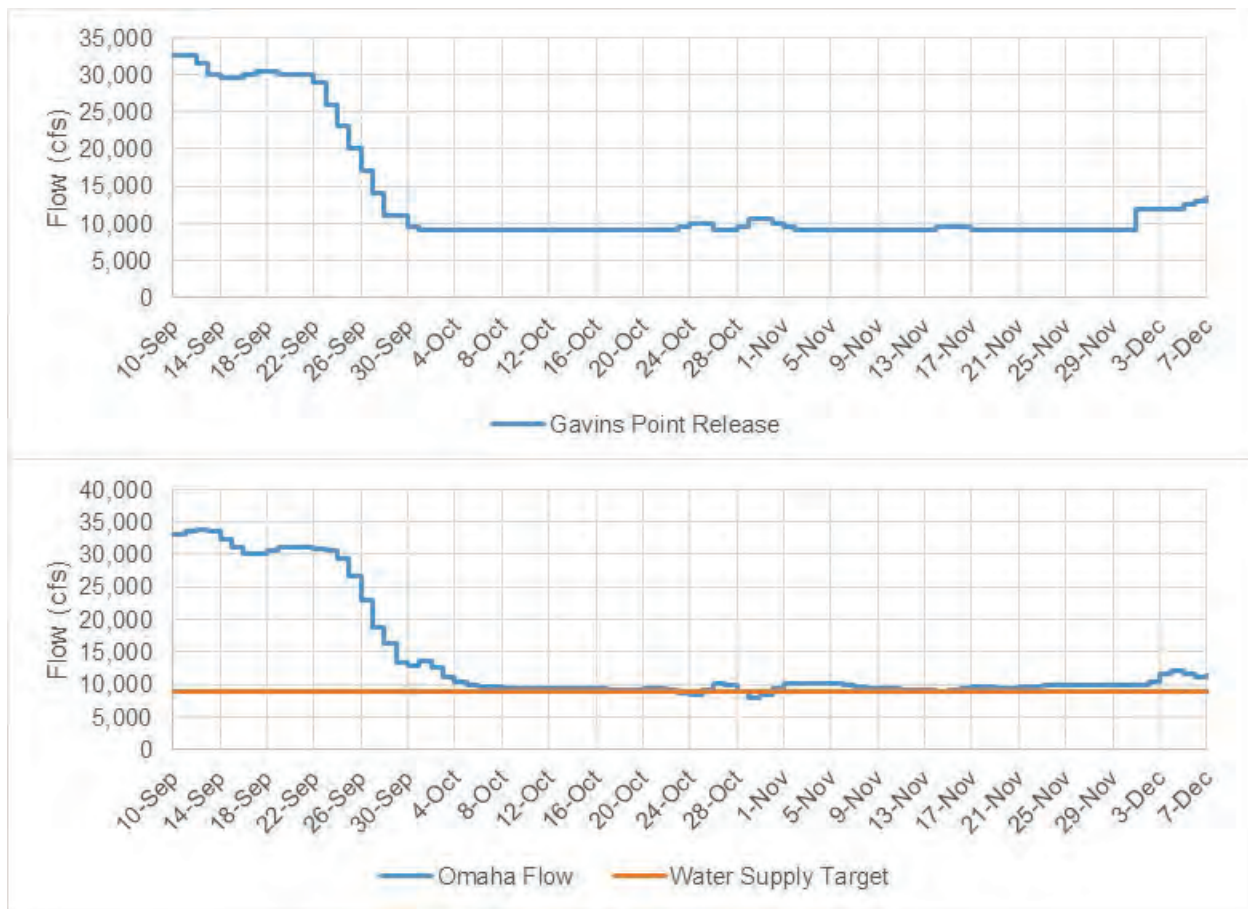
Figure 4-1: Fall water supply operations.
