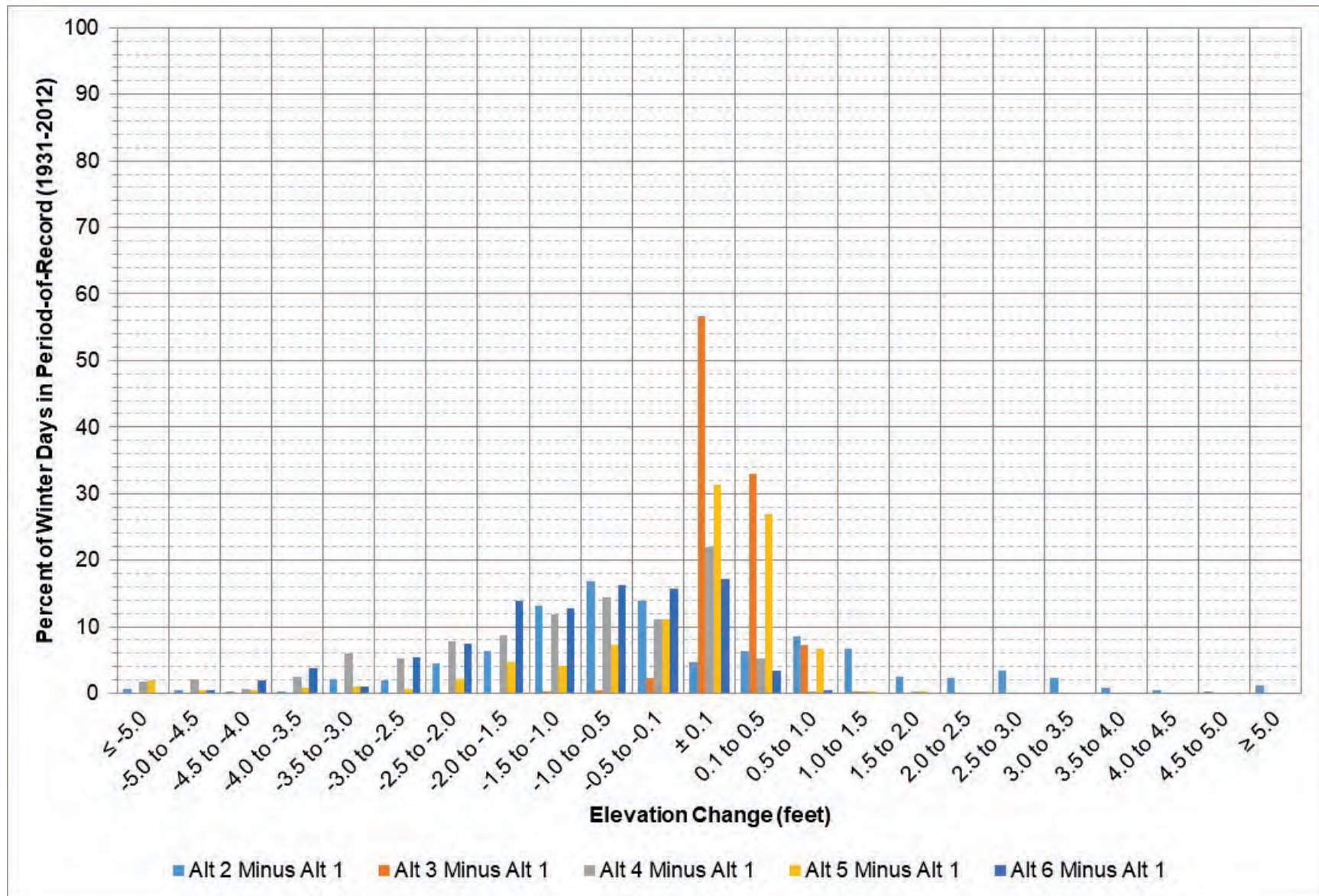
Figure 5-8: Garrison elevation change between each alternative and Alt 1 during December – February.
