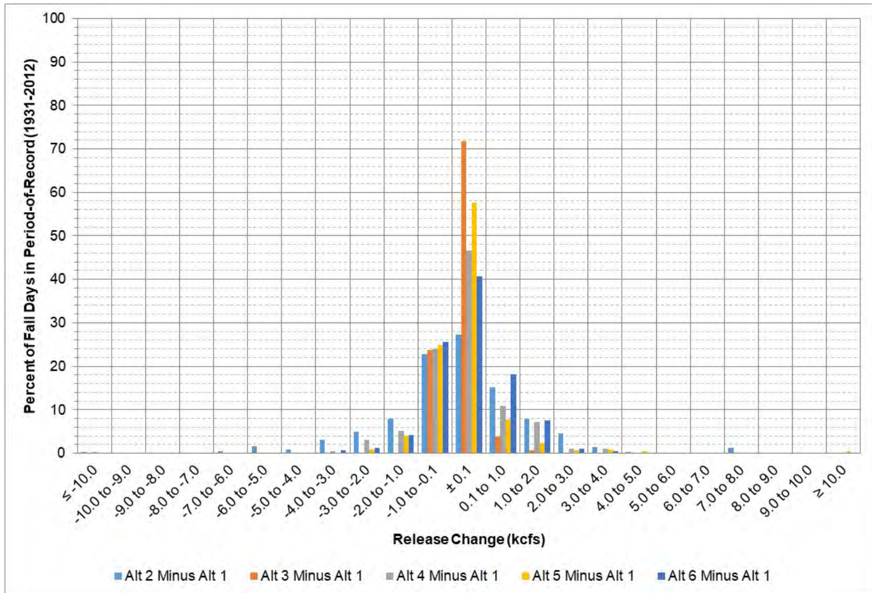
Figure 9-26: Fort Peck release change between each alternative and Alt 1 during September – November.
