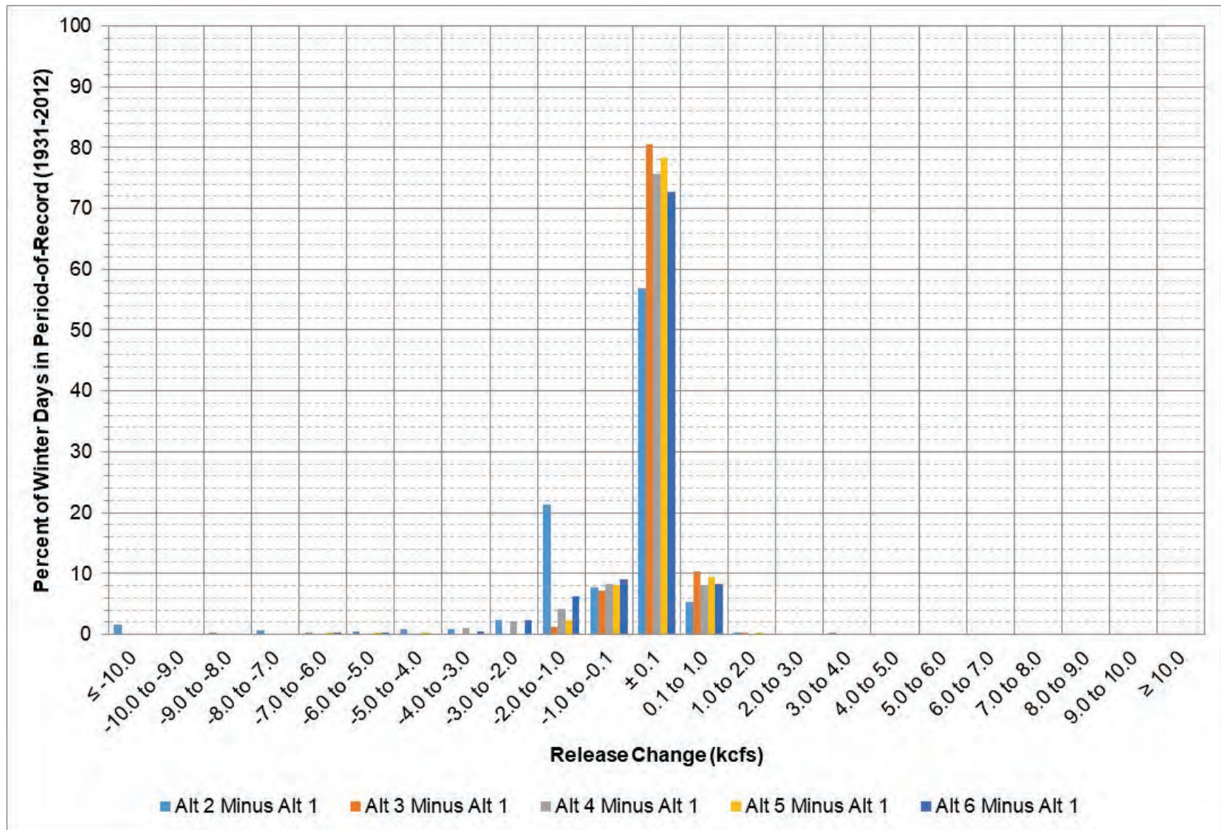
Figure 5-15: Fort Randall release change between each alternative and Alt 1 during December – February.
