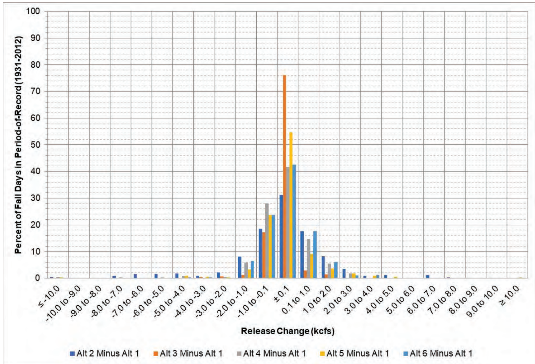
Figure 4-11: Fort Peck release change between each alternative and Alt 1 during September – November.
