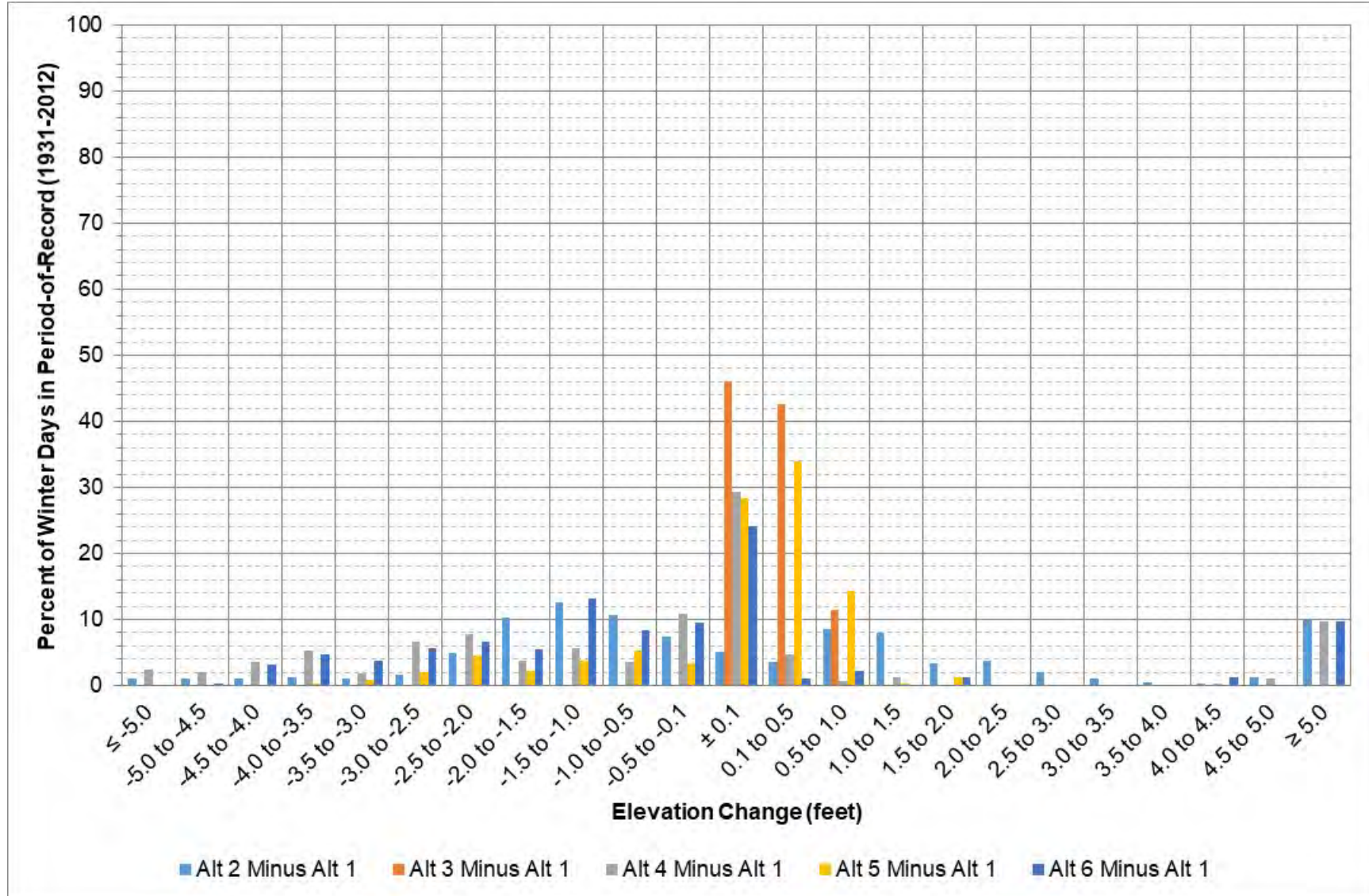
Figure 9-37: Fort Peck elevation change between each alternative and Alt 1 during December – February.
