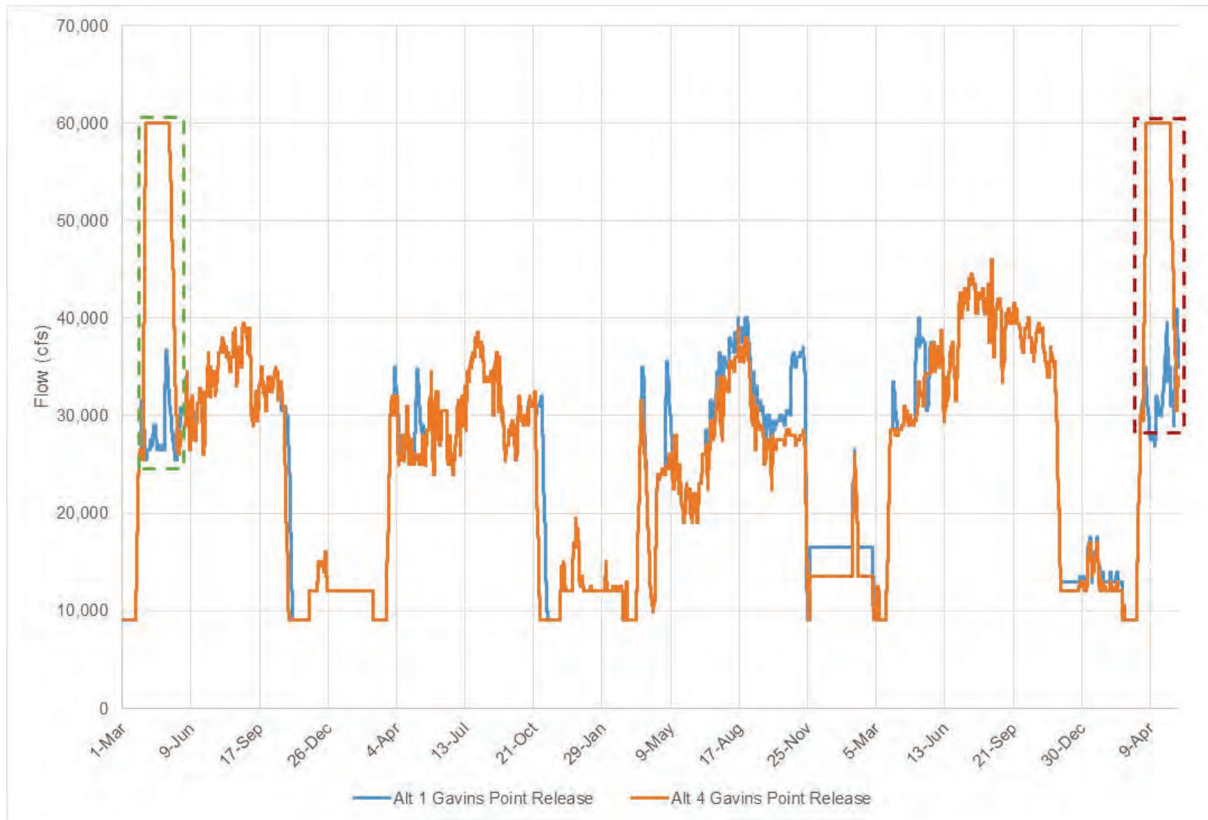
Figure 2-8: Comparison of Alt 1 vs Alt 4 Gavins Point releases during a five year period with ESH-creating release operations.
