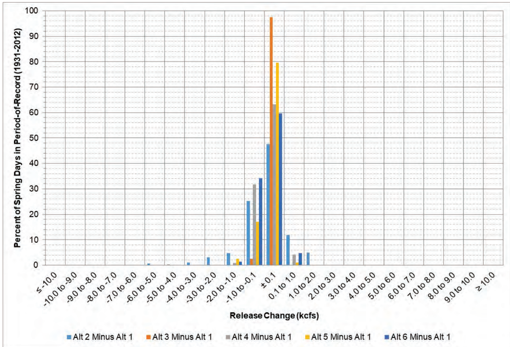
Figure 2-18: Fort Peck release change between each alternative and Alt 1 during March – April.
