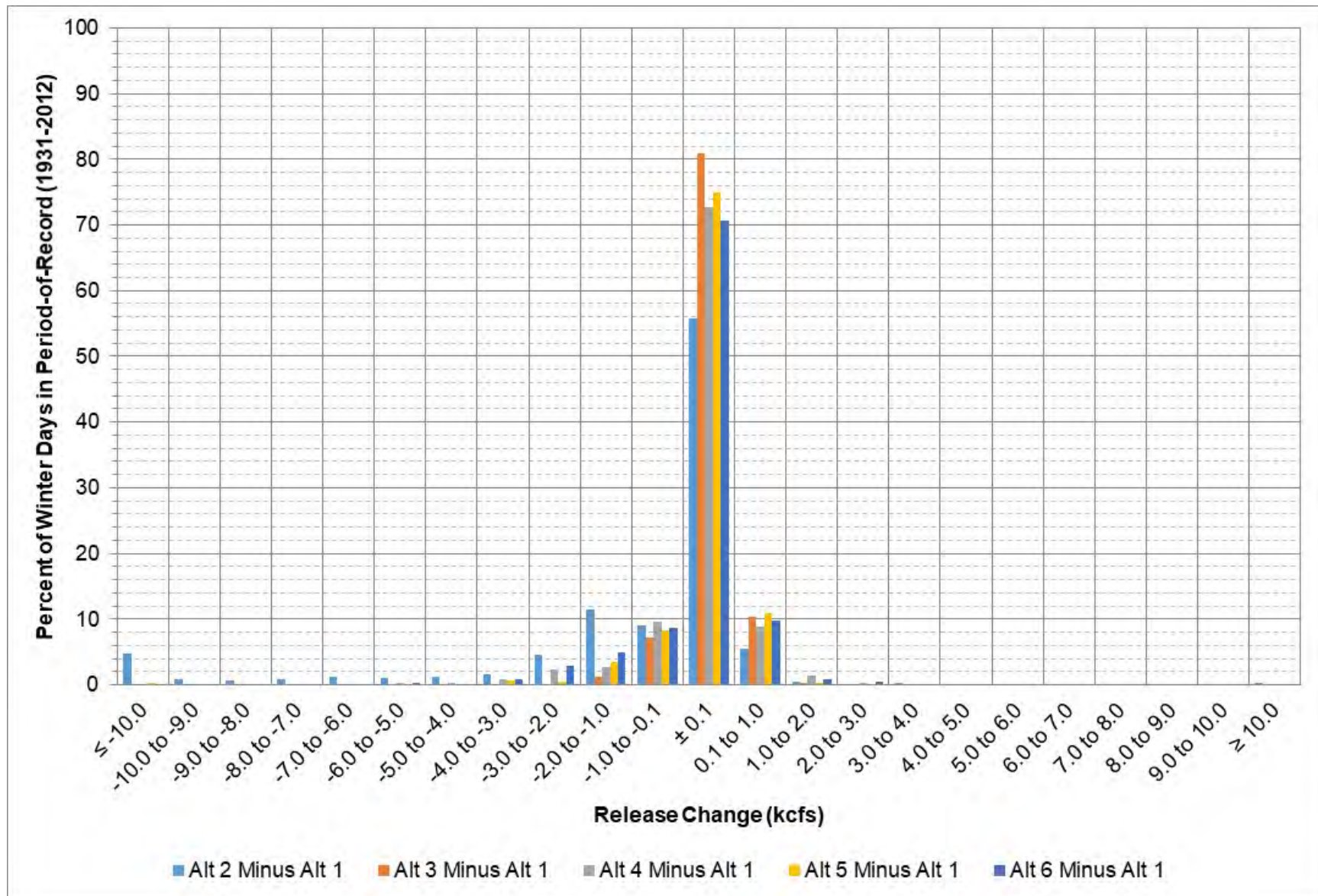
Figure 9-46: Fort Randall release change between each alternative and Alt 1 during December – February.
