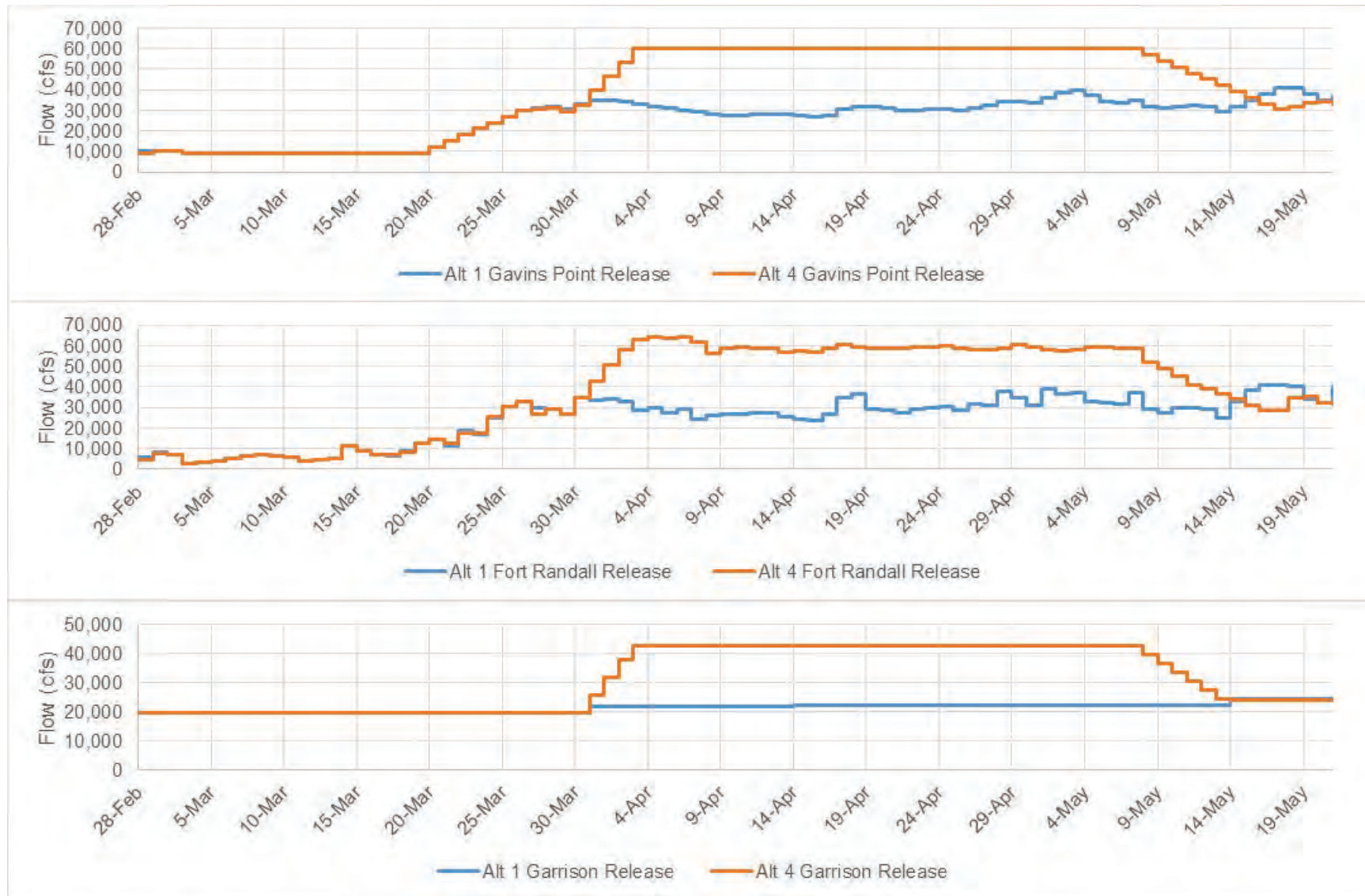
Figure 2-16: Comparison of Alt 1 vs Alt 4 Gavins Point, Fort Randall, and Garrison's releases during the ESH-creating release shown in Figure 2-14.
