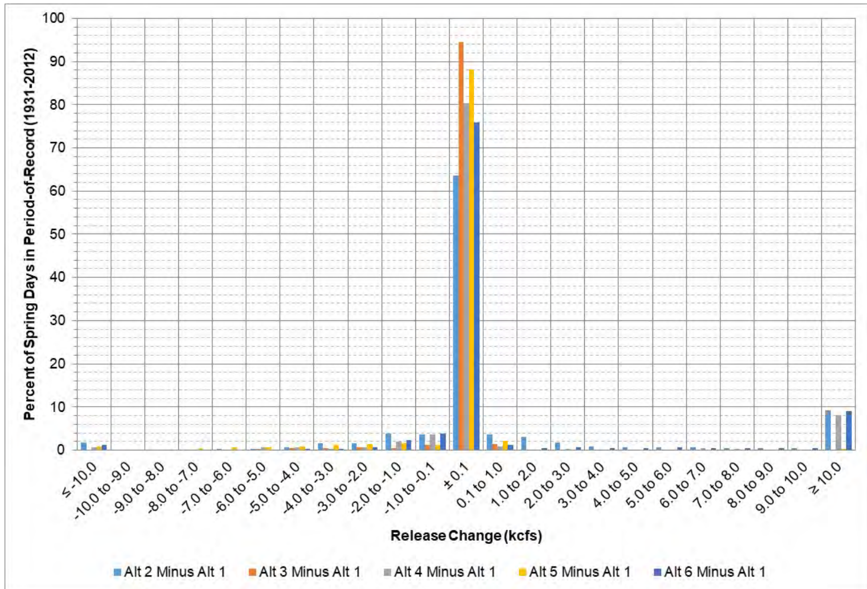
Figure 9-12: Gavins Point release change between each alternative and Alt 1 during March – April.
