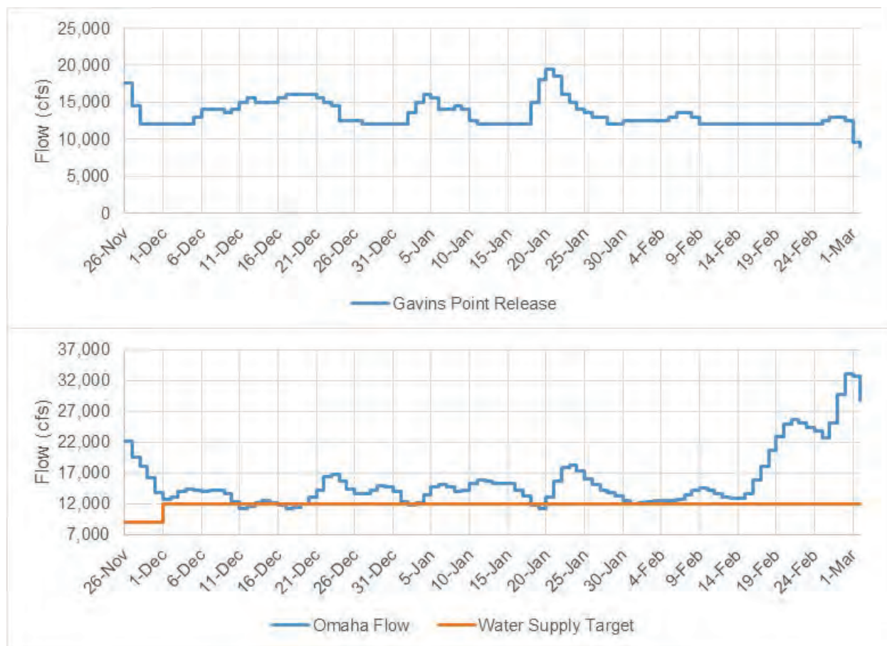
Figure 5-2: Low winter releases from Gavins Point Dam.
