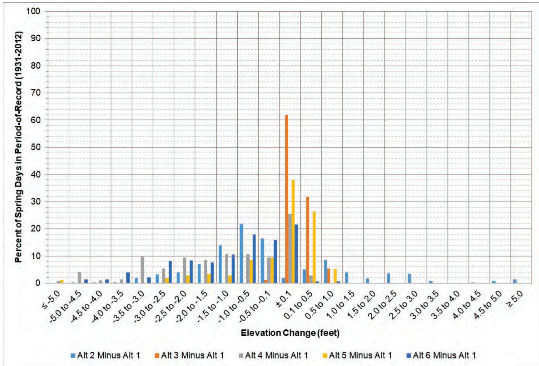
Figure 2-19: Garrison elevation change between each alternative and Alt 1 during March – April.
