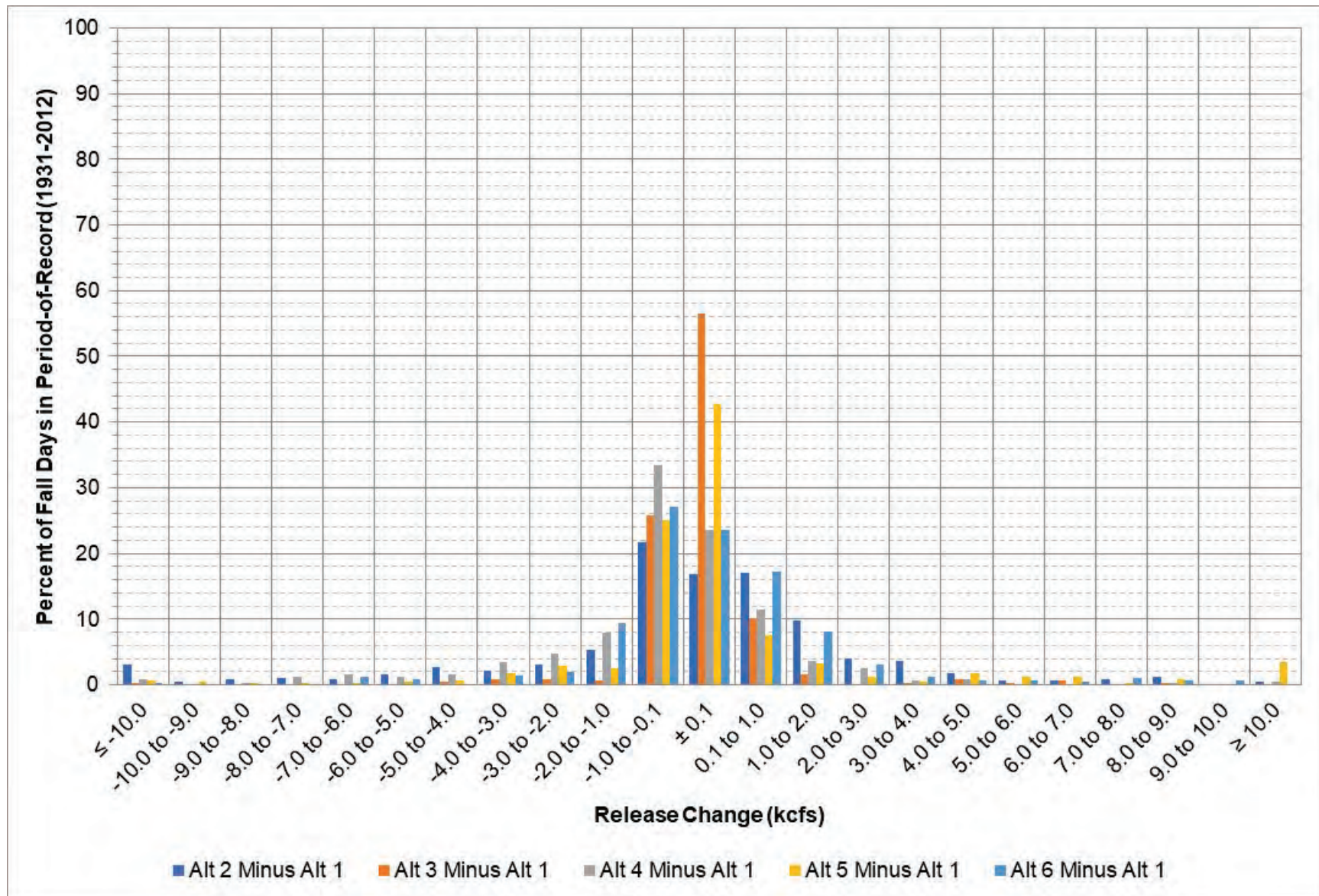
Figure 4-13: Garrison release change between each alternative and Alt 1 during September – November.
