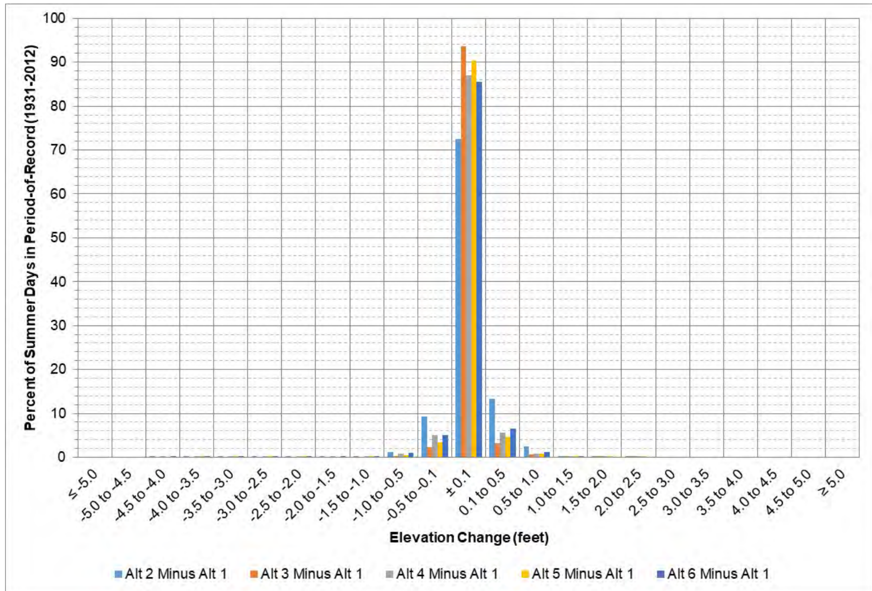
Figure 9-23: Gavins Point elevation change between each alternative and Alt 1 during May – August.
