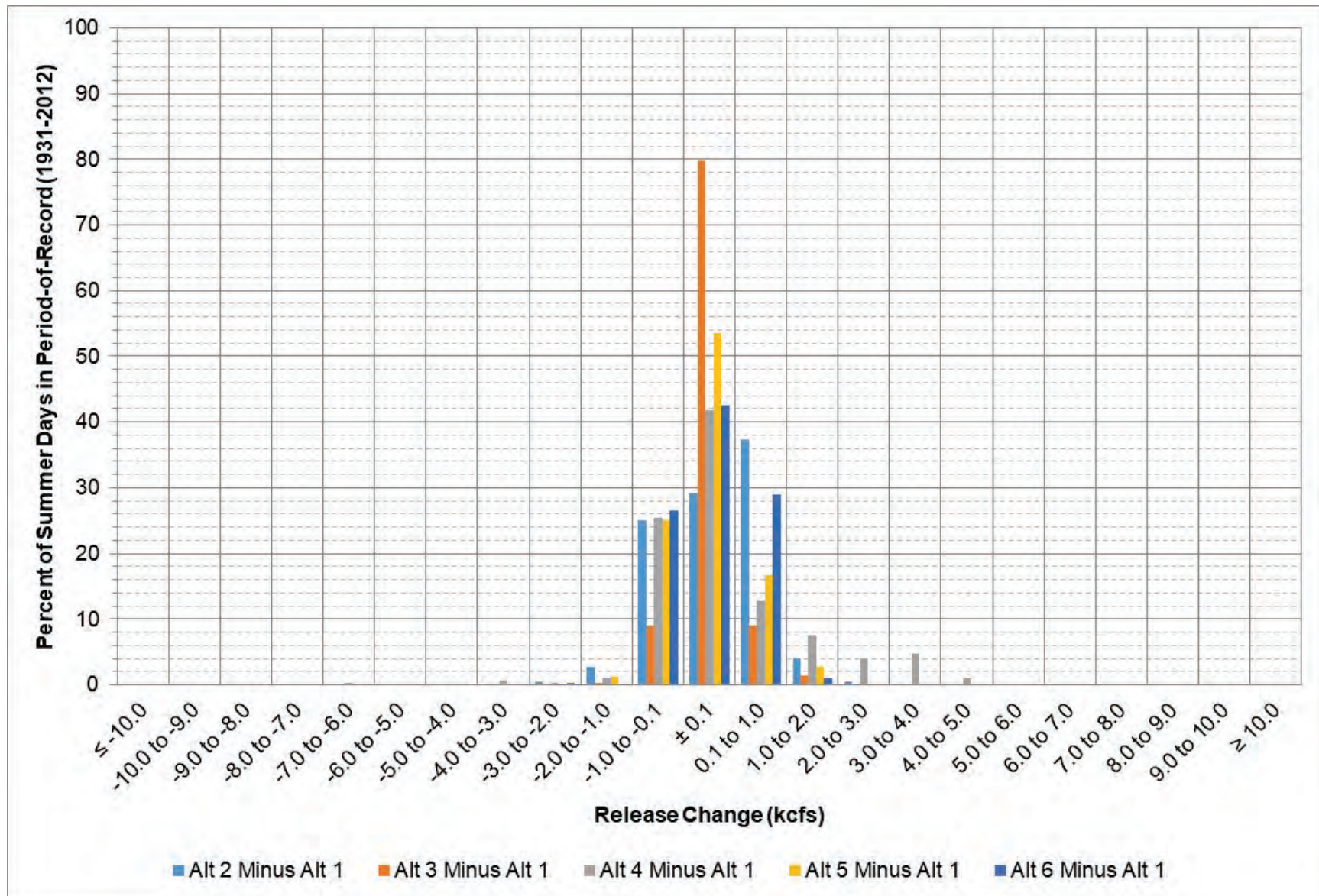
Figure 3-15: Fort Peck release change between each alternative and Alt 1 during May – August.
