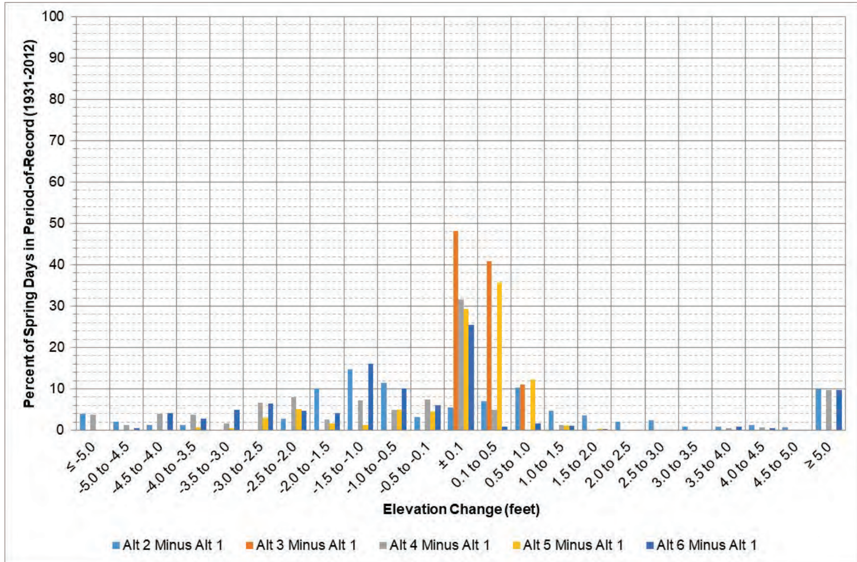
Figure 9-1: Fort Peck elevation change between each alternative and Alt 1 during March – April.
