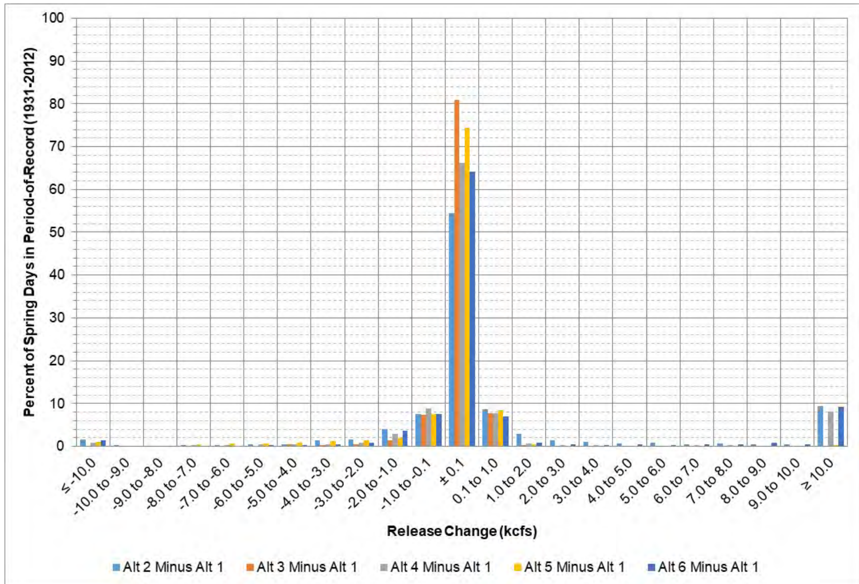
Figure 9-10: Fort Randall release change between each alternative and Alt 1 during March – April.
