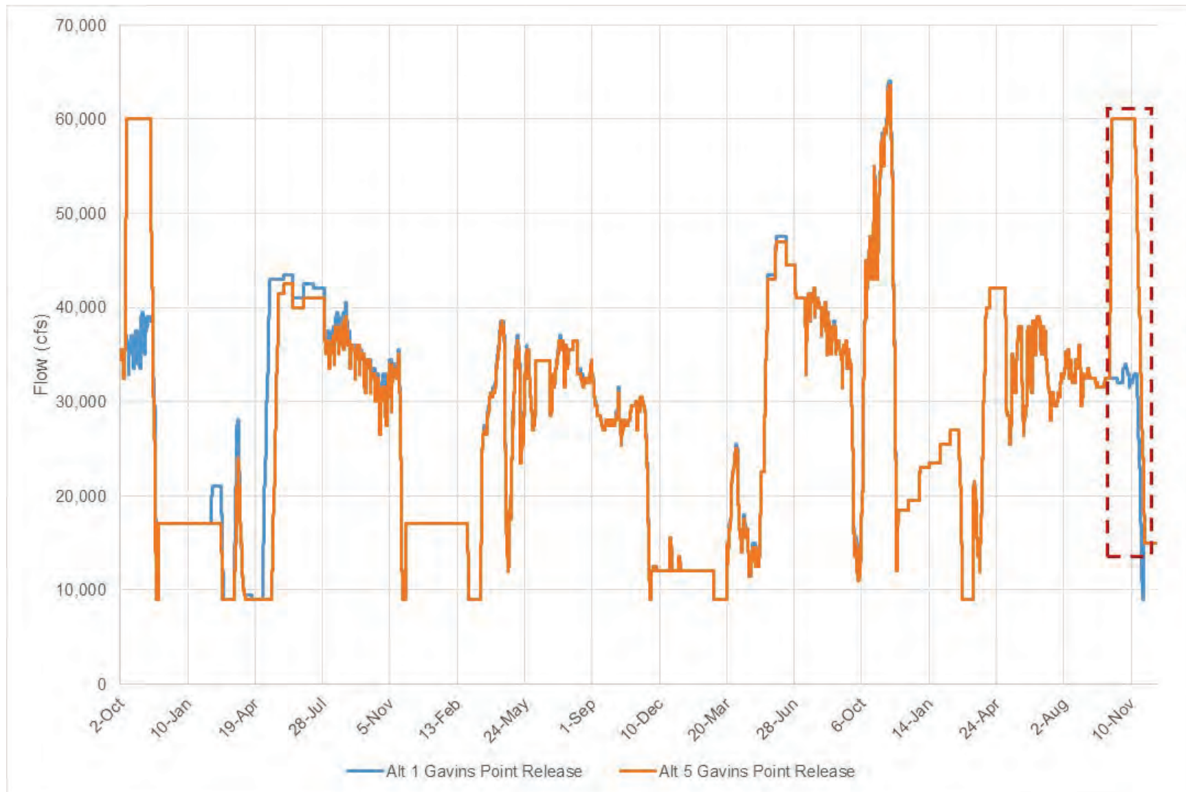
Figure 4-3: Comparison of Alt 1 vs Alt 5 Gavins Point releases during a five year period with ESH-creating release operations.
