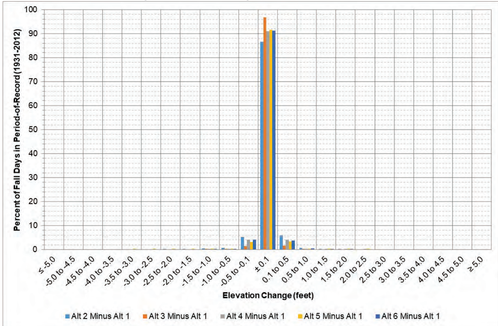
Figure 4-5: Gavins Point elevation change between each alternative and Alt 1 during September – November.
