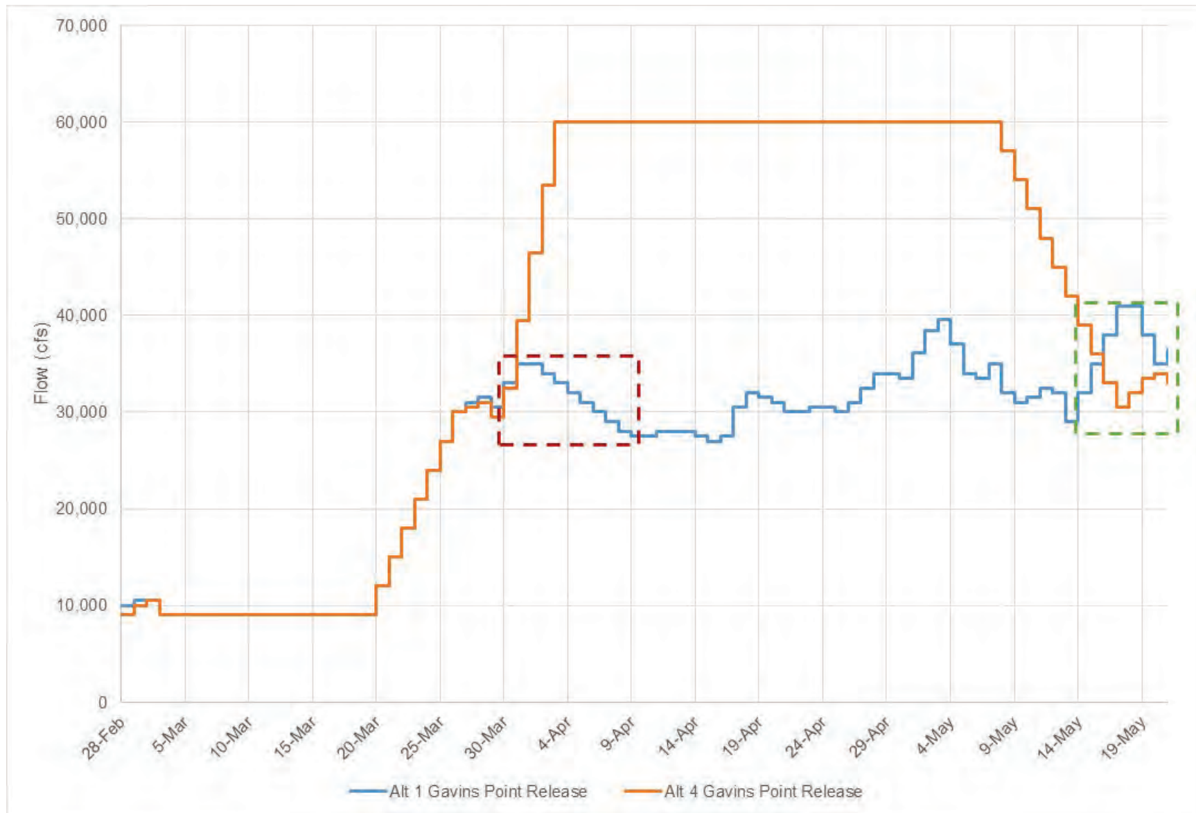
Figure 2-9: Comparison of Alt 1 vs Alt 4 Gavins Point releases during the ESH-creating release shown in Figure 2-8.
