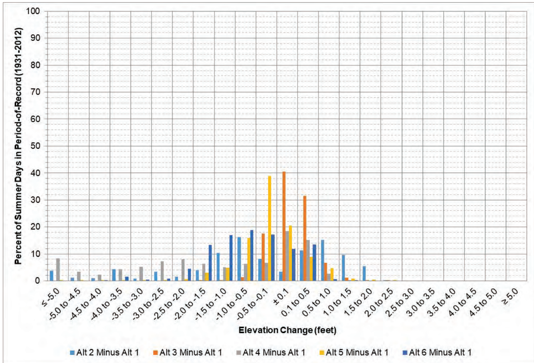
Figure 3-16: Garrison elevation change between each alternative and Alt 1 during May – August.
