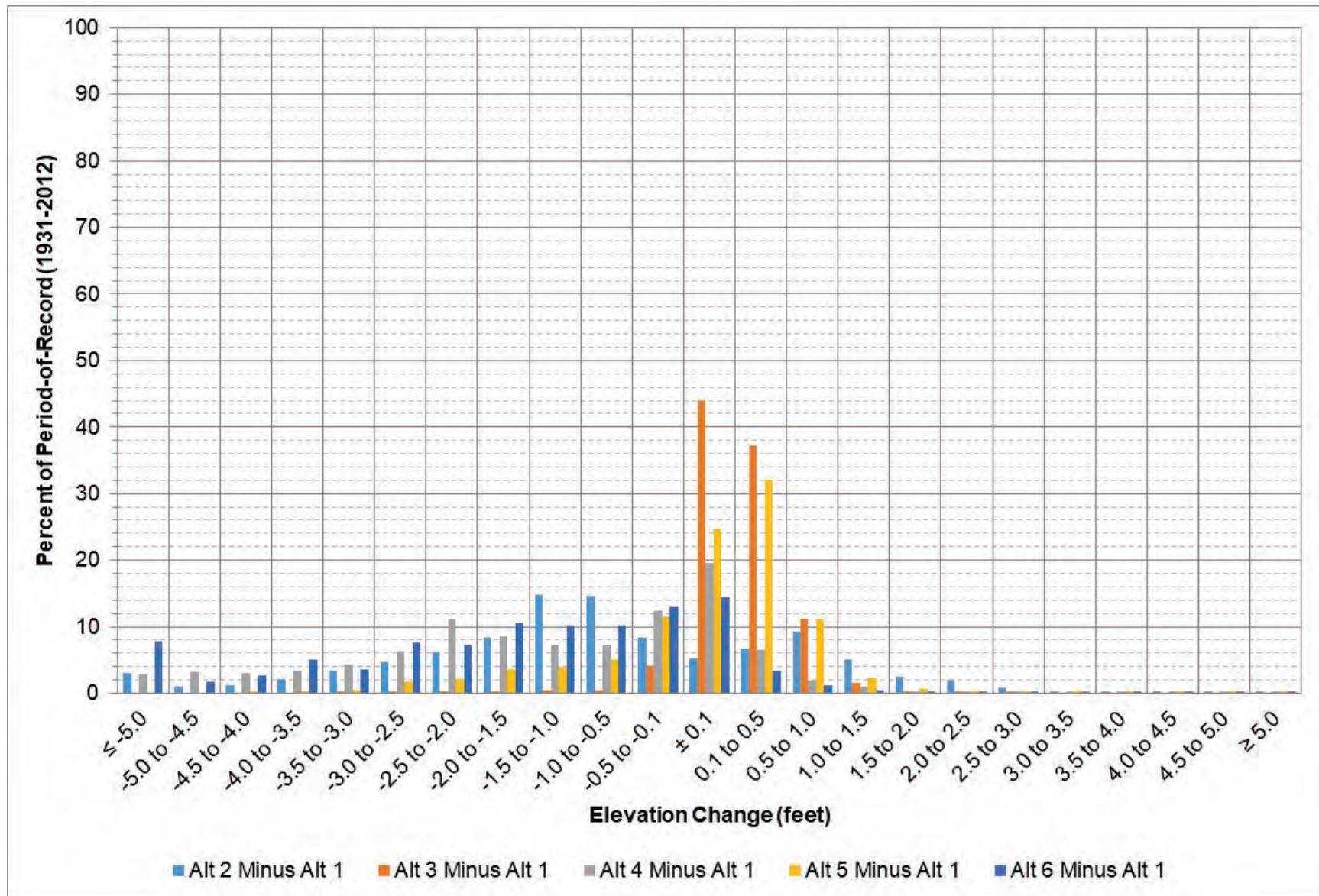
Figure 6-5: Oahe elevation change between each alternative and Alt 1 for all days in the period-of-record.
