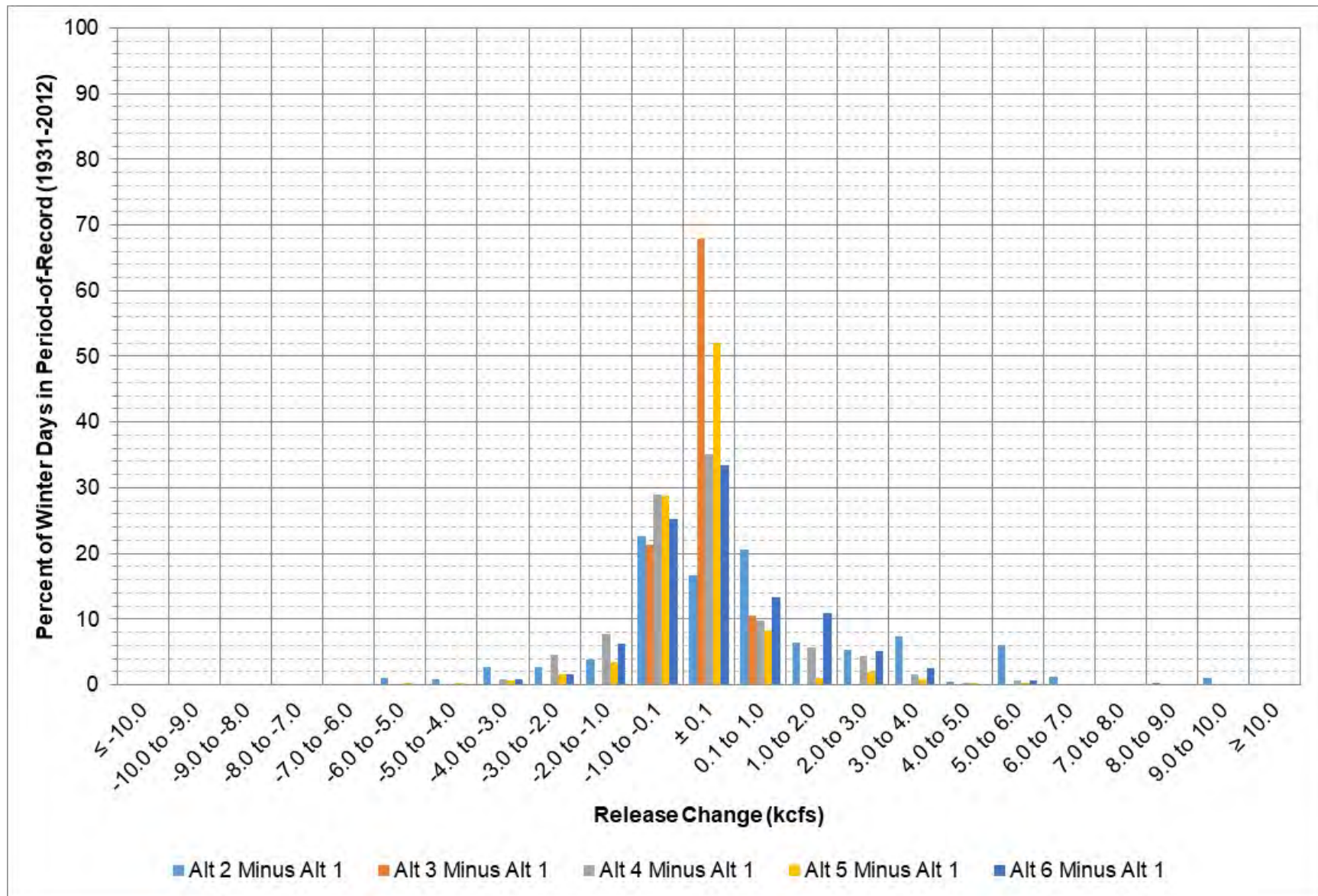
Figure 9-40: Garrison release change between each alternative and Alt 1 during December – February.
