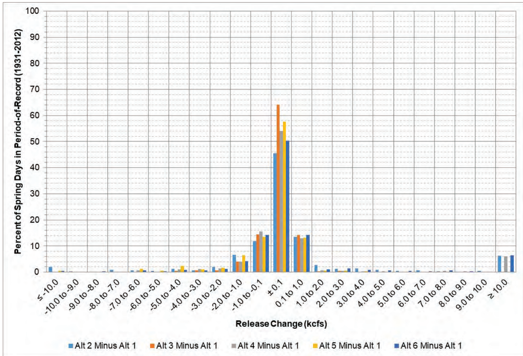
Figure 2-24: Big Bend release change between each alternative and Alt 1 during March – April.
