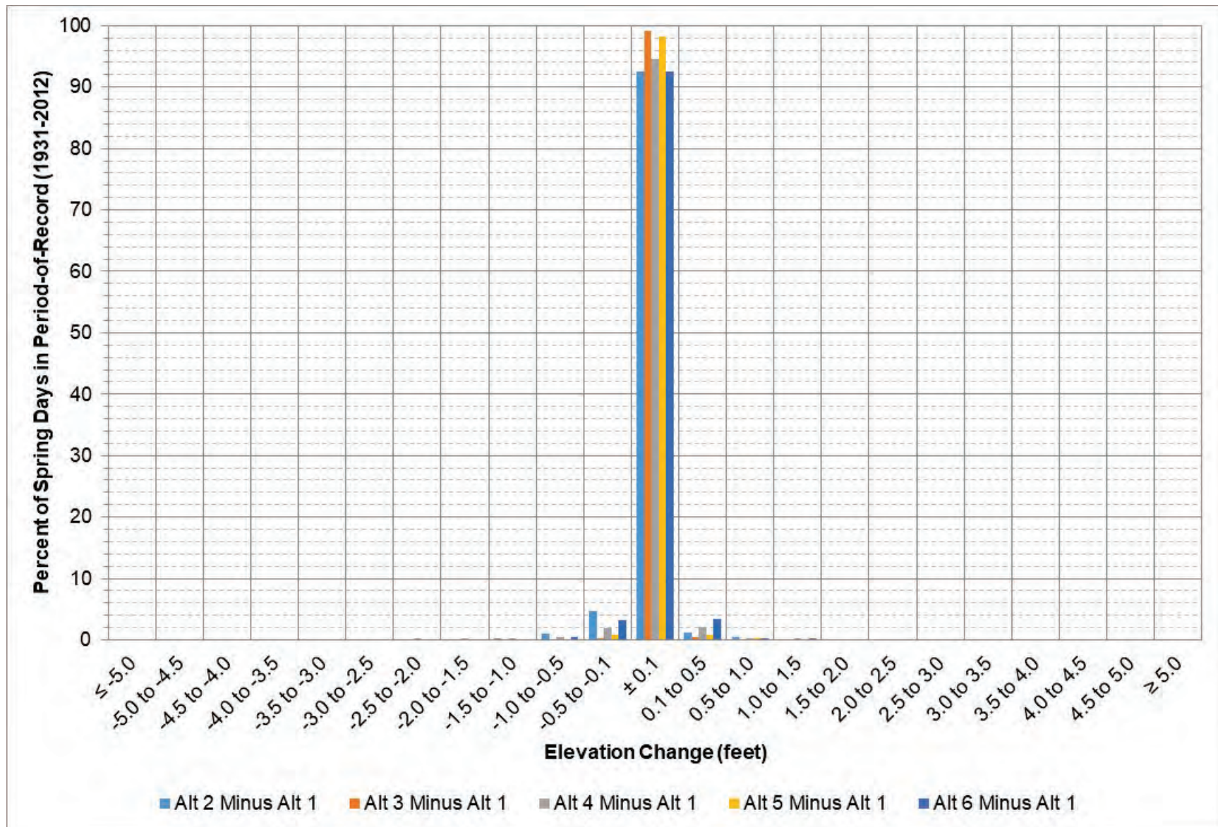
Figure 2-23: Big Bend elevation change between each alternative and Alt 1 during March – April.
