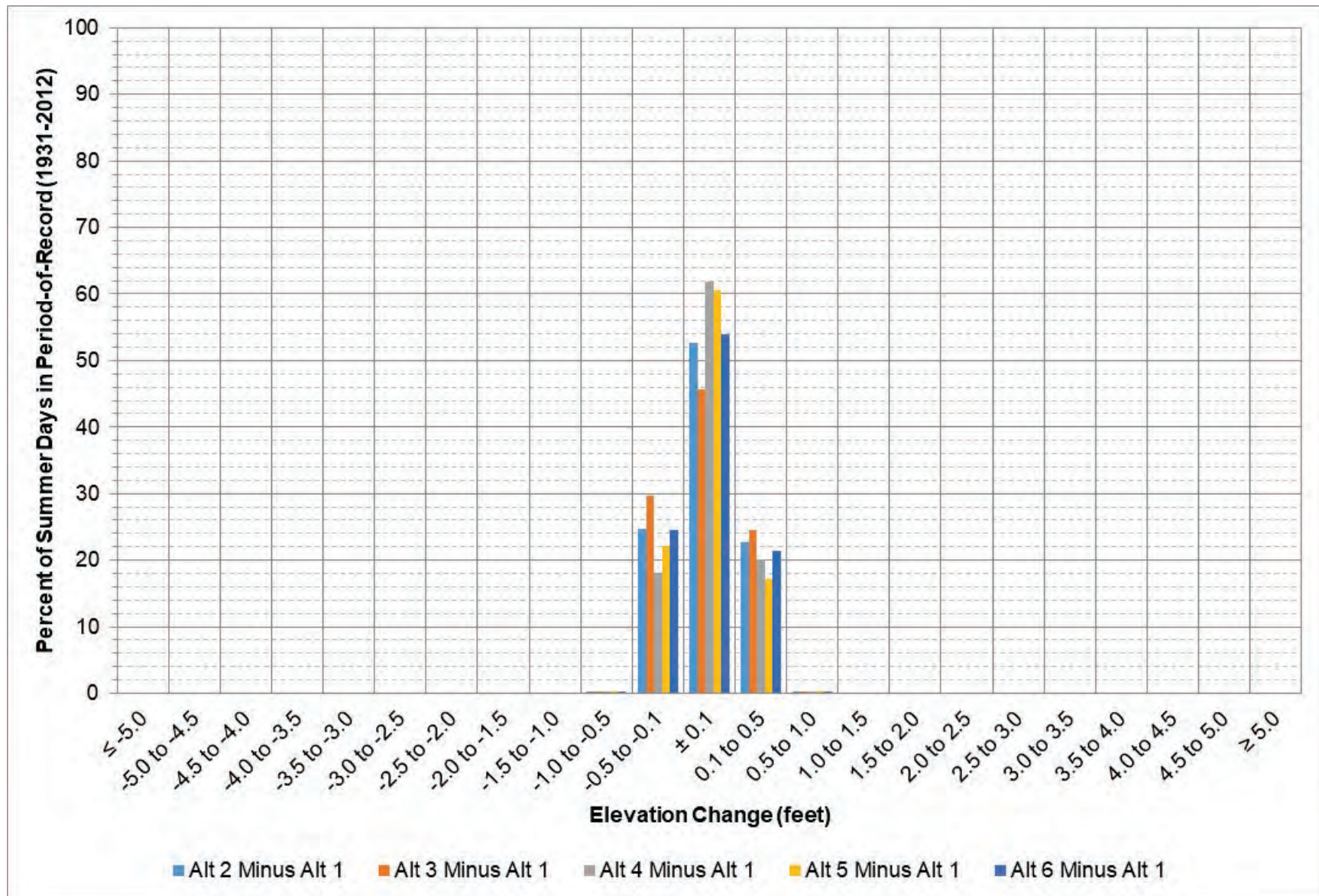
Figure 3-20: Big Bend elevation change between each alternative and Alt 1 during May – August.
