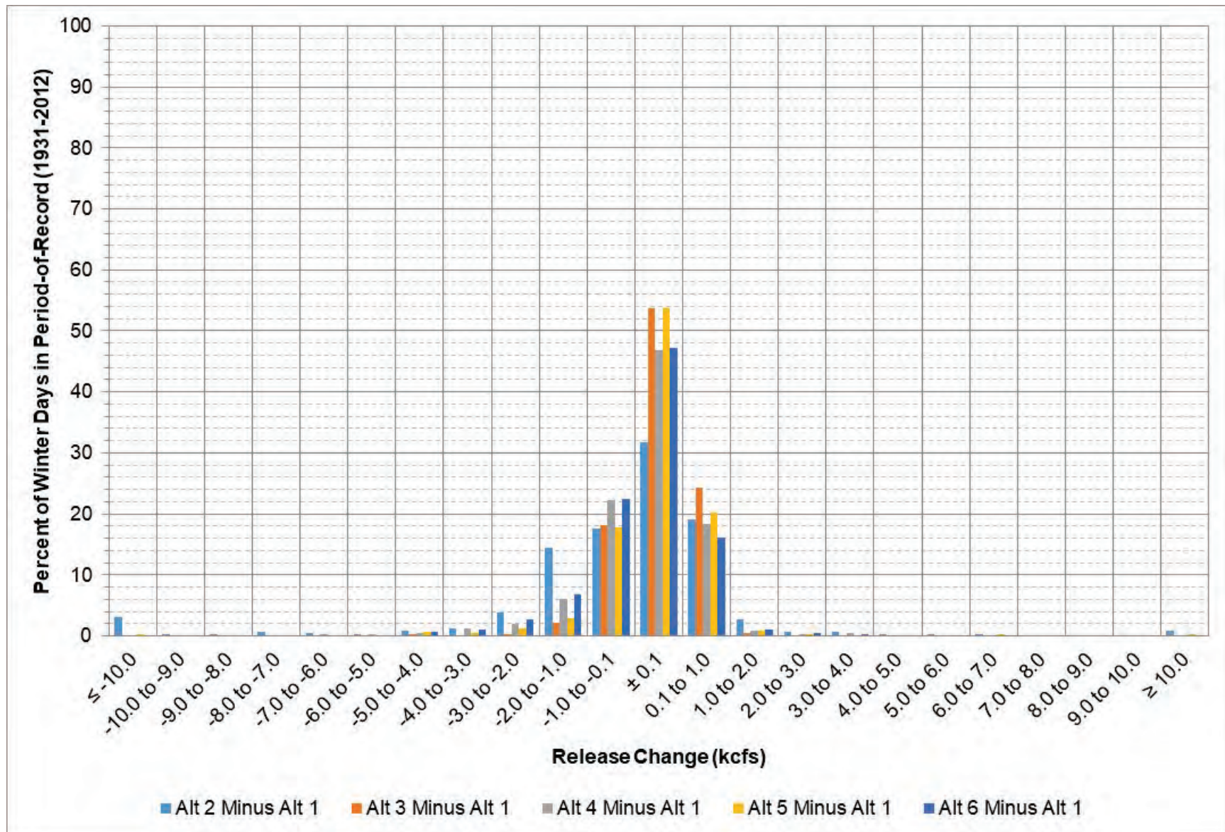
Figure 5-13: Big Bend release change between each alternative and Alt 1 during December – February.
