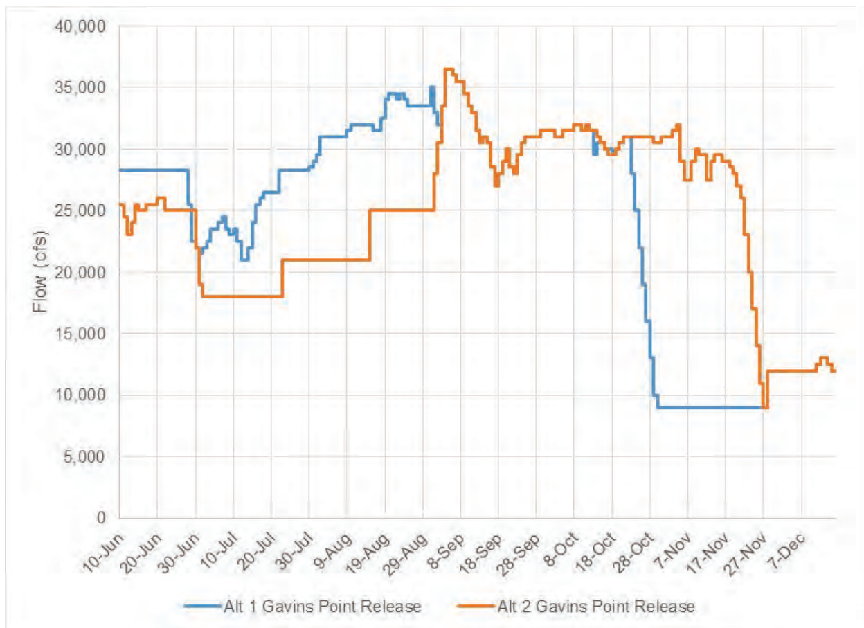
Figure 3-6: Alt 1 Gavins Point releases vs Alt 2's Gavins Point releases for low summer flow operations.
