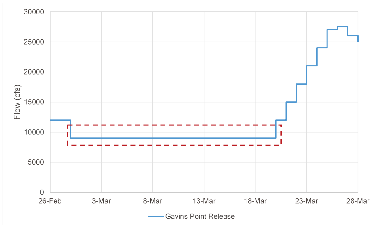
Figure 2-1: Spring water supply release from Gavins Point.
