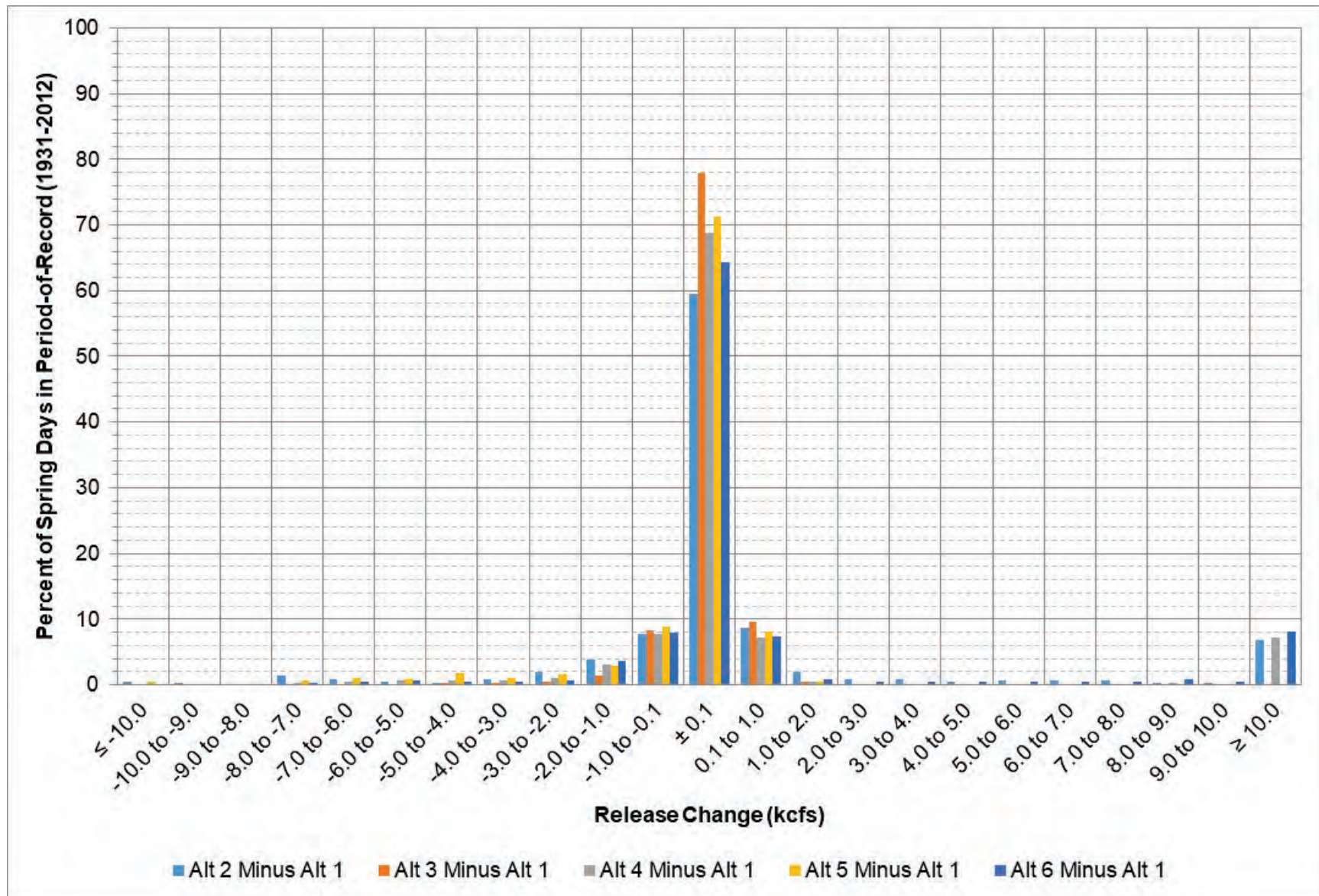
Figure 2-26: Fort Randall release change between each alternative and Alt 1 during March – April.
