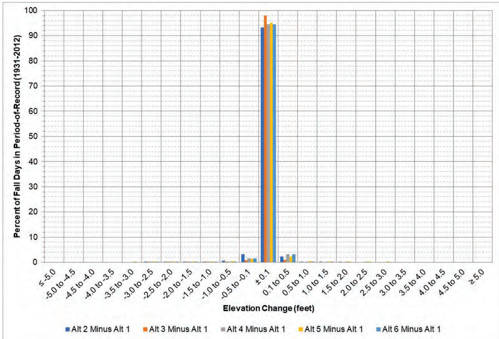
Figure 4-16: Big Bend elevation change between each alternative and Alt 1 during September – November.
