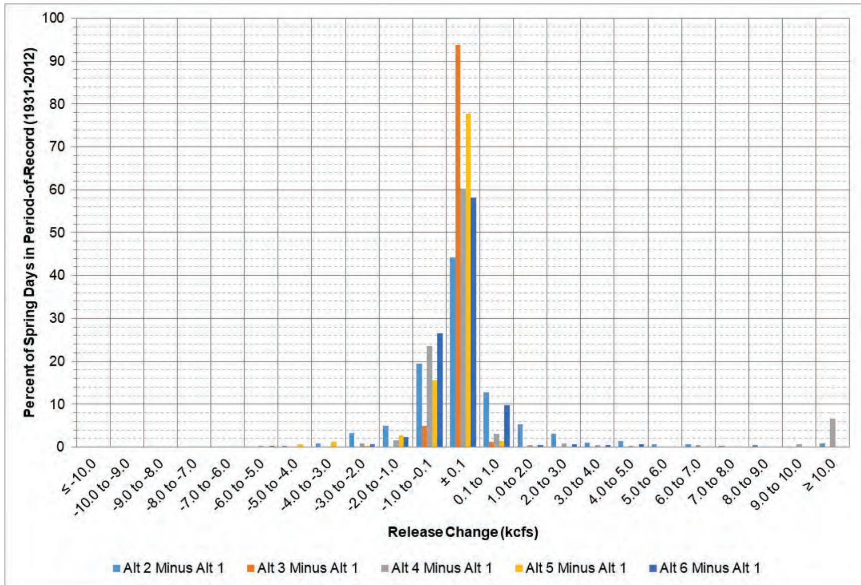
Figure 2-20: Garrison release change between each alternative and Alt 1 during March – April.
