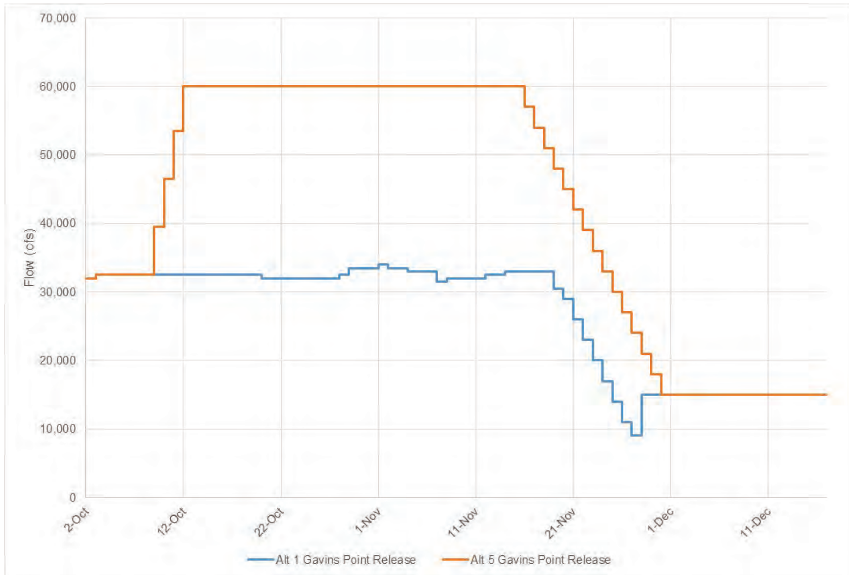
Figure 4-4: Comparison of Alt 1 vs Alt 5 Gavins Point releases during the ESH-creating release shown in Figure 4-3.
