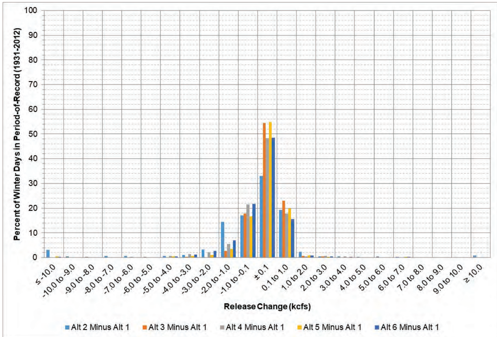
Figure 5-11: Oahe release change between each alternative and Alt 1 during December – February.
