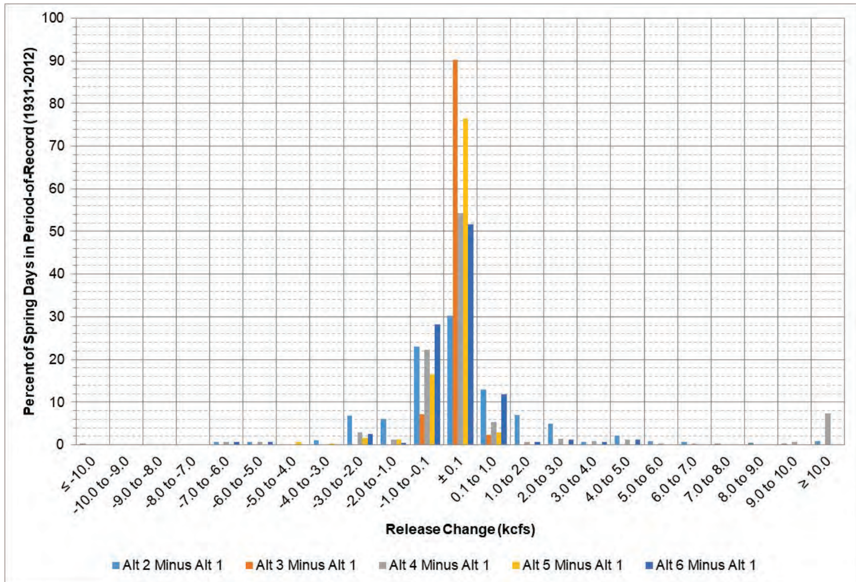
Figure 9-4: Garrison release change between each alternative and Alt 1 during March – April.
