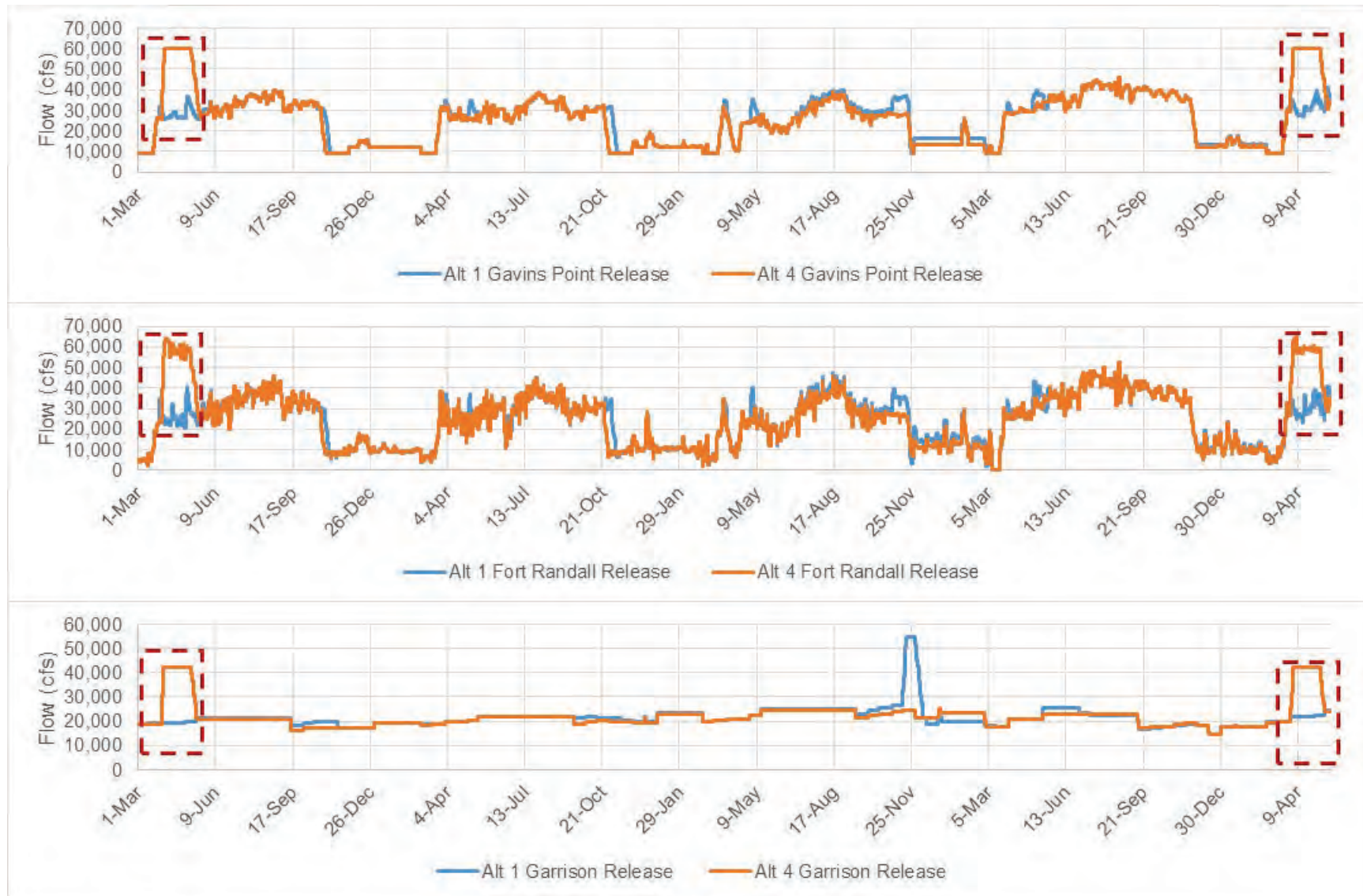
Figure 2-15: Comparison of Alt 1 vs Alt 4 Gavins Point, Fort Randall, and Garrison releases during same five year period with ESH-creating release operations as shown in Figure 2-8.
