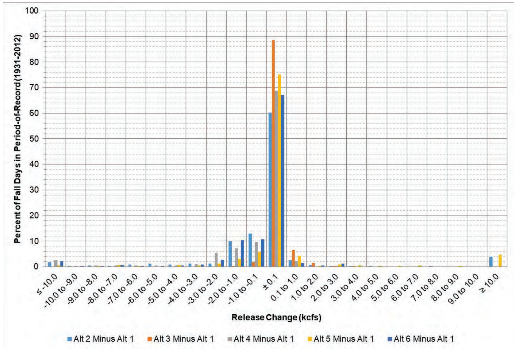
Figure 4-6: Gavins Point release change between each alternative and Alt 1 during September – November.
