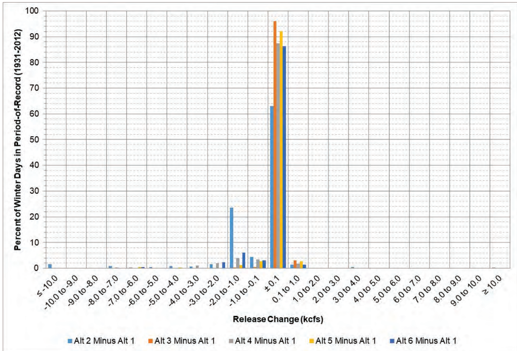
Figure 5-5: Gavins Point release change between each alternative and Alt 1 during December – February.
