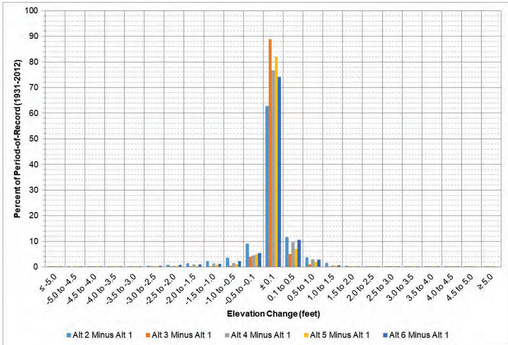
Figure 6-9: Fort Randall elevation change between each alternative and Alt 1 for all days in the period-of-record.
