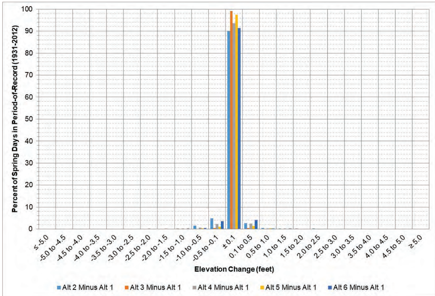
Figure 9-7: Big Bend elevation change between each alternative and Alt 1 during March – April.
