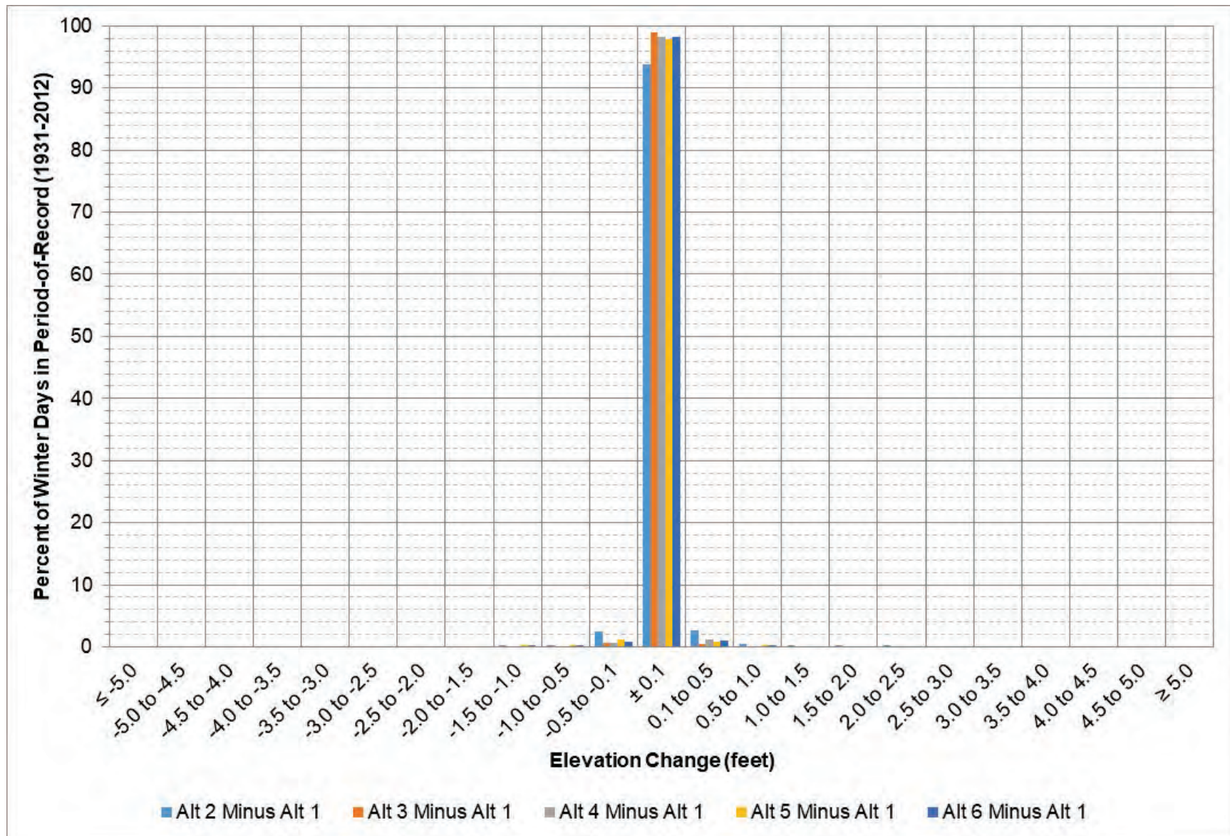
Figure 5-12: Big Bend elevation change between each alternative and Alt 1 during December – February.
