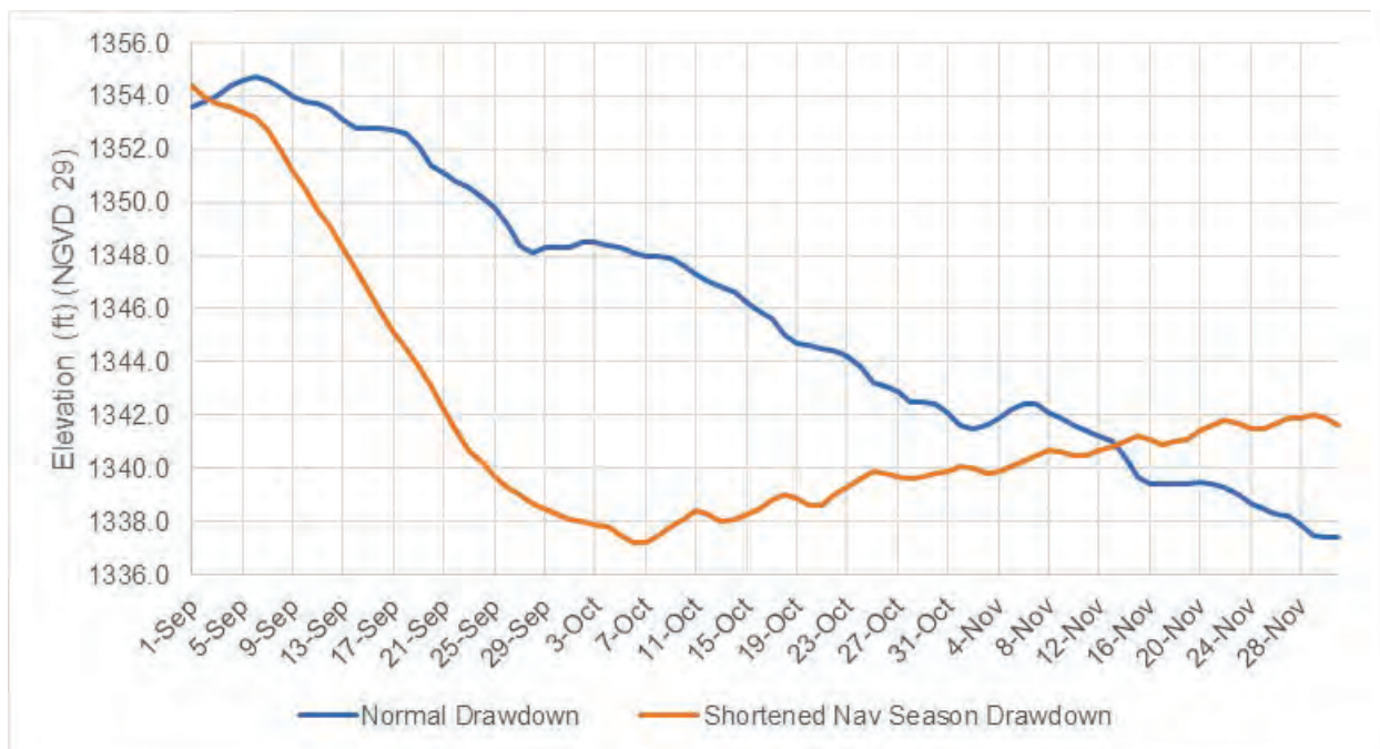
Figure 4-7: Fort Randall fall drawdown.
