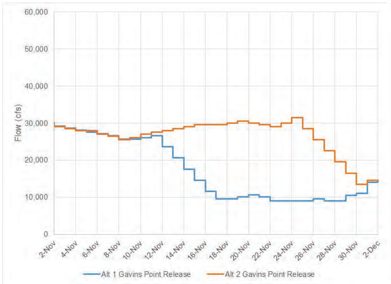
Figure 4-2: Alt 1 Gavins Point releases vs Alt 2's Gavins Point releases for end-of-the-season navigation operations.
