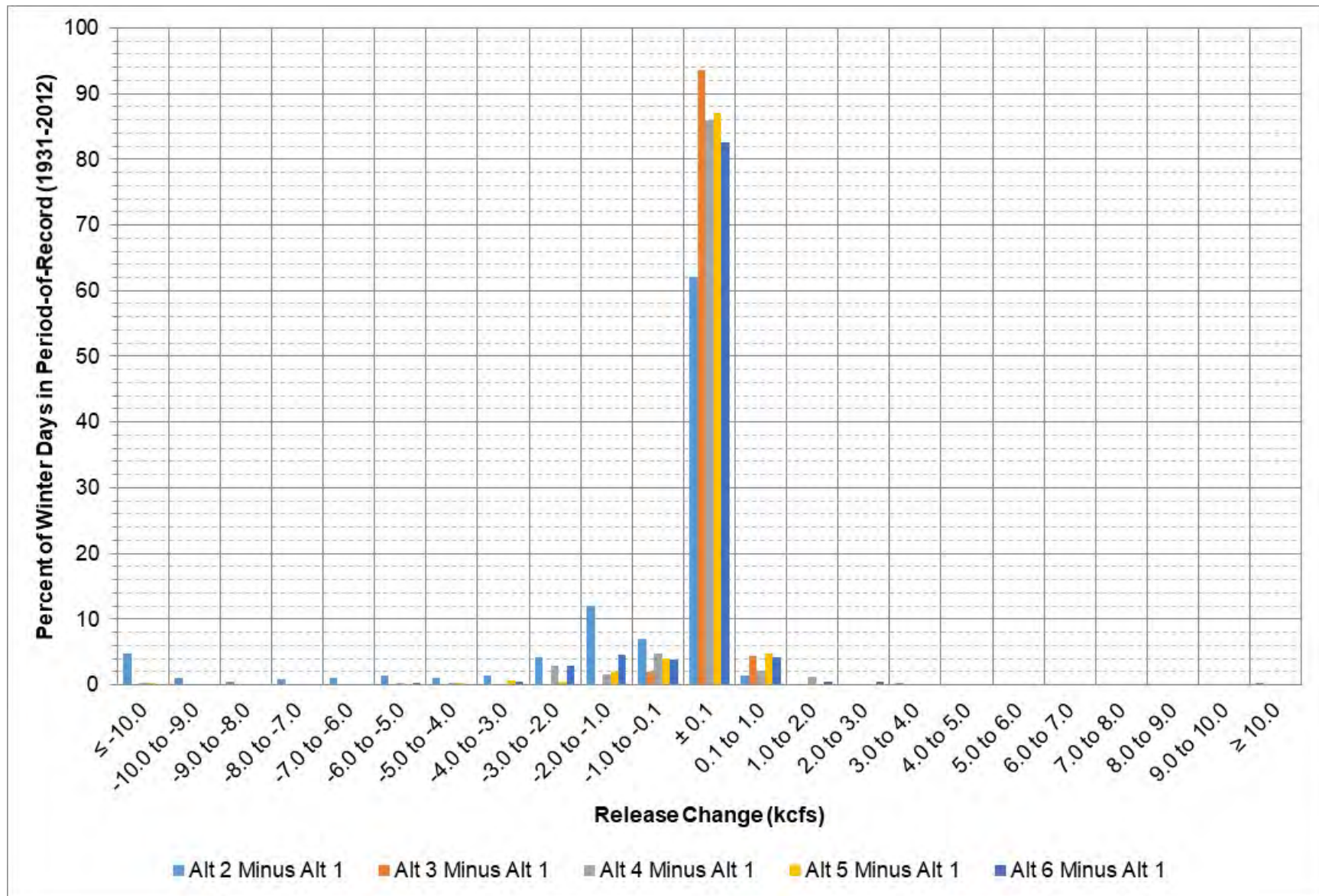
Figure 9-48: Gavins Point release change between each alternative and Alt 1 during December – February.
