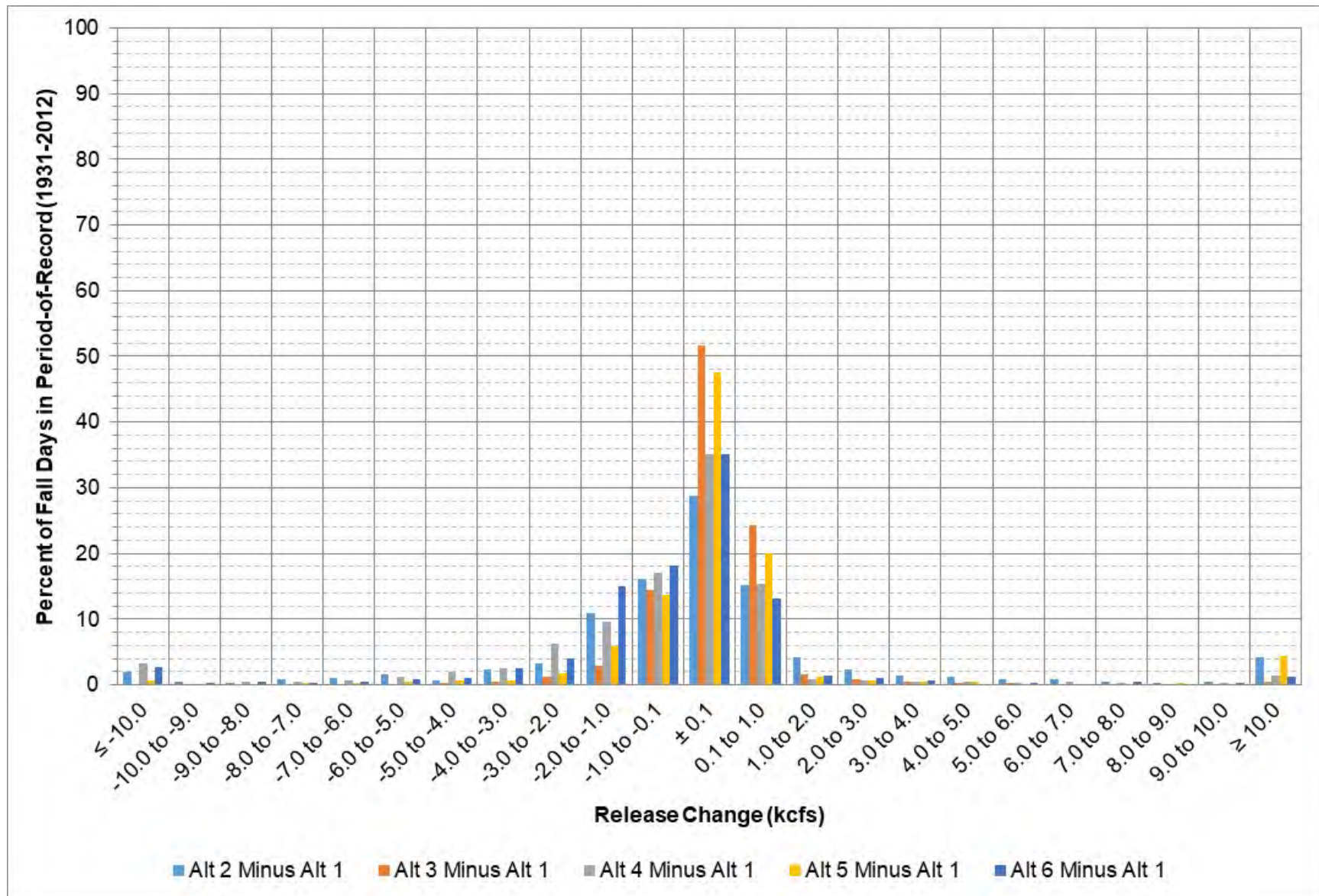
Figure 9-32: Big Bend release change between each alternative and Alt 1 during September – November.
