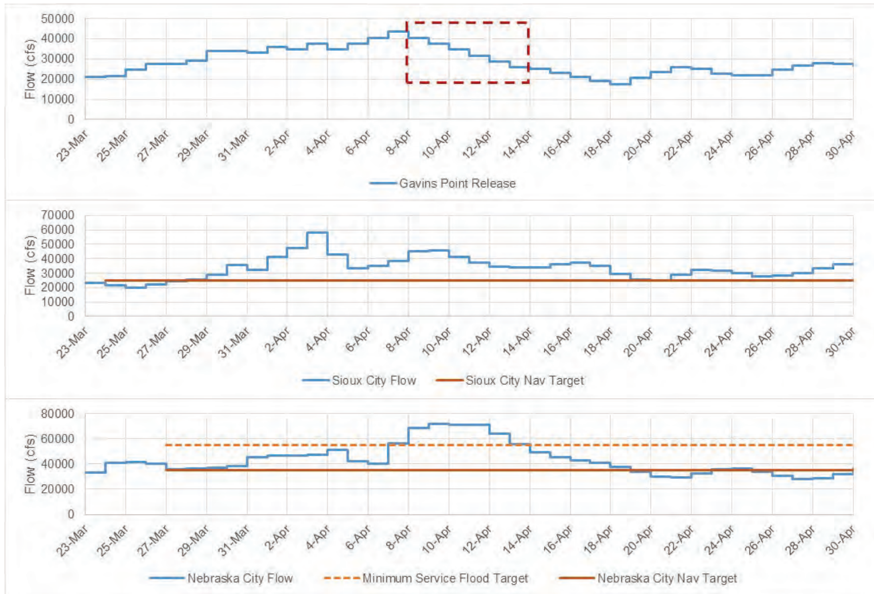
Figure 2-5: Example of reducing Gavins Point due to exceeding flood targets at Nebraska City.
