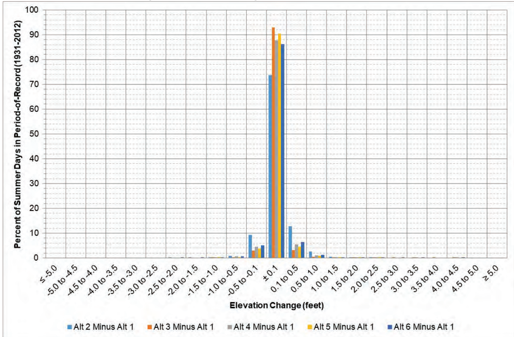
Figure 3-10: Gavins Point elevation change between each alternative and Alt 1 during May – August.
