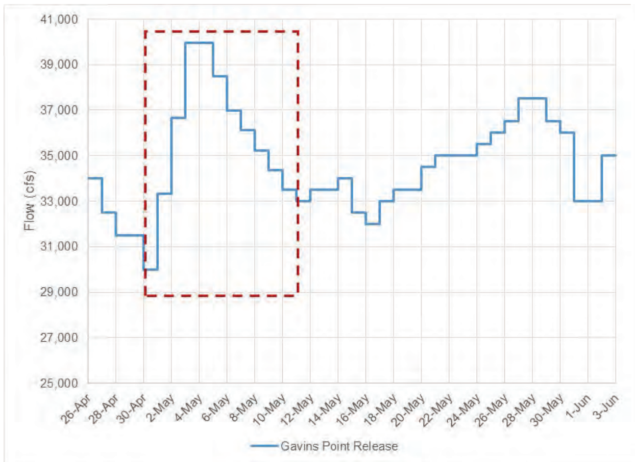
Figure 3-1: Late spring spawning cue for Alt 1.
