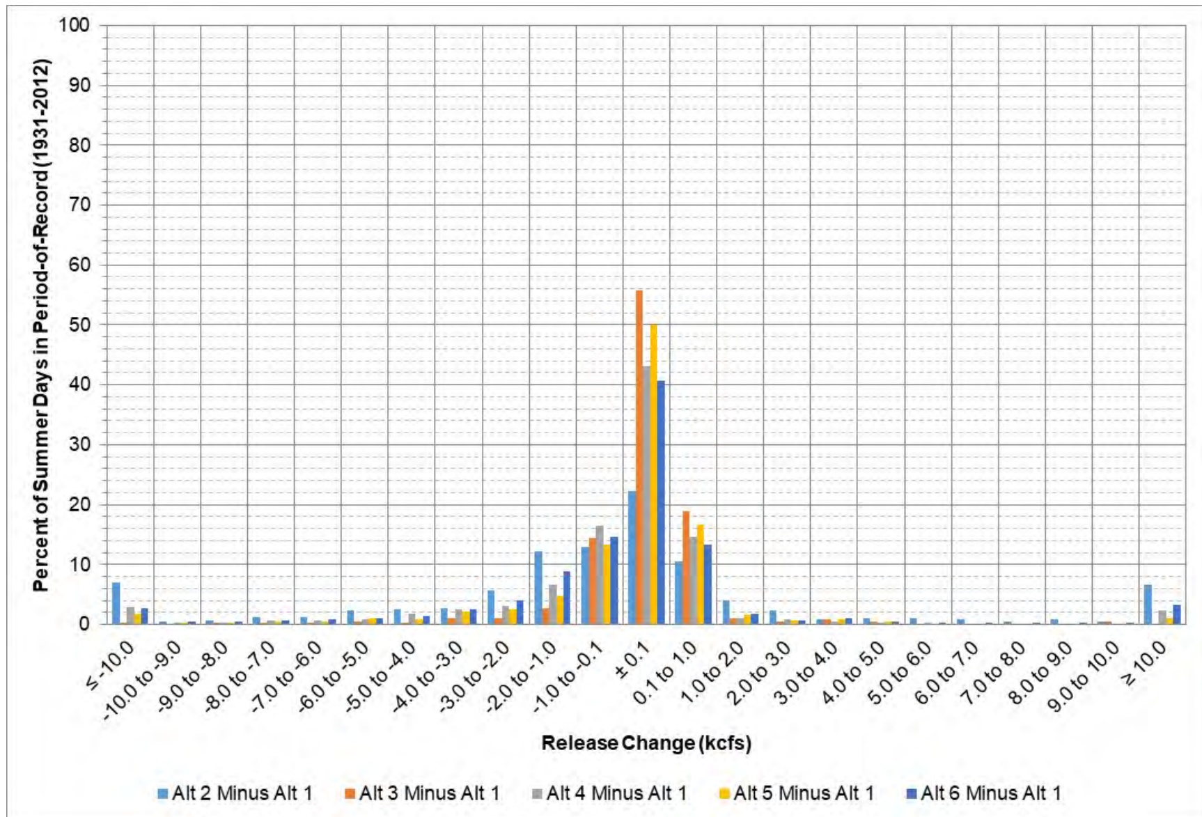
Figure 9-20: Big Bend release change between each alternative and Alt 1 during May – August.
