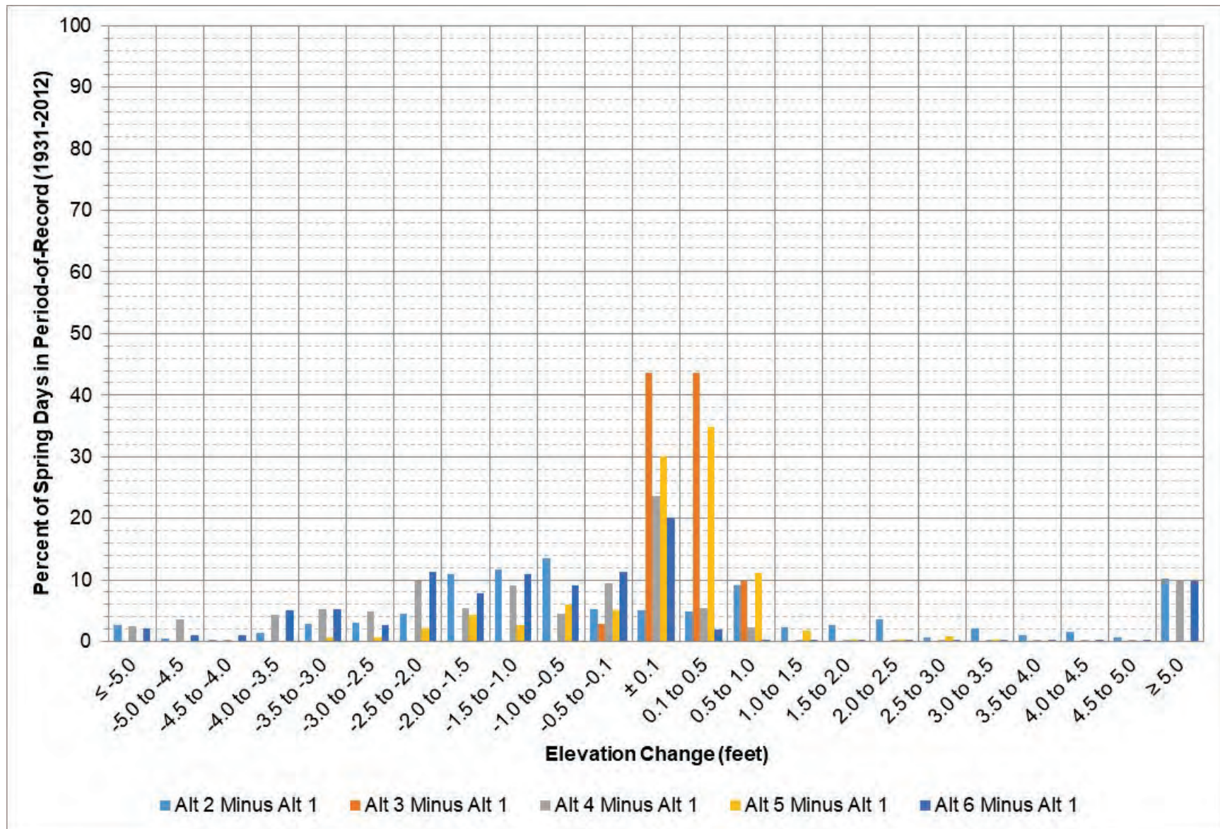
Figure 9-5: Oahe elevation change between each alternative and Alt 1 during March – April.
