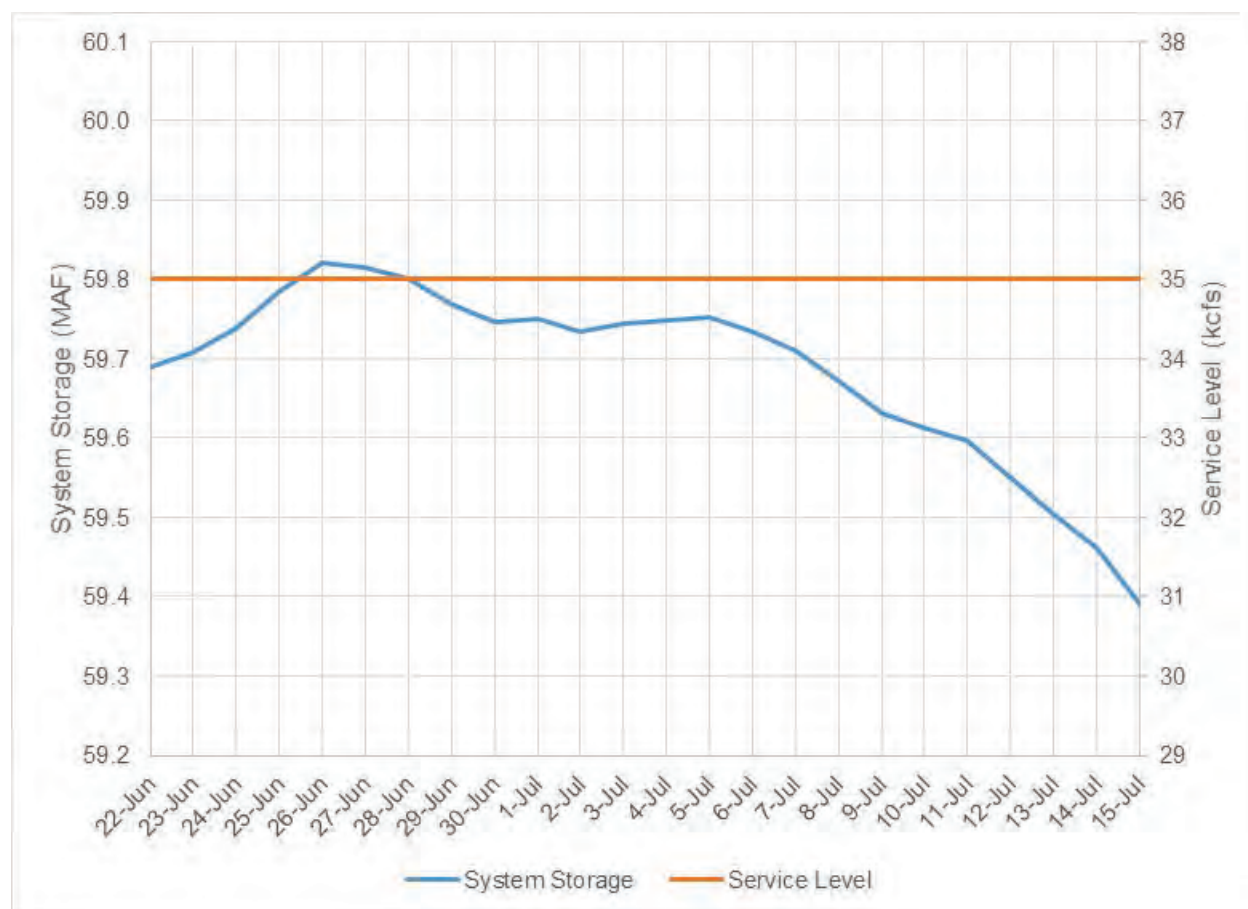
Figure 3-3: July 1 System storage assessment and resulting service level.
