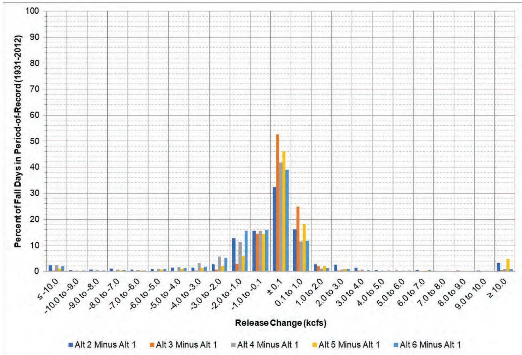
Figure 4-15: Oahe release change between each alternative and Alt 1 during September – November.
