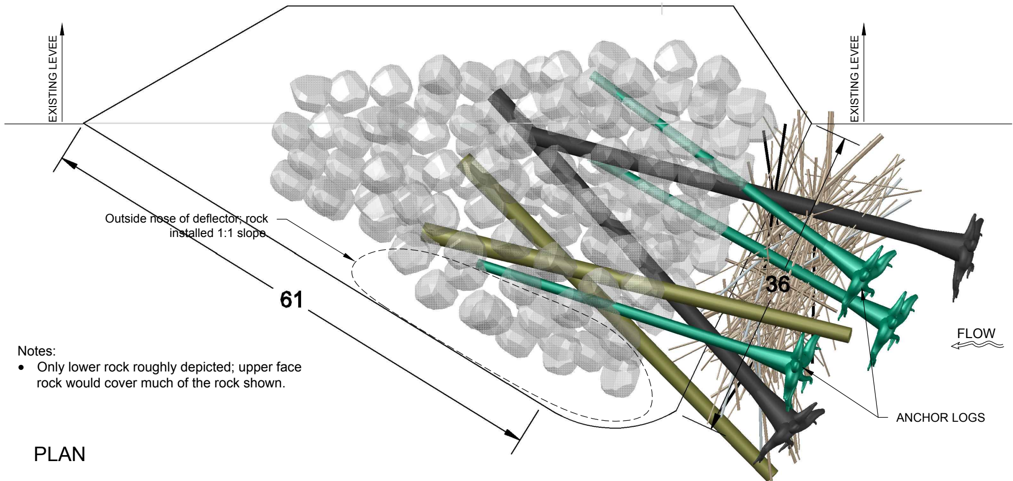
Wood Augmentation of Sunshine Point Deflector Structures - Option 1 LW with Rootwad/Racking
