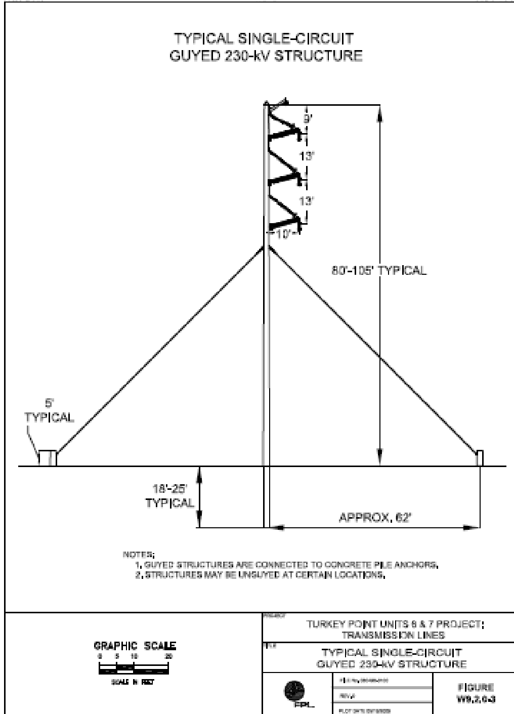
Figure 2B. Conceptual drawing of the 230-kV transmission power line structure within the West Preferred Corridor.
