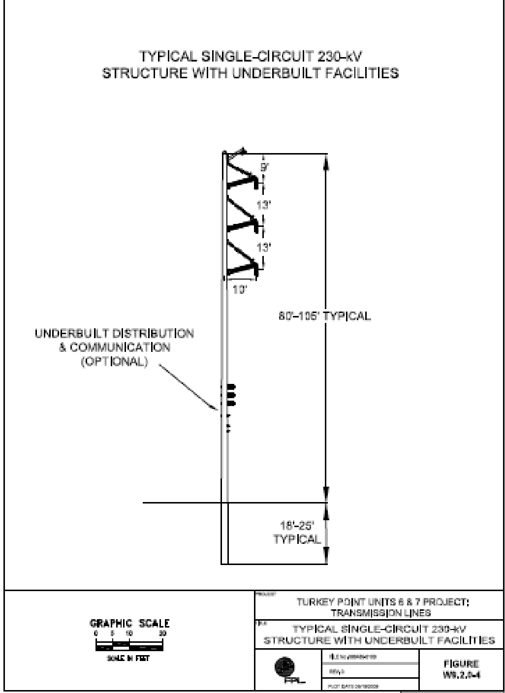
Figure 2C. Conceptual drawing of the 230-kV transmission power line structure within the West Preferred Corridor.
