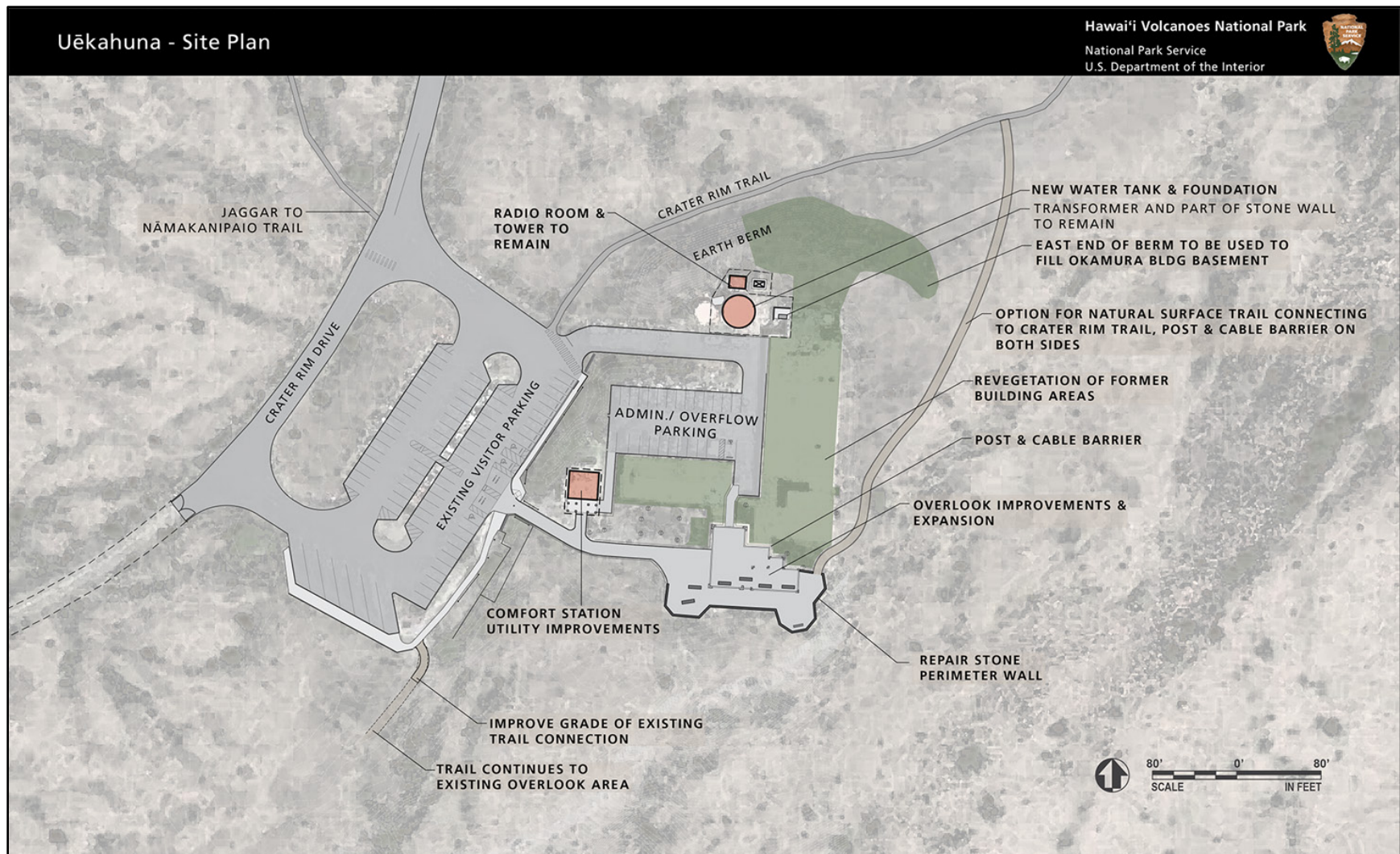
Figure 2. Proposed Action – Uēkahuna Site Plan
