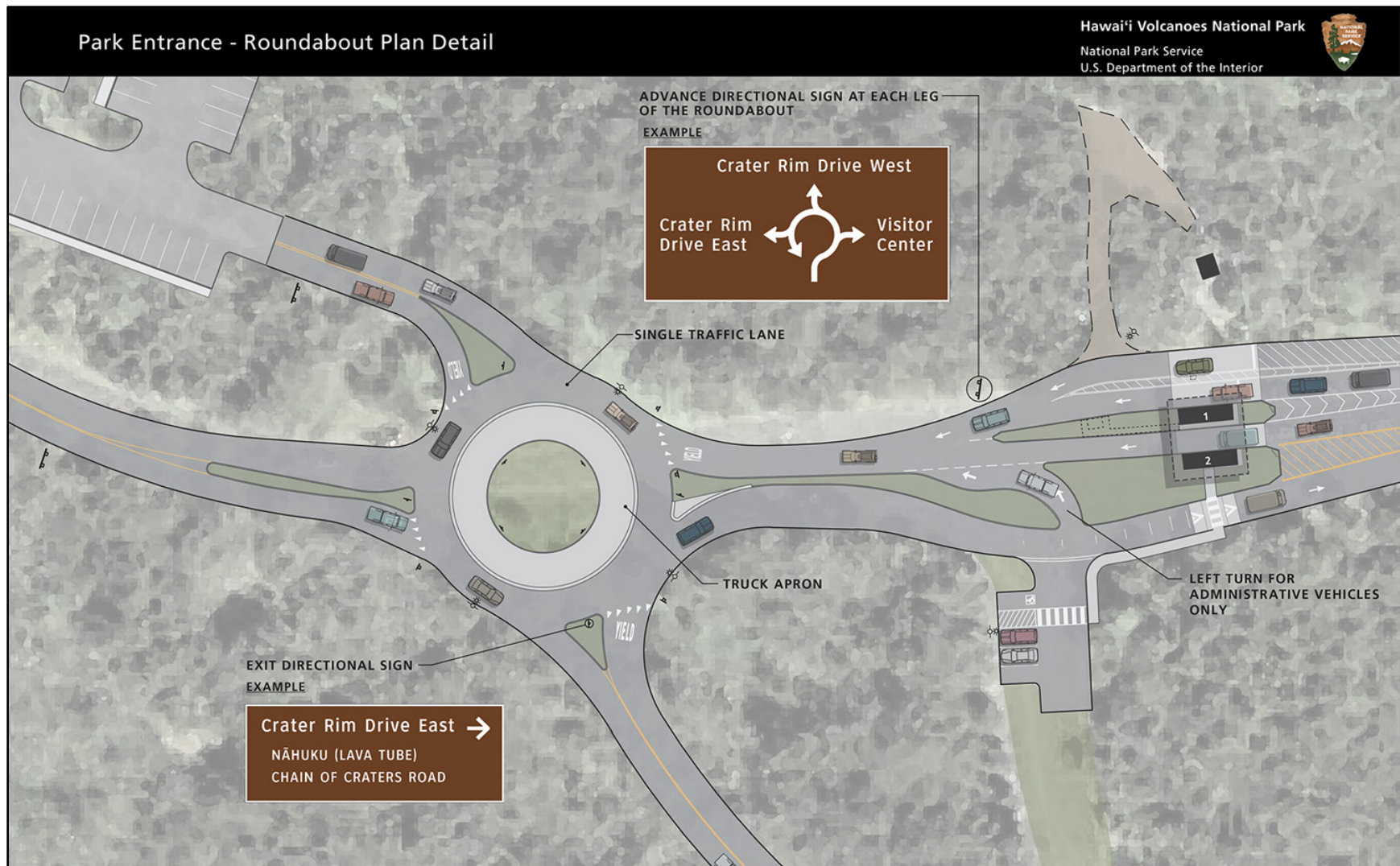
Figure 6. Proposed Action – Park Entrance Roundabout Plan Detail
