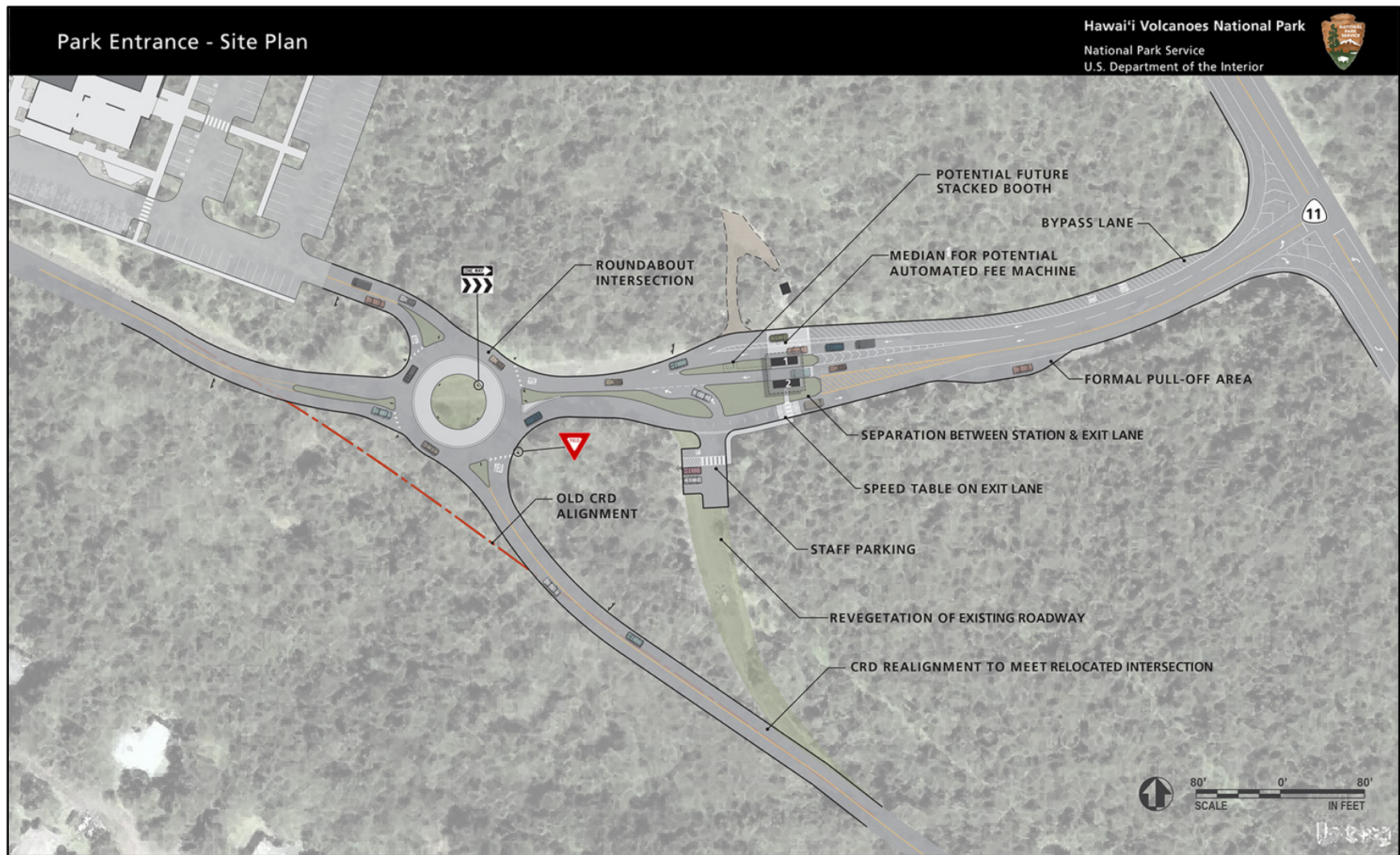
Figure 5. Park Entrance Site Plan
