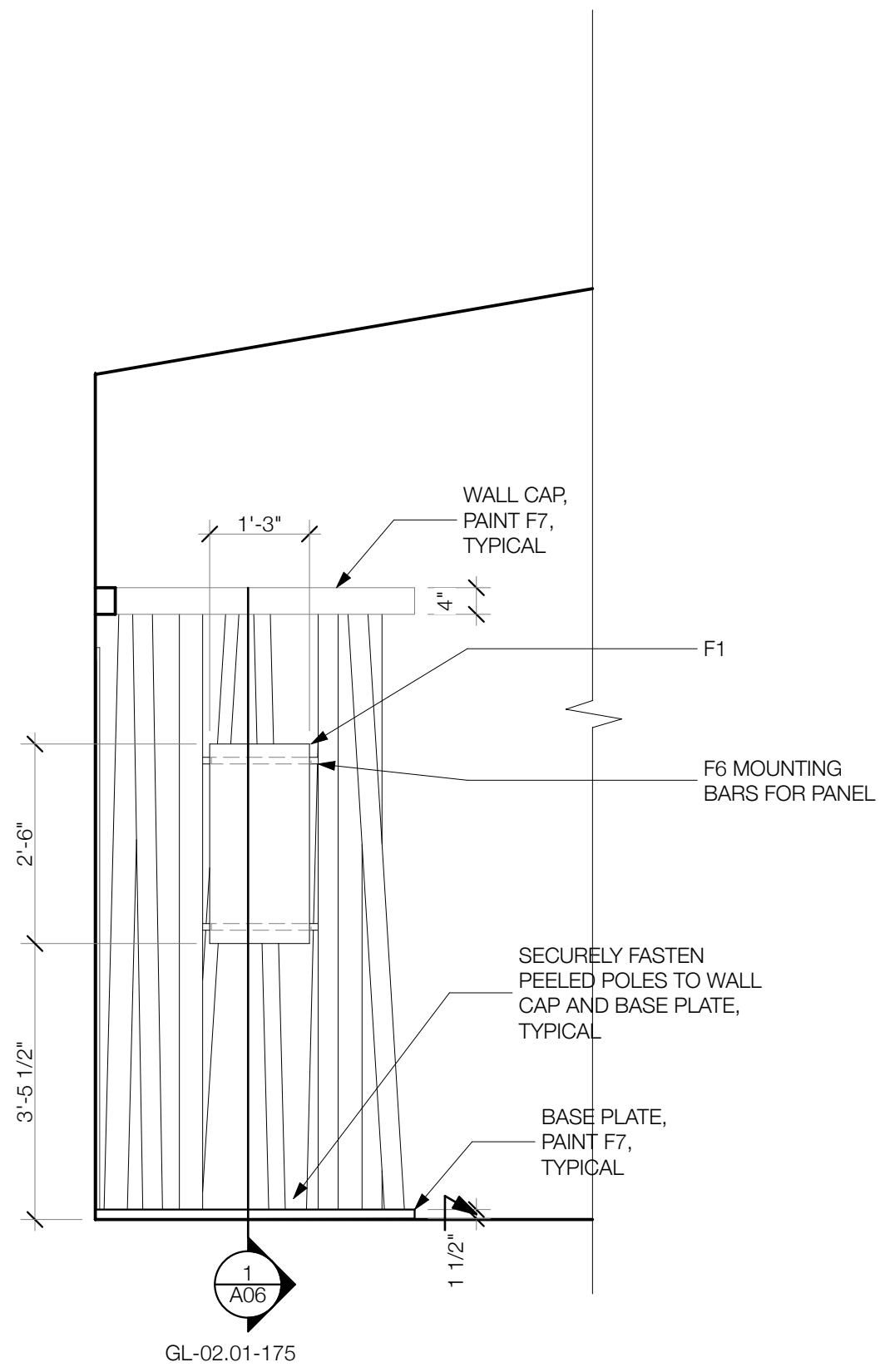
MEDICINE WHEEL PANEL ELEVATION
