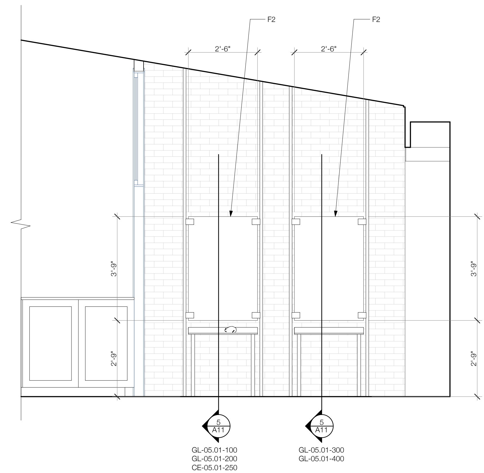
PANELS ELEVATION SCALE: 1/2" = 1'-0"
