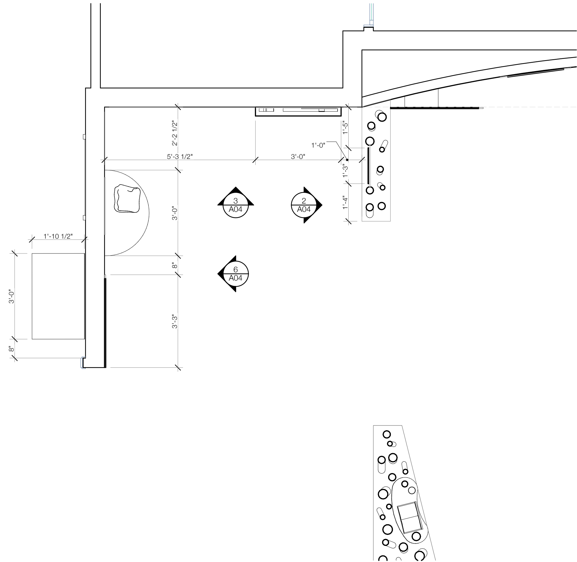
SCENE 01 INTRODUCTION PLAN
