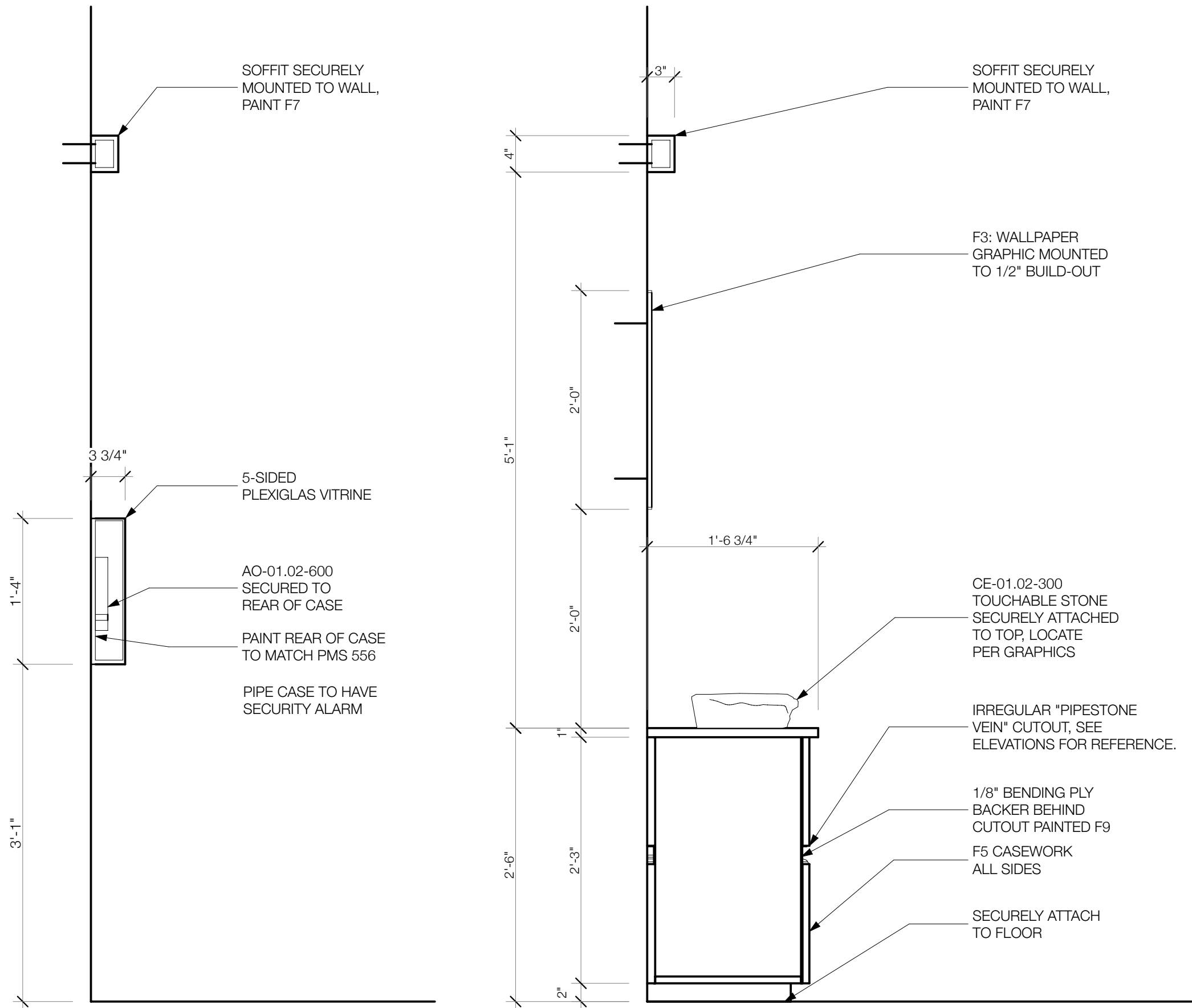
PIPE CASE SECTION
