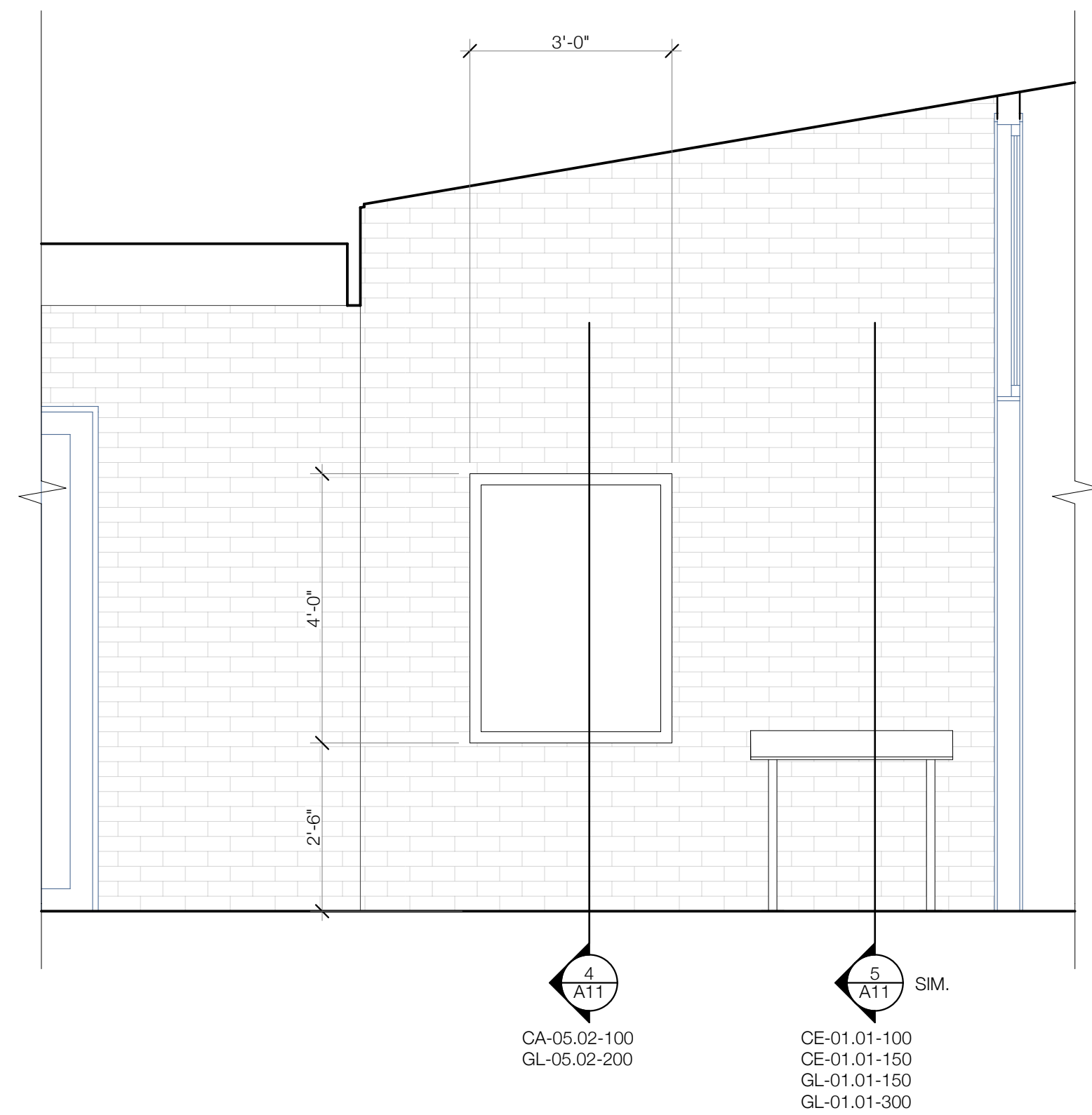
CHANGING CONTENT BOARD & TACTILE FLOOR PLAN ELEVATION SCALE: 1/2" = 1'-0"
