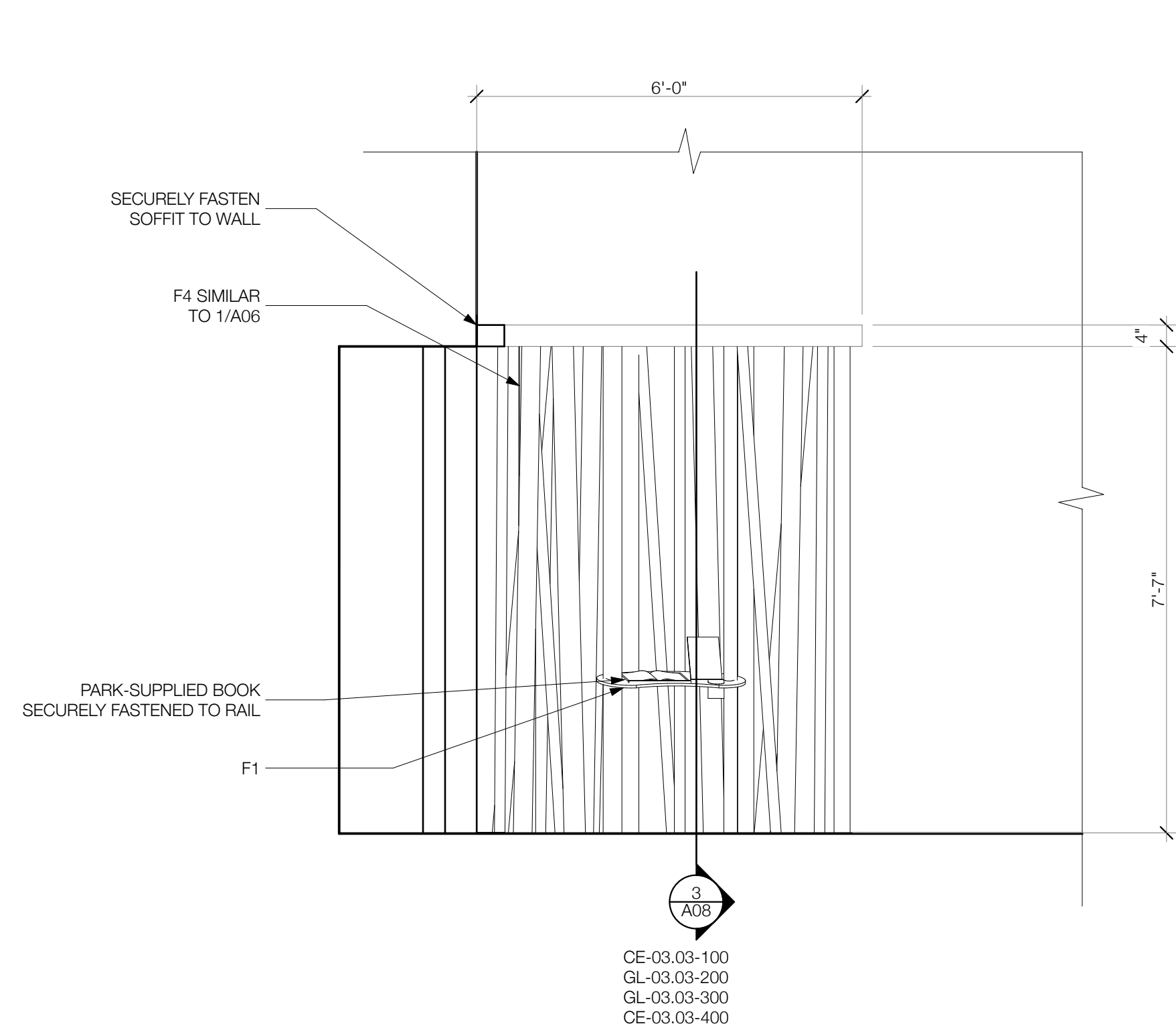
RESPONSE STATION ELEVATION SCALE: 1/2" = 1'-0"
