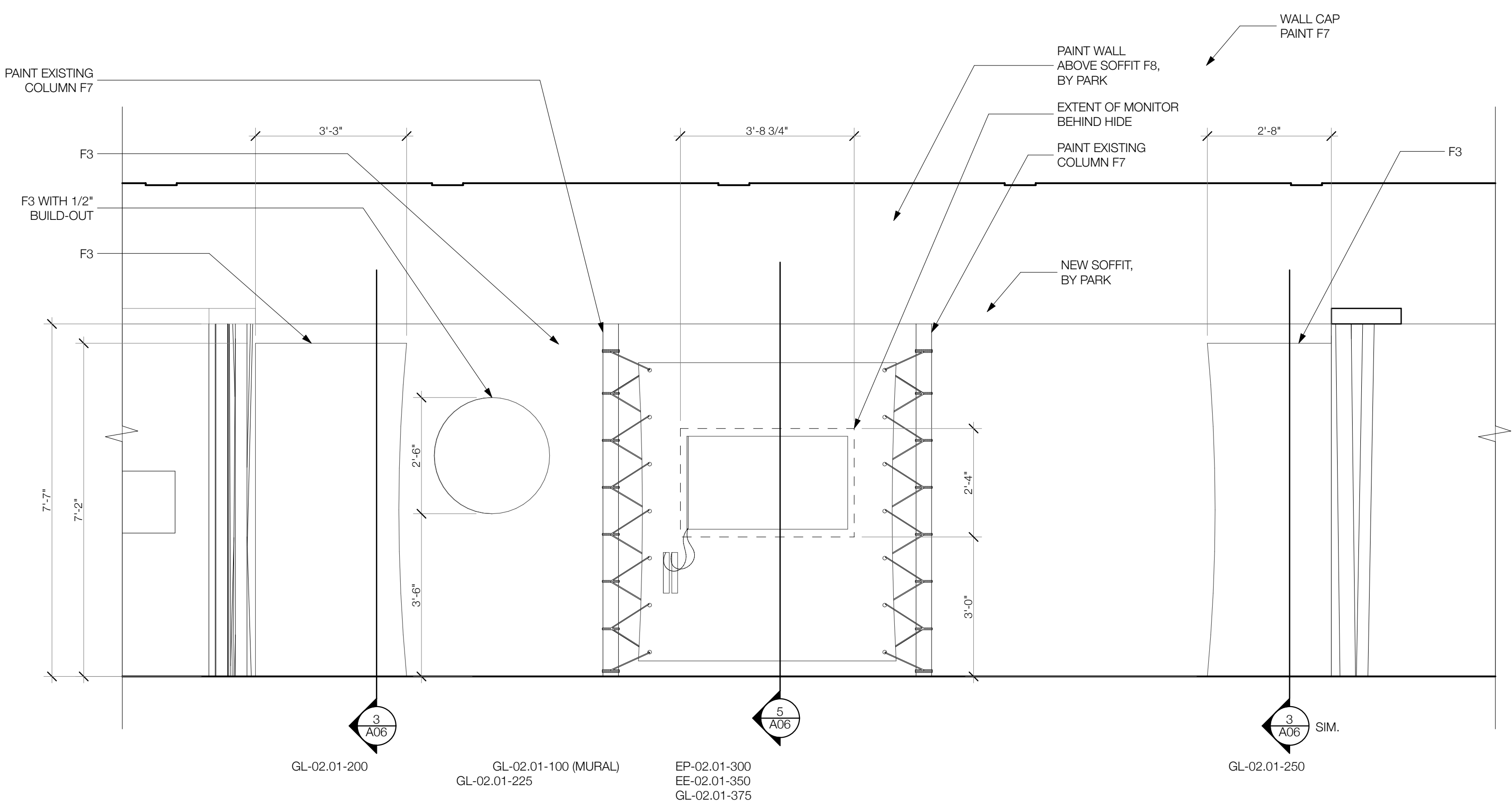
PRAIRIE ELEVATION
