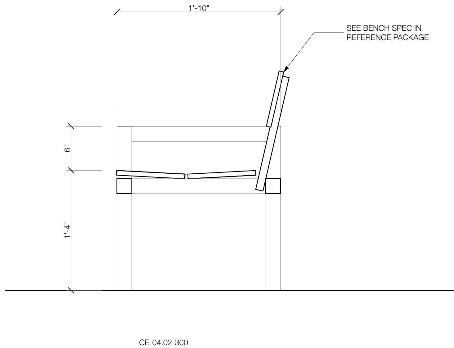
THEATER BENCH SECTION SCALE: 1 1/2" = 1'-0" 2
