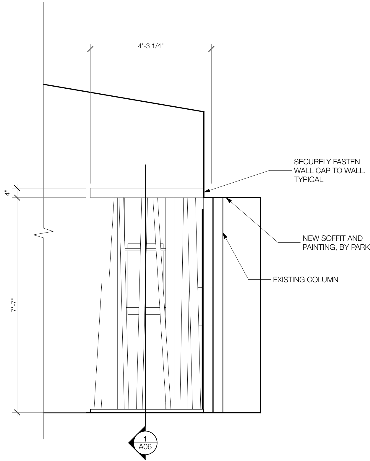
S02 PEELED POLE WALL ELEVATION
