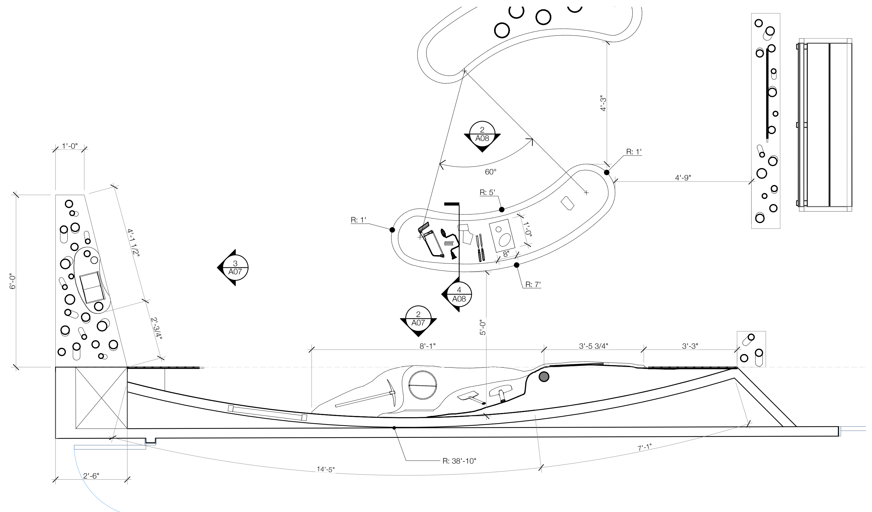
SCENE 03 QUARRYING AND CARVING PLAN
