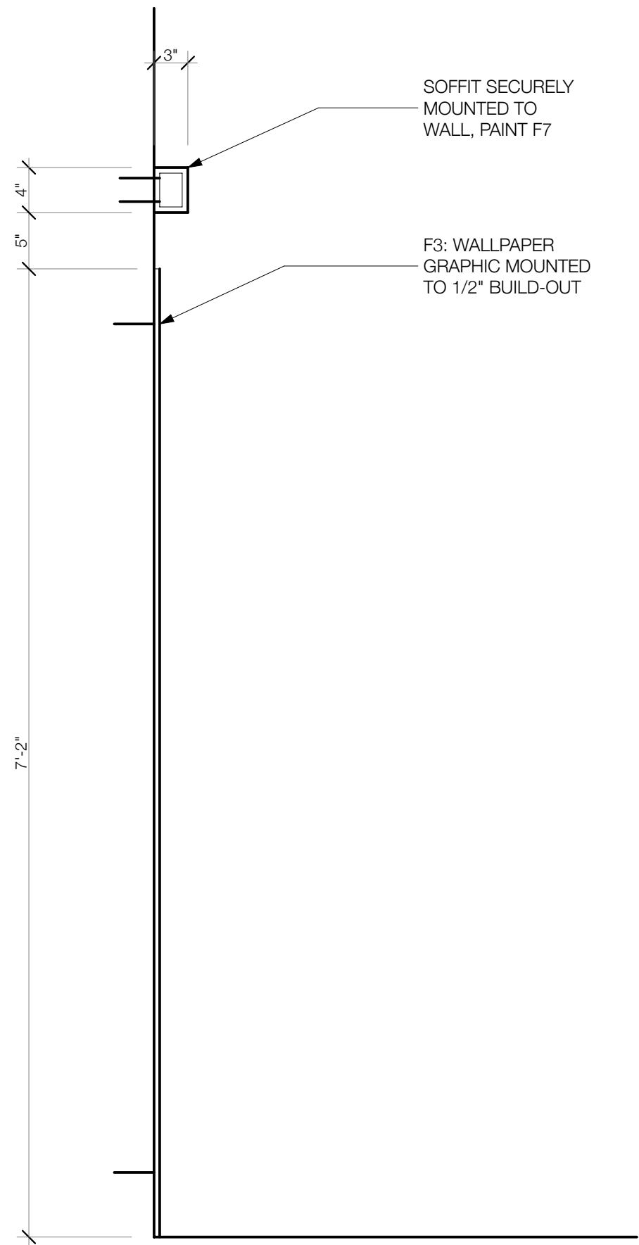
WALL-MOUNTED PANEL SECTION
