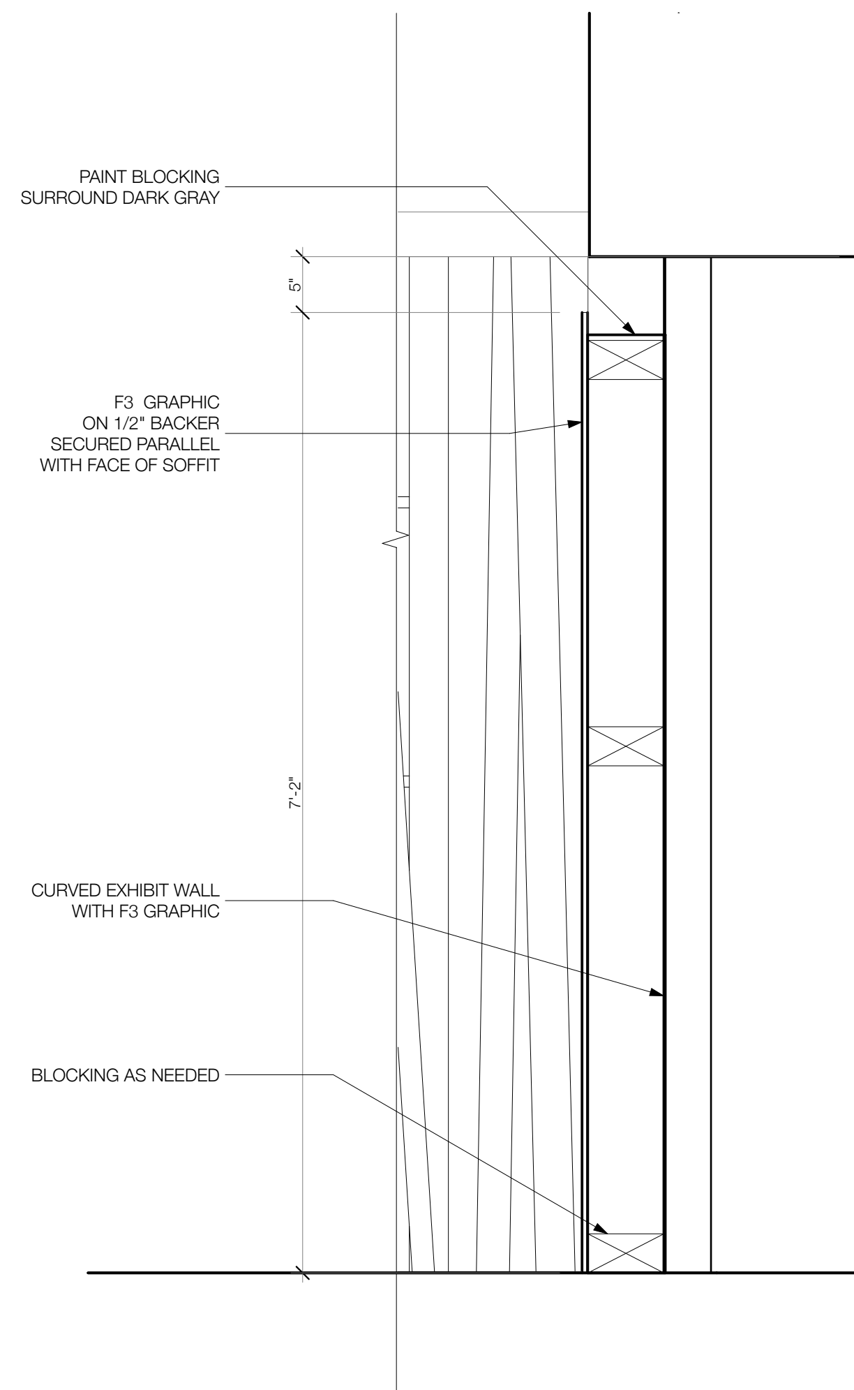
TOPIC PANEL SECTION SCALE: 1" = 1'-0"
