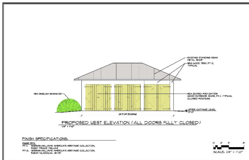
Front (west) façade: first proposal (top drawing); current/revised proposal showing doors in closed position (bottom drawing).
